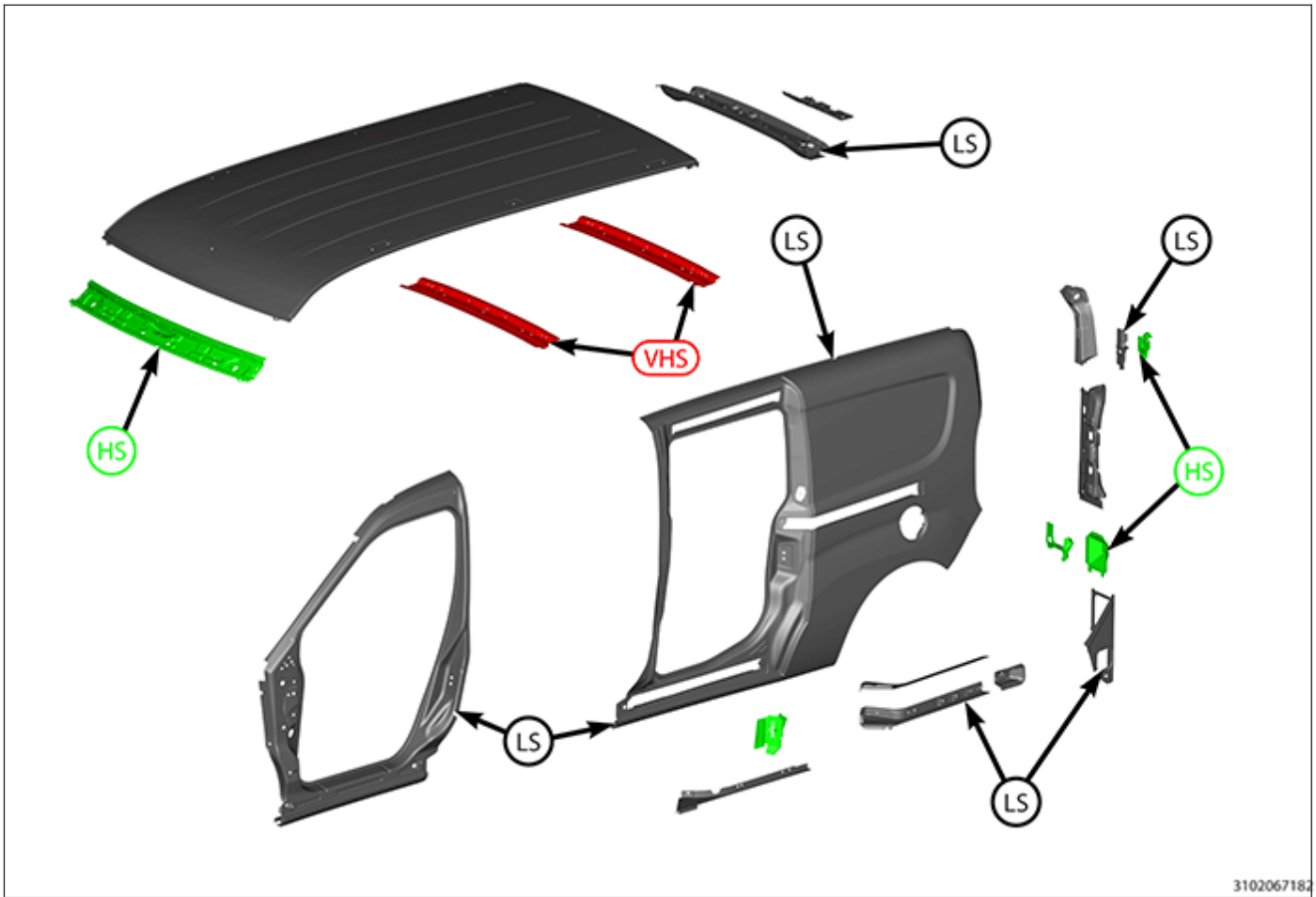
BODY IN WHITE COMPONENT IDENTIFICATION - ROOF AND SIDE PANELS
