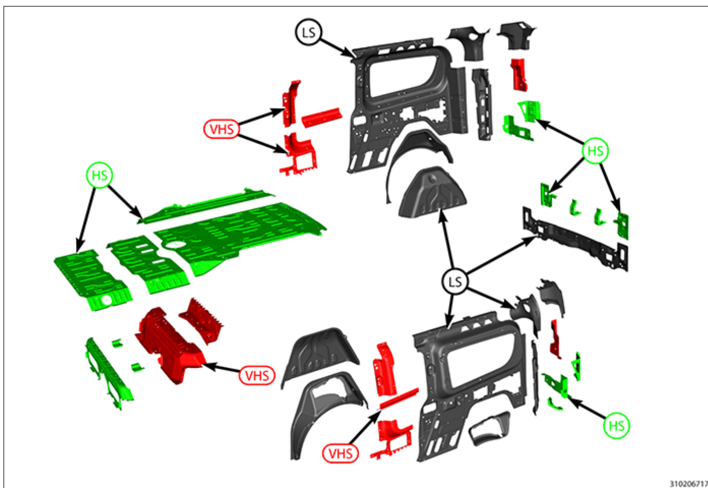
BODY IN WHITE COMPONENT IDENTIFICATION - INNER BODY SIDE, CENTER AND REAR FLOORS
