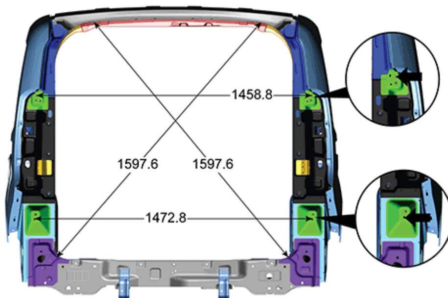
Rear Door Opening
