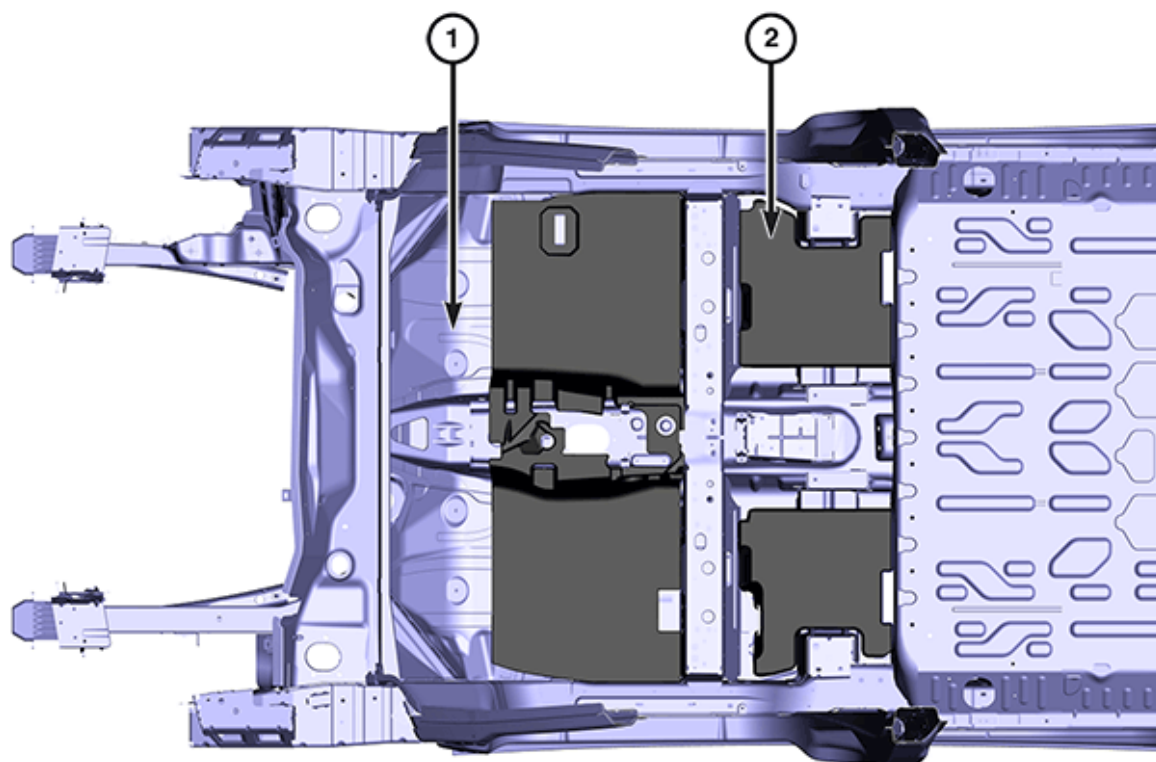
Front Floor (1 of 2)
