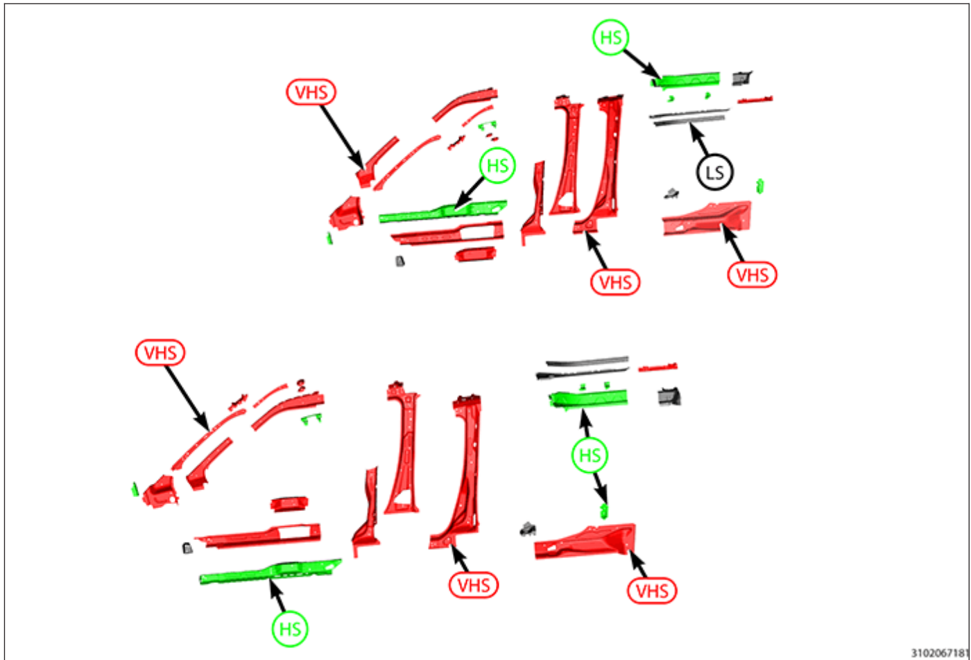
BODY IN WHITE COMPONENT IDENTIFICATION - INNER PILLARS, SILL AND SLIDING DOOR HEADER
