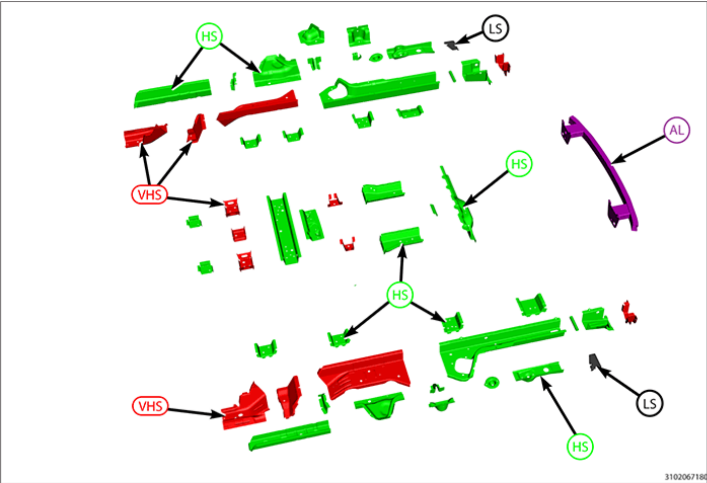
BODY IN WHITE COMPONENT IDENTIFICATION - REAR STRUCTURE
