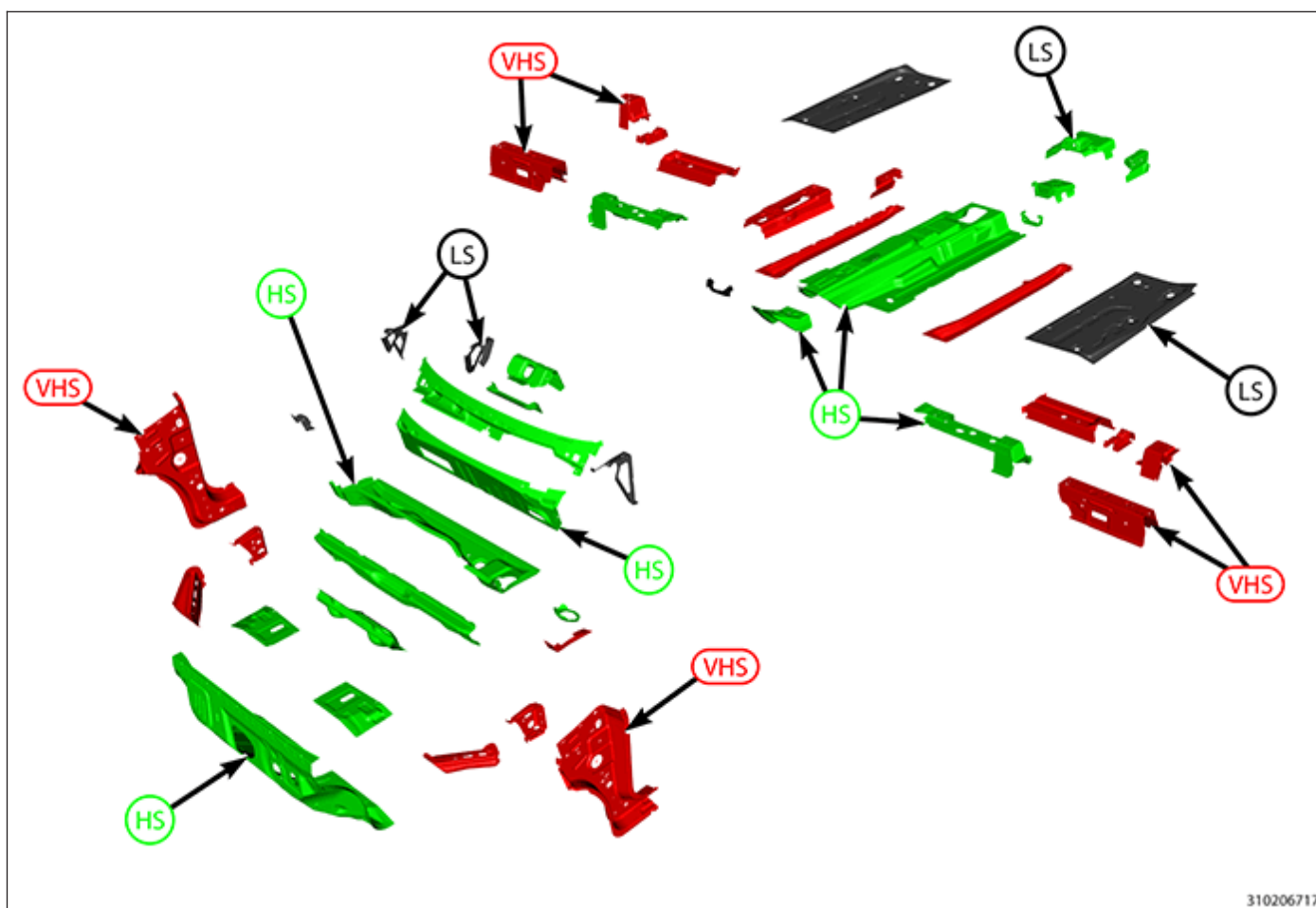
BODY IN WHITE COMPONENT IDENTIFICATION - DASH, COWL AND FRONT FLOOR
