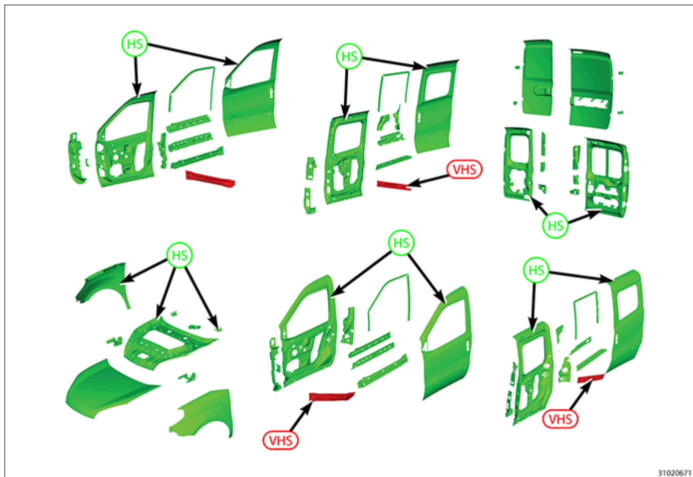
BODY IN WHITE COMPONENT IDENTIFICATION - CLOSURE PANELS
