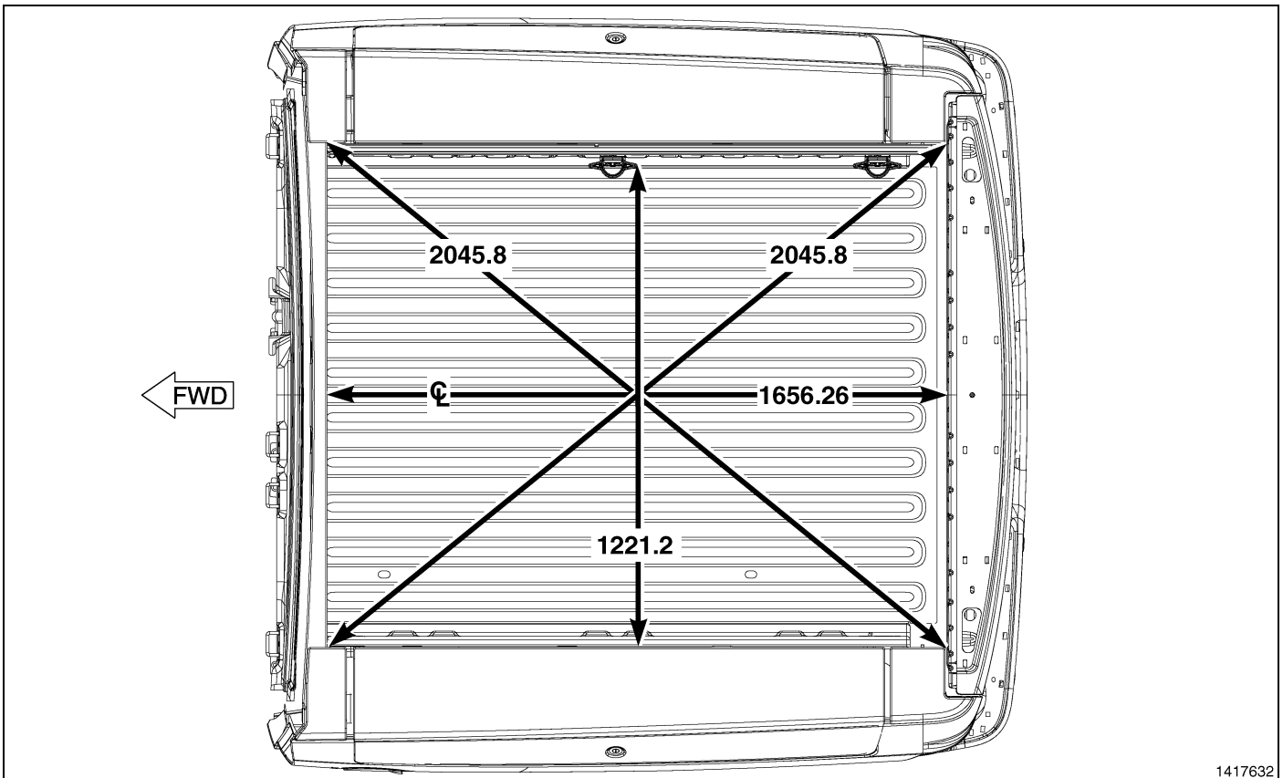
Fig. 7 Pickup Box - 5.7' Ram Box (Plan View)
