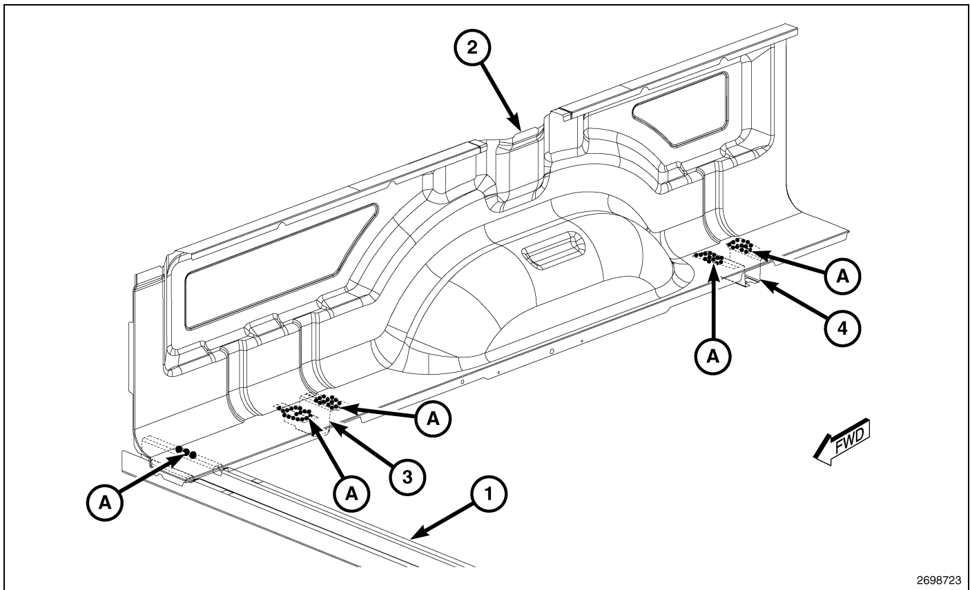
Fig. 87 8.0' Box Floor
