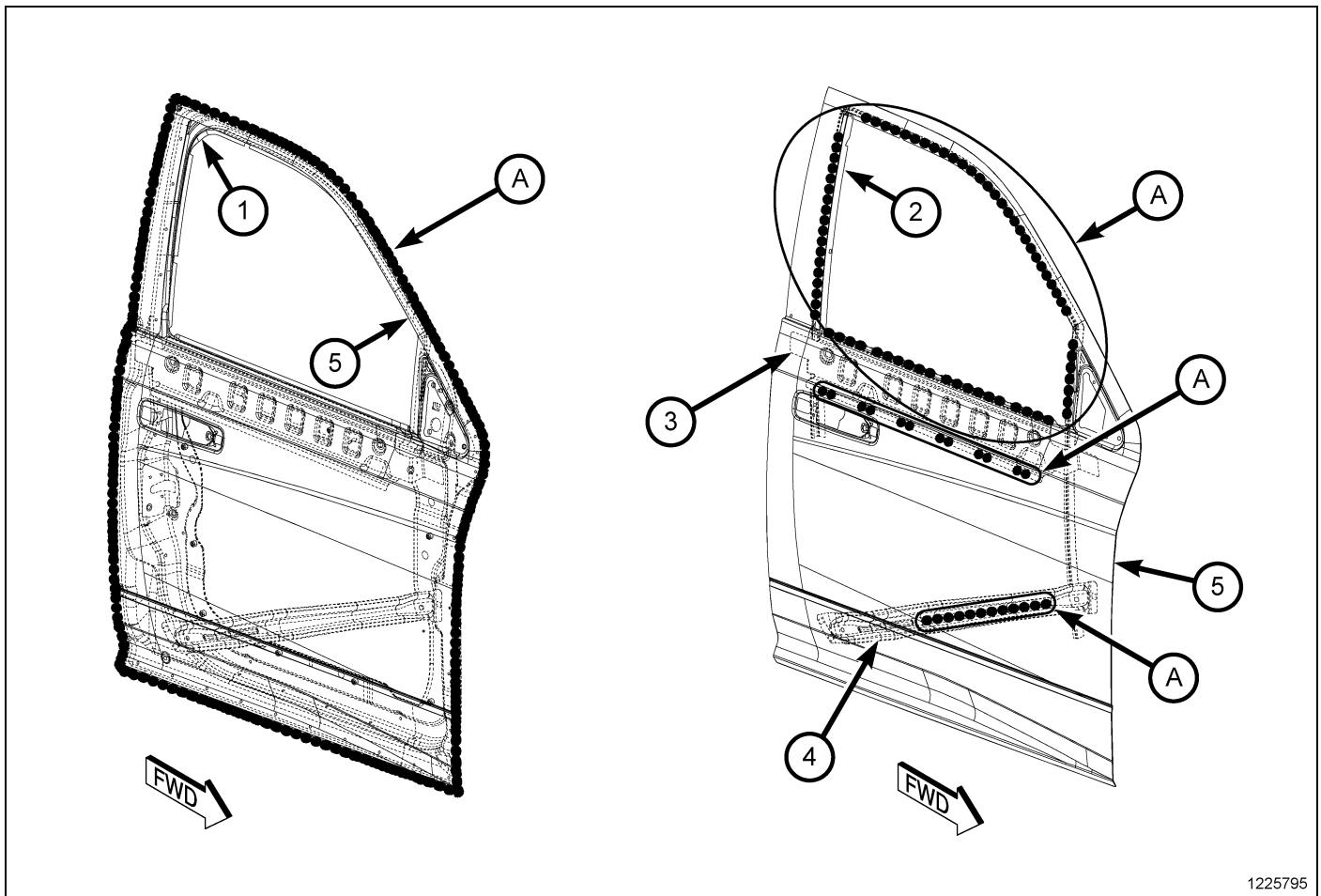
Fig. 88 Front Doors - Short
