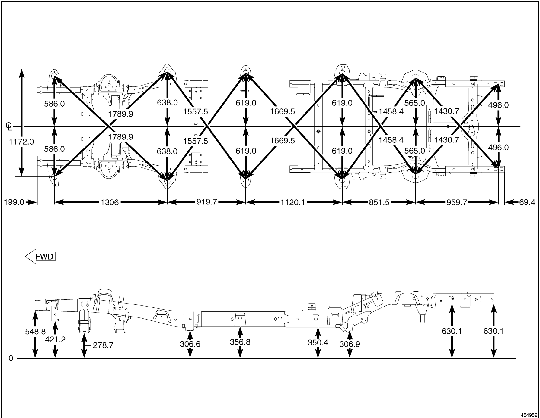
Fig. 16 140.5 In. Wheelbase – Crew Cab – 5.7 Ft. Box
