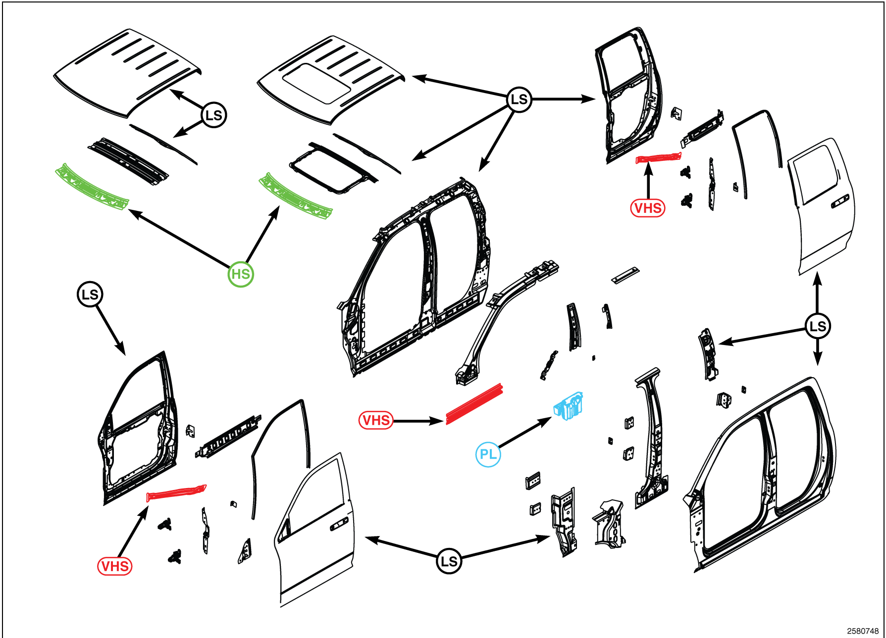
BODY IN WHITE COMPONENT IDENTIFICATION - BODY SIDE APERTURE, DOOR AND ROOF - QUAD CAB
