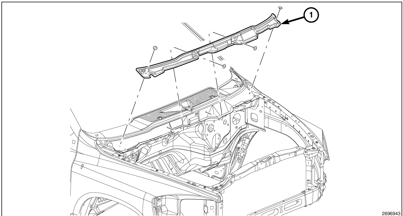
Fig. 34 COWL
