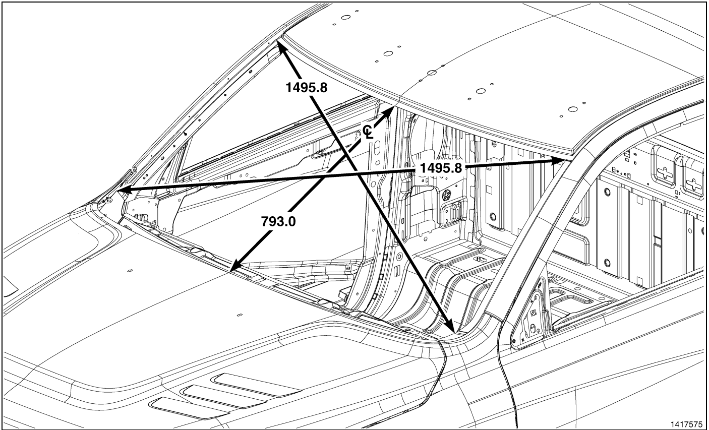
Fig. 2 Windshield Opening - All
