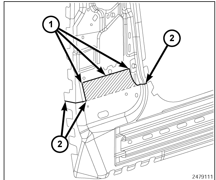
Fig. 22 Modified Lap Joint
