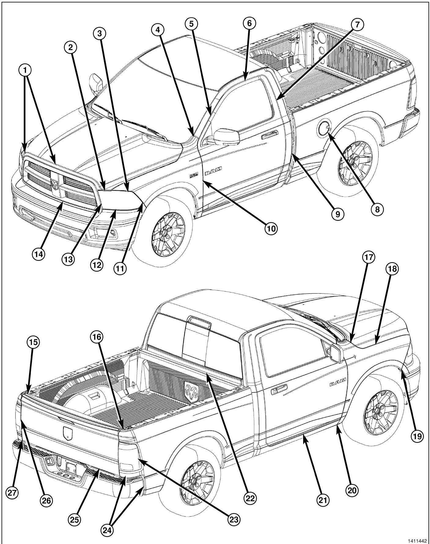
Fig. 17 REGULAR CAB
