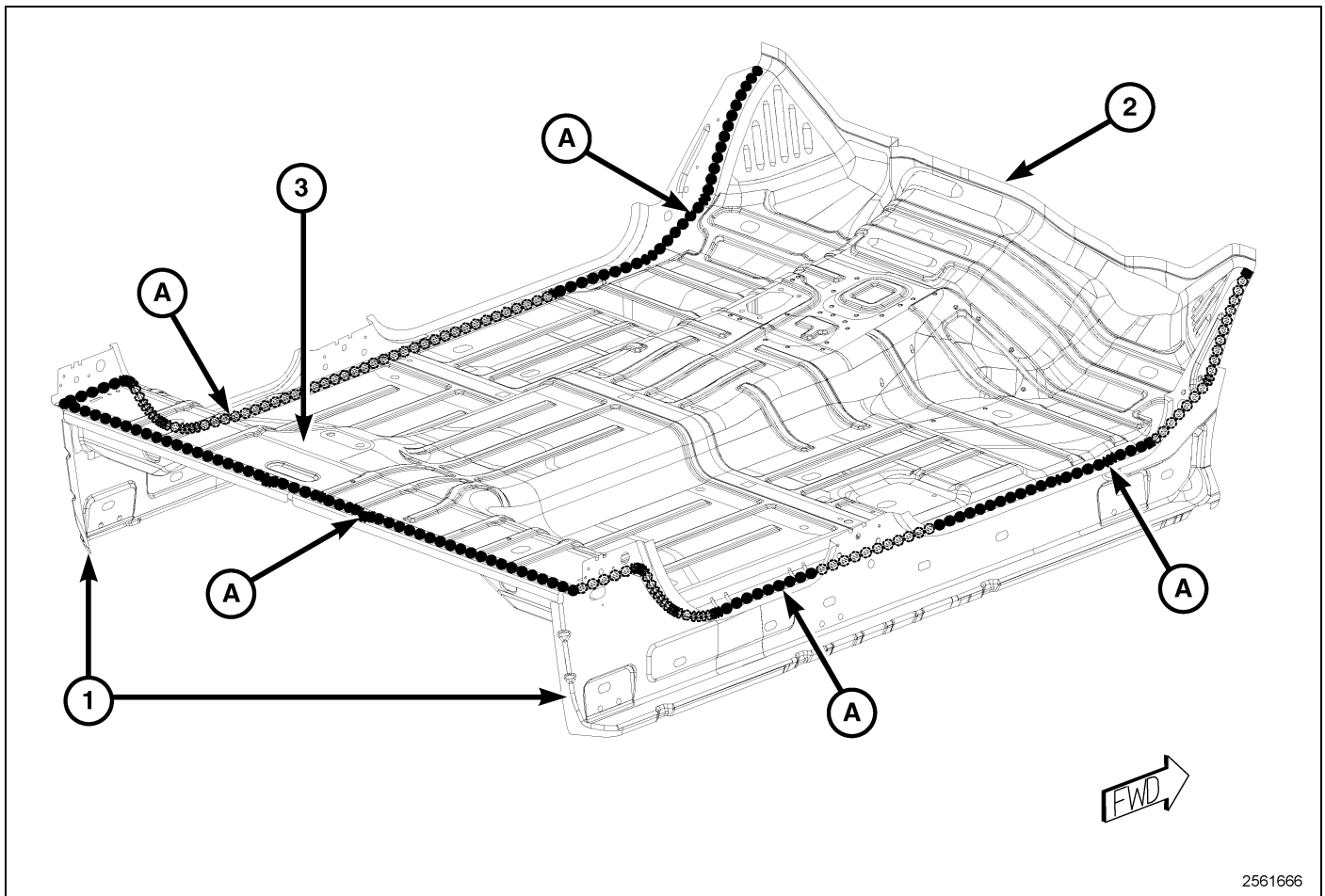
Fig. 66 Underbody Complete – Quad Cab
