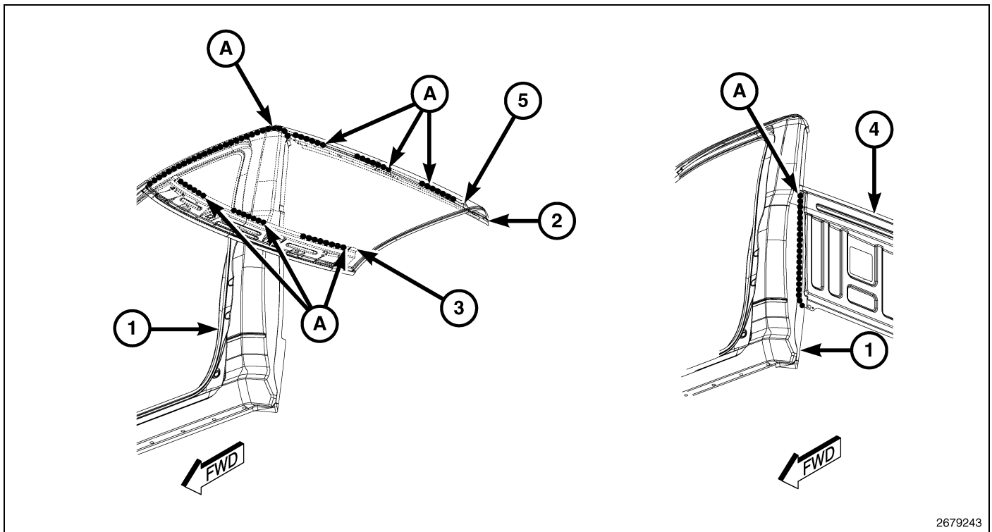
Fig. 72 Cab Complete – Standard (2 of 2)
