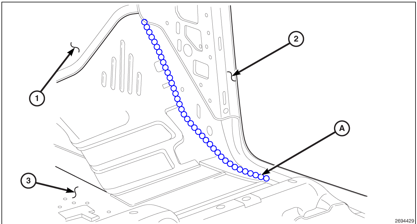
Fig. 50 Dash Panel/Front Floor Pan/Cowl Side Panel (2 of 2)
