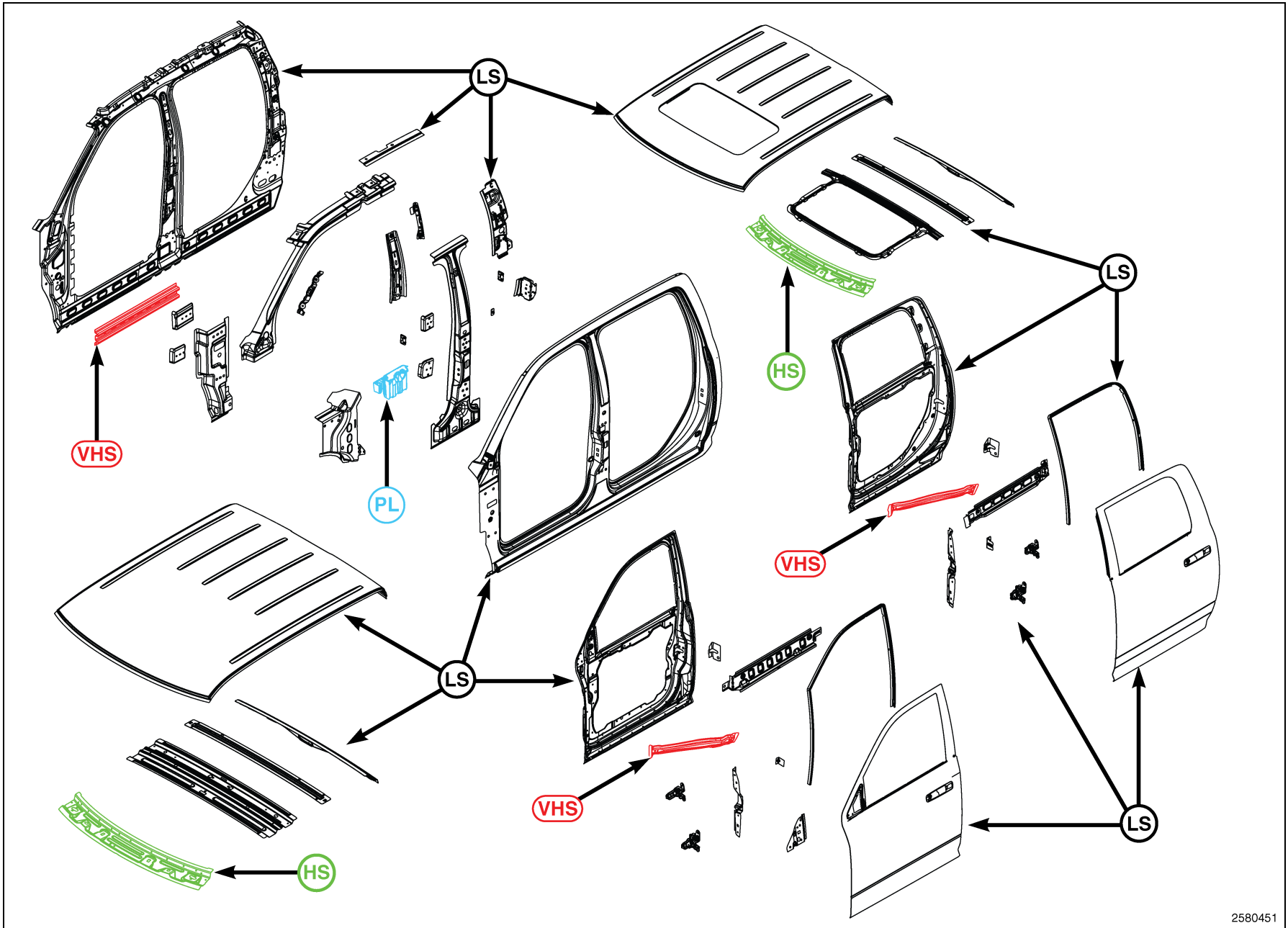
BODY IN WHITE COMPONENT IDENTIFICATION - BODY SIDE APERTURE, DOOR AND ROOF - CREW CAB
