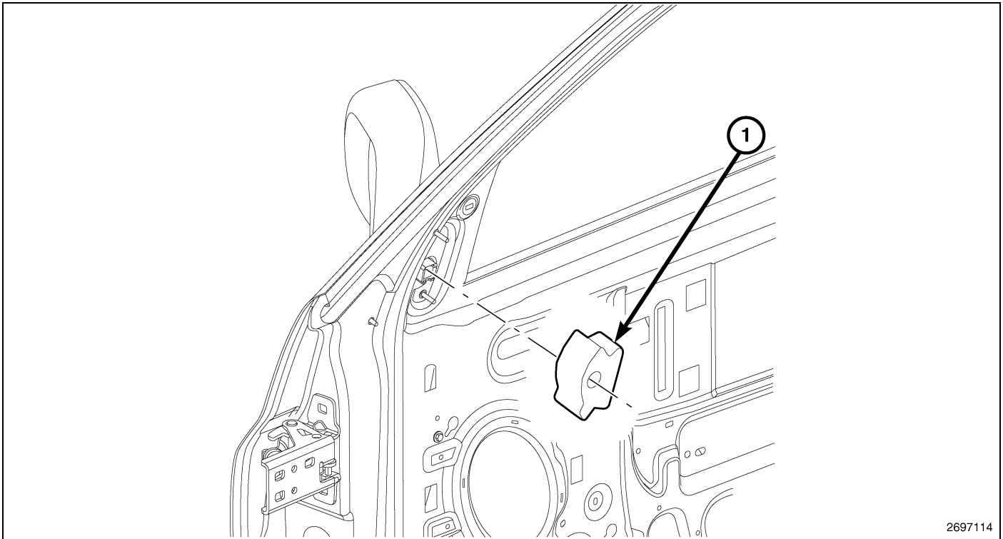
Fig. 40 FRONT DOORS
