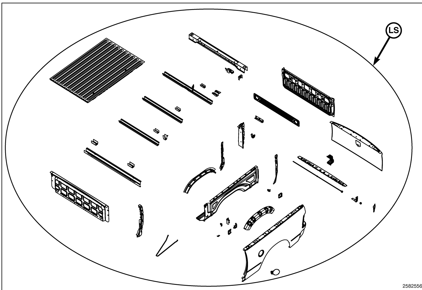
BODY IN WHITE COMPONENT IDENTIFICATION - PICKUP BOX - 6.3' SHOWN, 5.7' AND 8.0' TYPICAL, 5.7' RAMBOX SIMILAR
