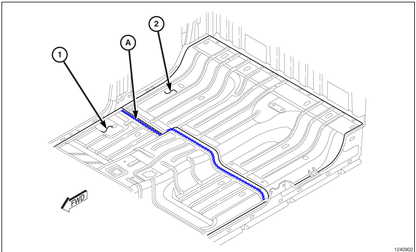
Fig. 52 Front Floor Pan/Rear Floor Pan
