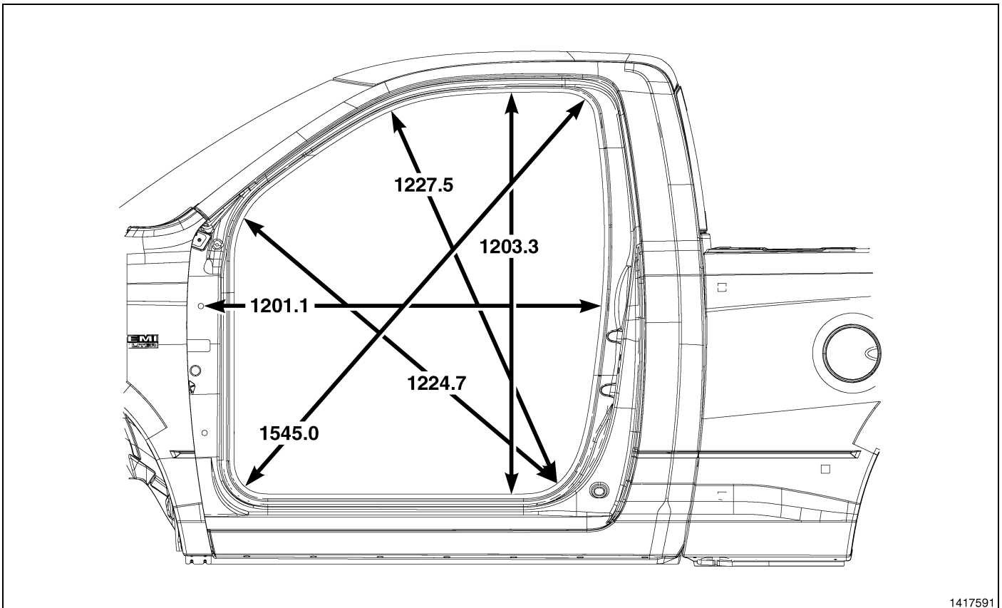
Fig. 3 Door Openings – Standard Cab
