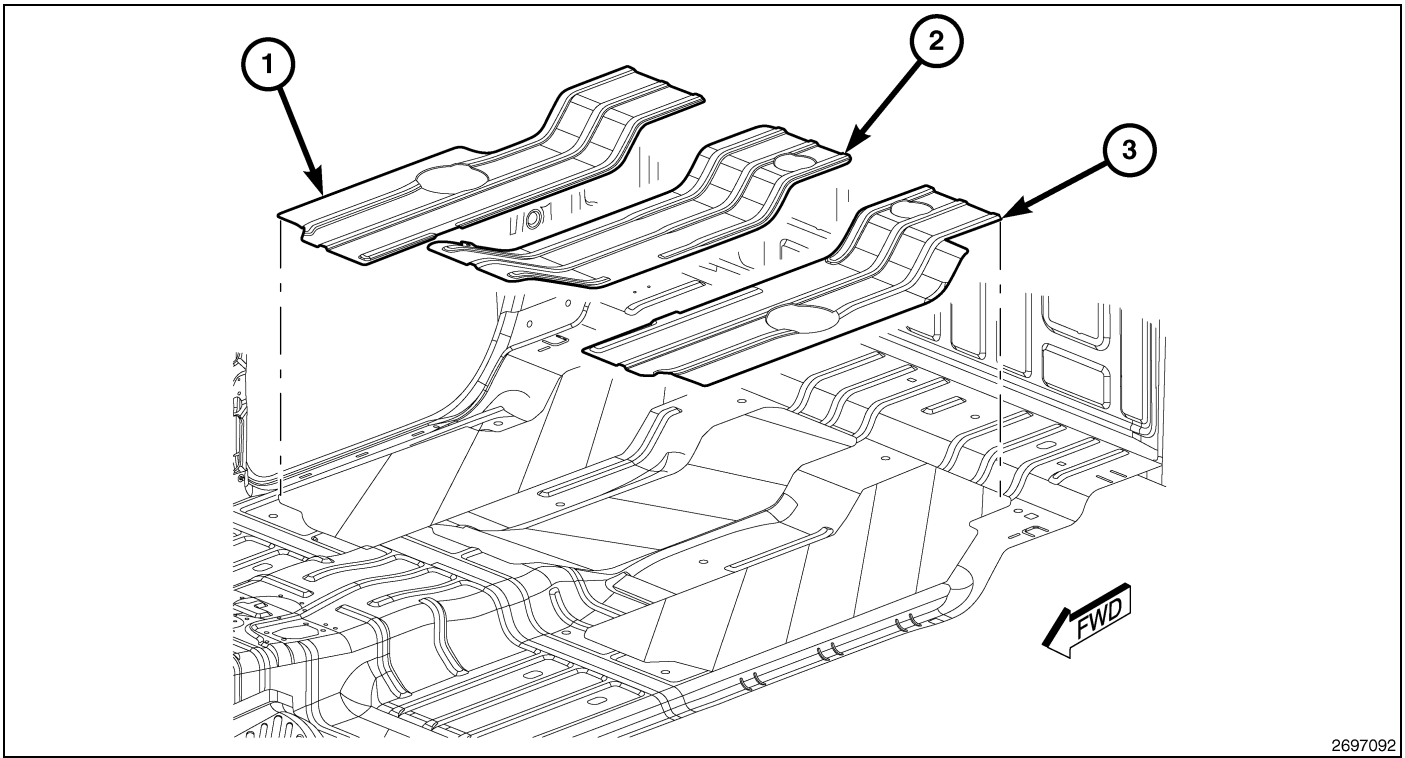
Fig. 39 REAR FLOOR PAN – CREW CAB
