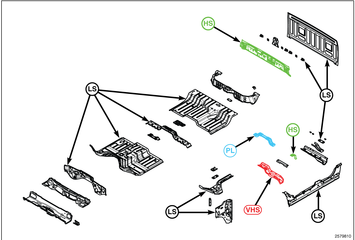
BODY IN WHITE COMPONENT IDENTIFICATION - UNDERBODY - QUAD CAB
