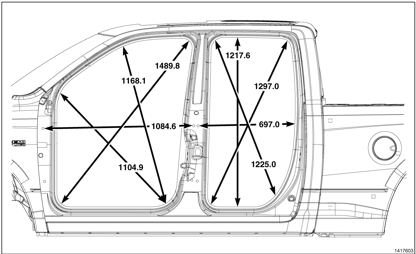
Fig. 4 Door Openings – Quad Cab
