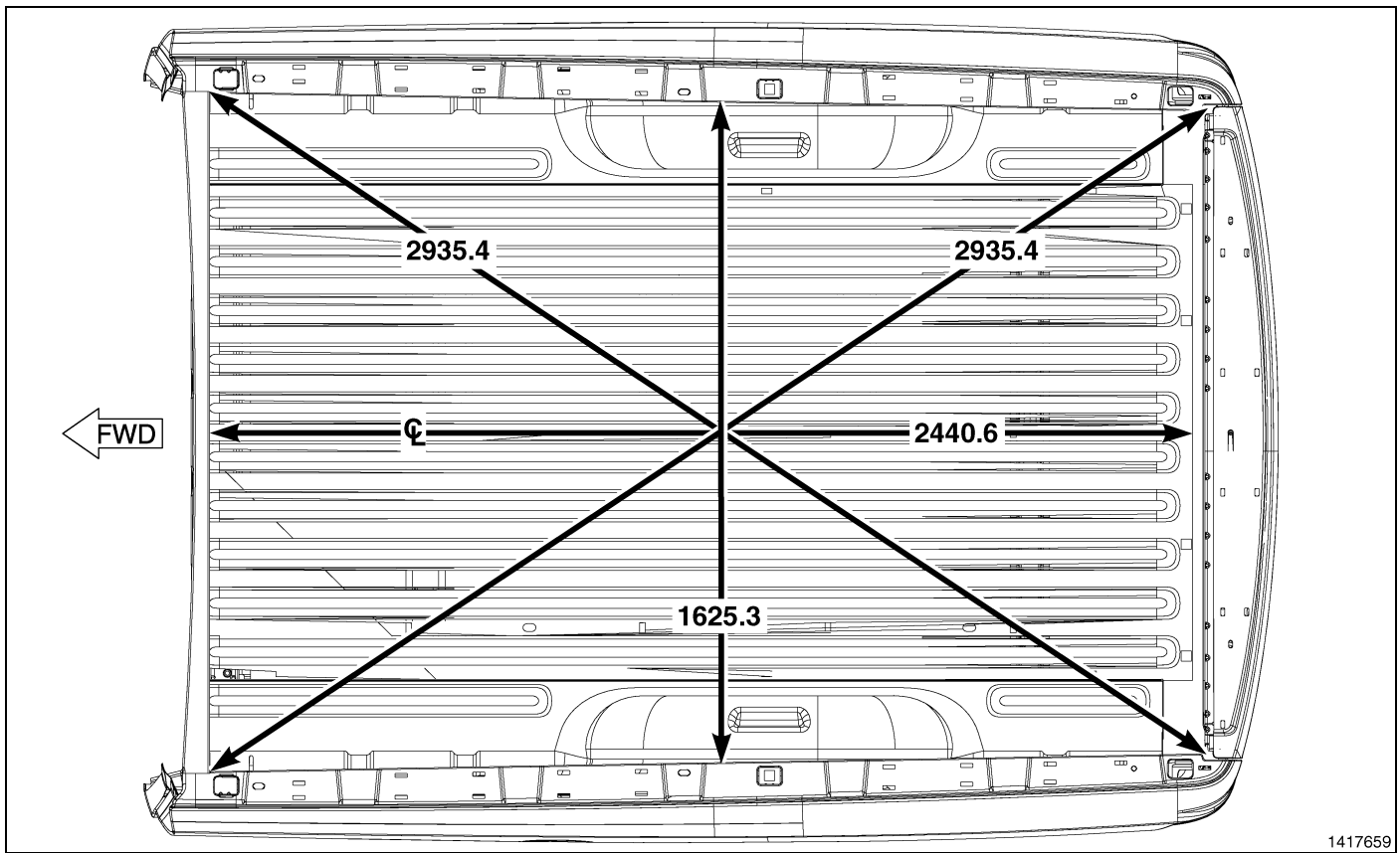
Fig. 10 Pickup Box – 8.0' Box (Plan View)
