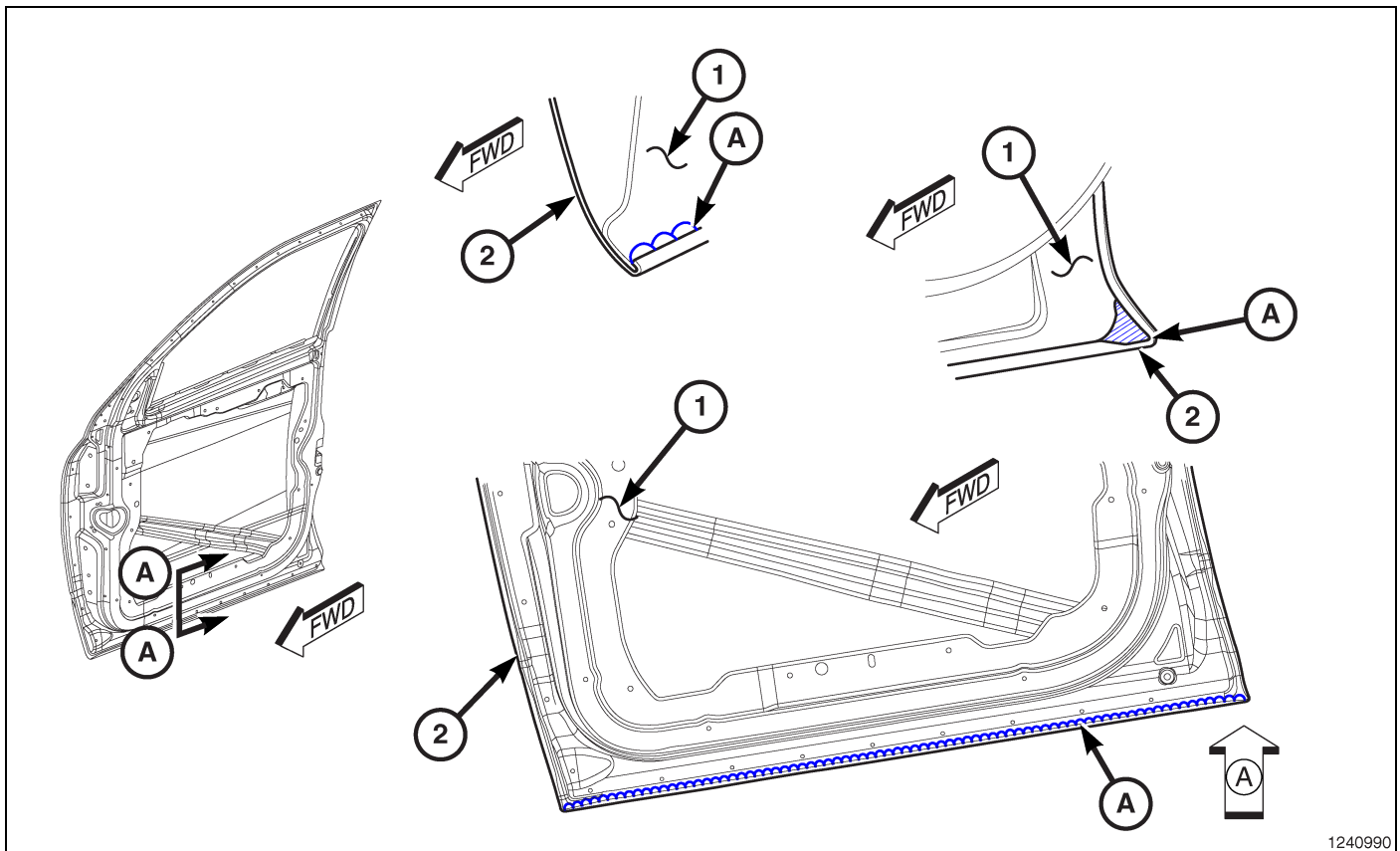
Fig. 60 Front Door – Quad, Crew Cab
