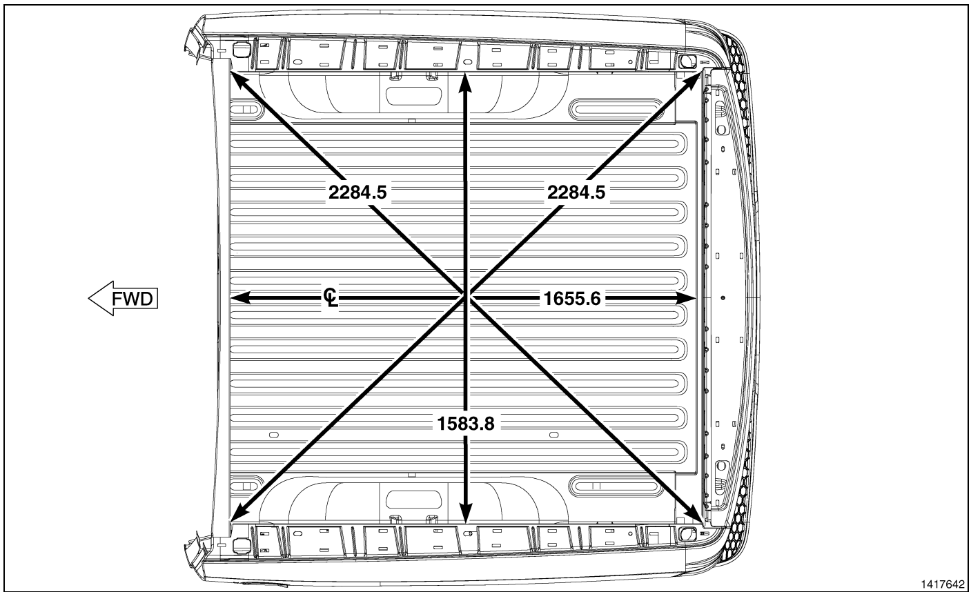
Fig. 8 Pickup Box – 5.7' Box (Plan View)
