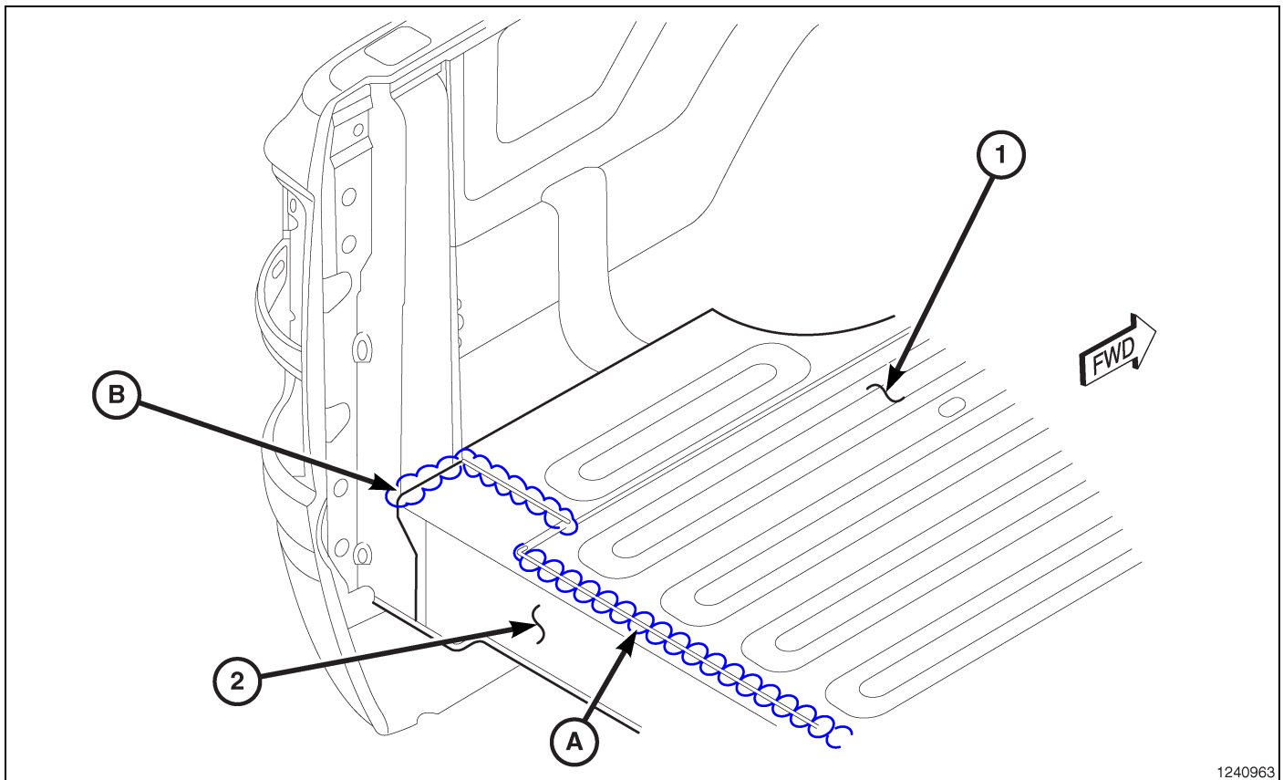
Fig. 57 Box Floor Panel/Box Floor Extension
