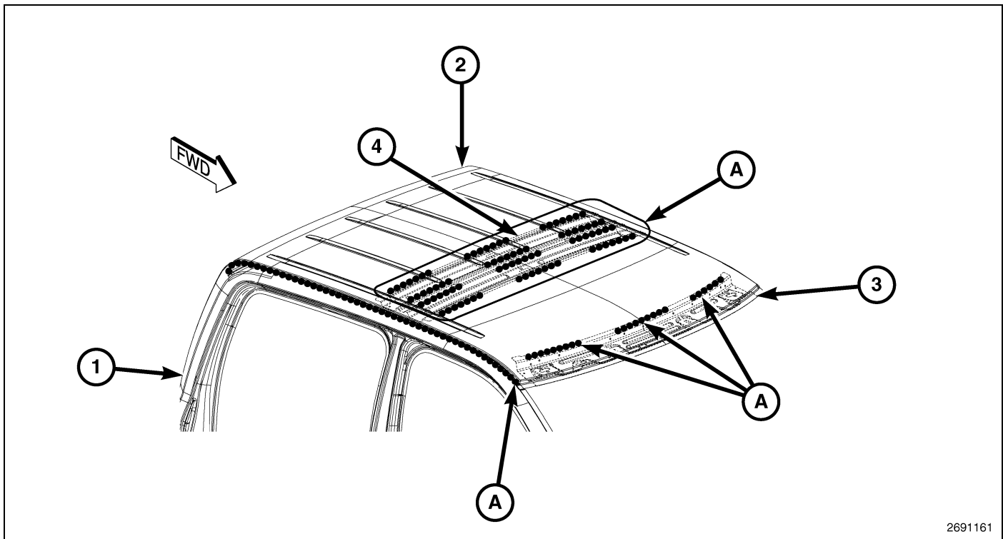
Fig. 79 Cab Complete – Crew (3 of 5)
