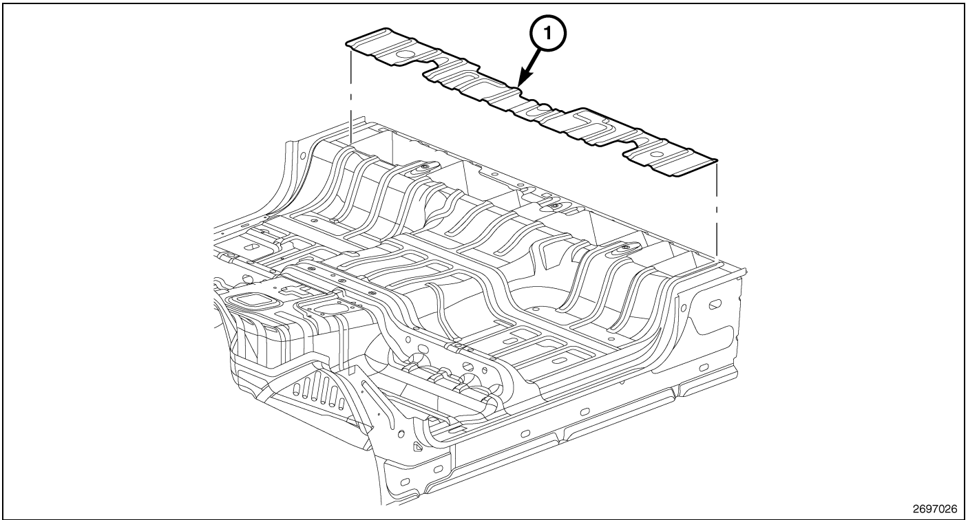
Fig. 37 REAR FLOOR PAN – STANDARD CAB
