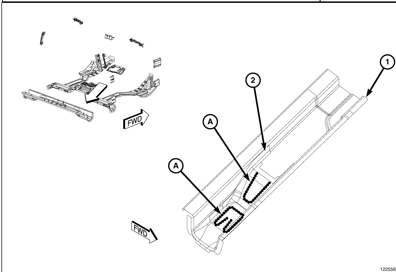
Fig. 63 MISCELLANEOUS COMPONENTS - STANDARD AND QUAD CAB ONLY
