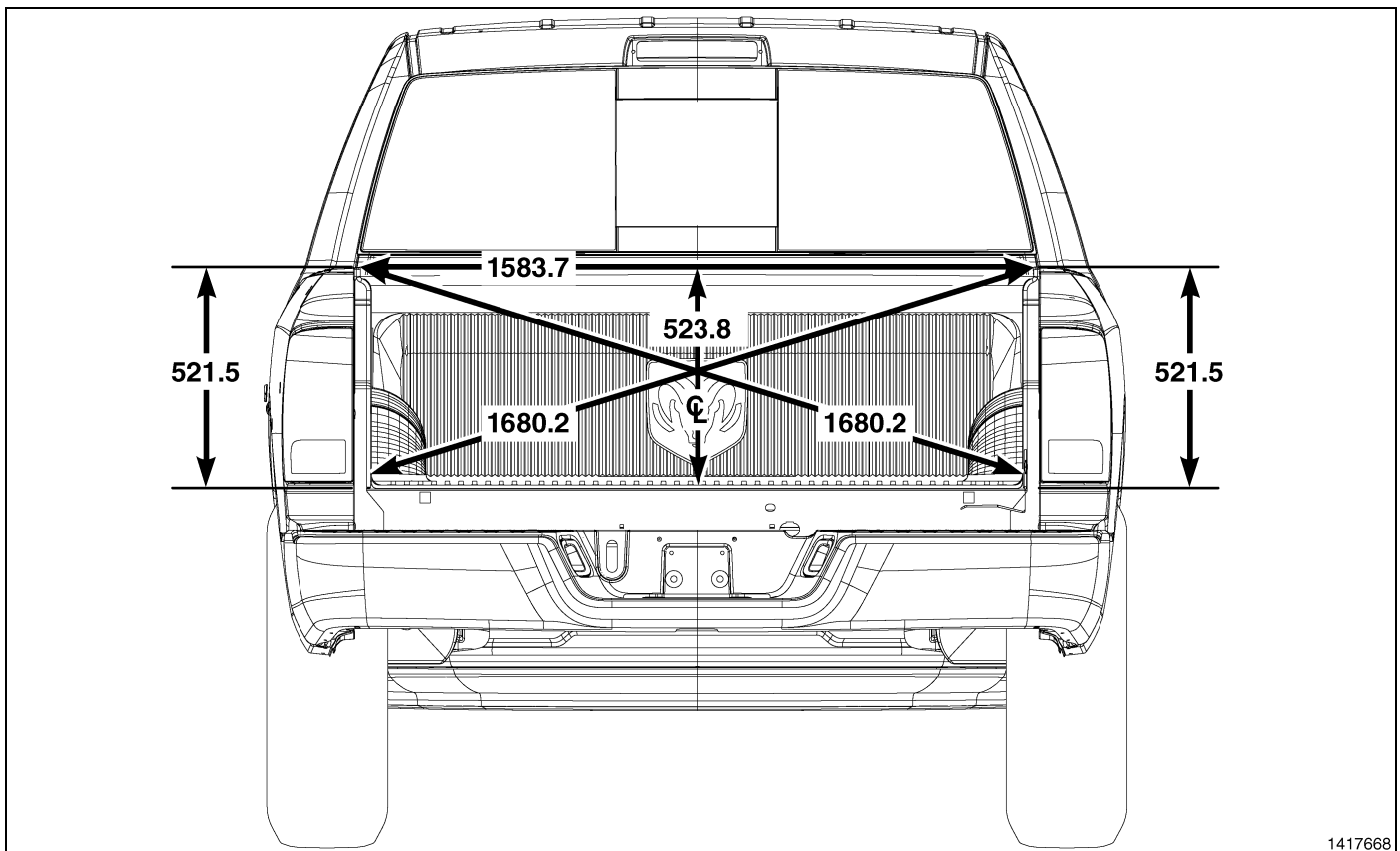
Fig. 11 Pickup Box – Tail Gate Opening - All
