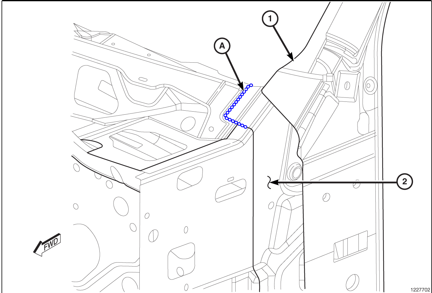
Fig. 46 Inner Body Side Panel and Cowl Side Panel
