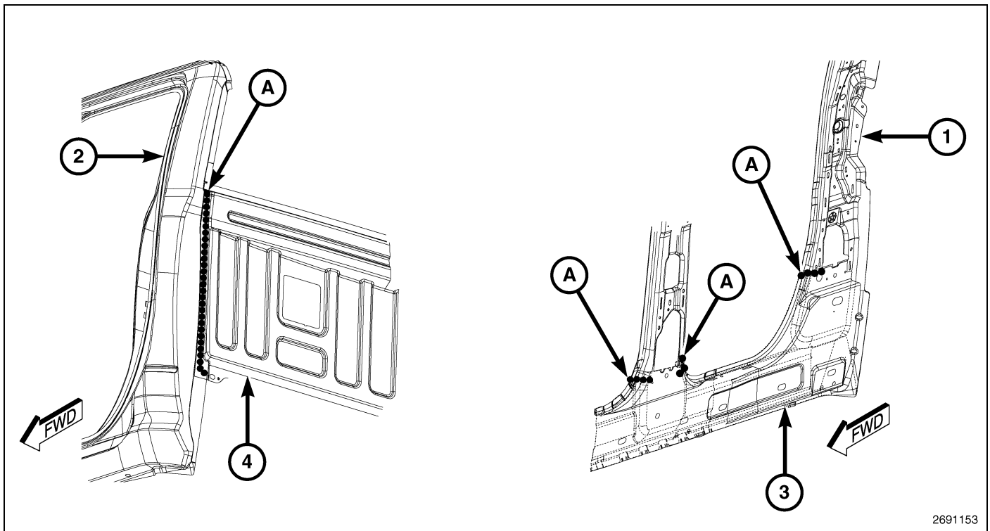
Fig. 78 Cab Complete – Crew (2 of 5)
