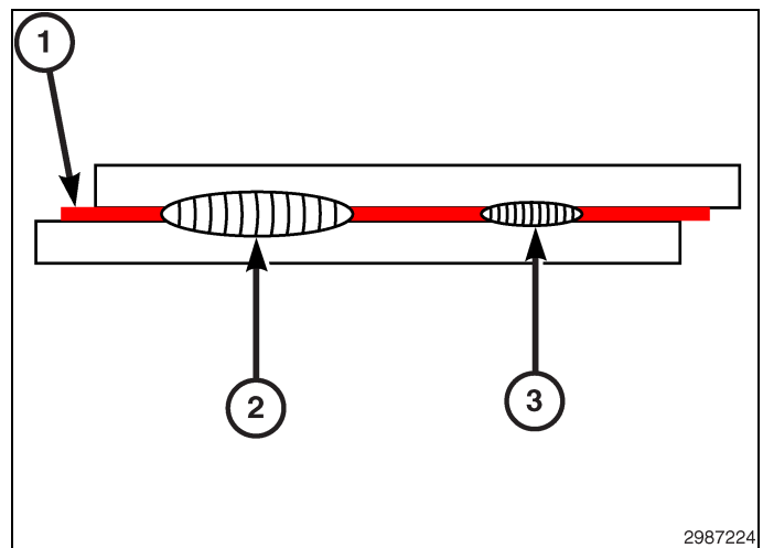
Fig. 25 Current Level Medium for Both Welds
