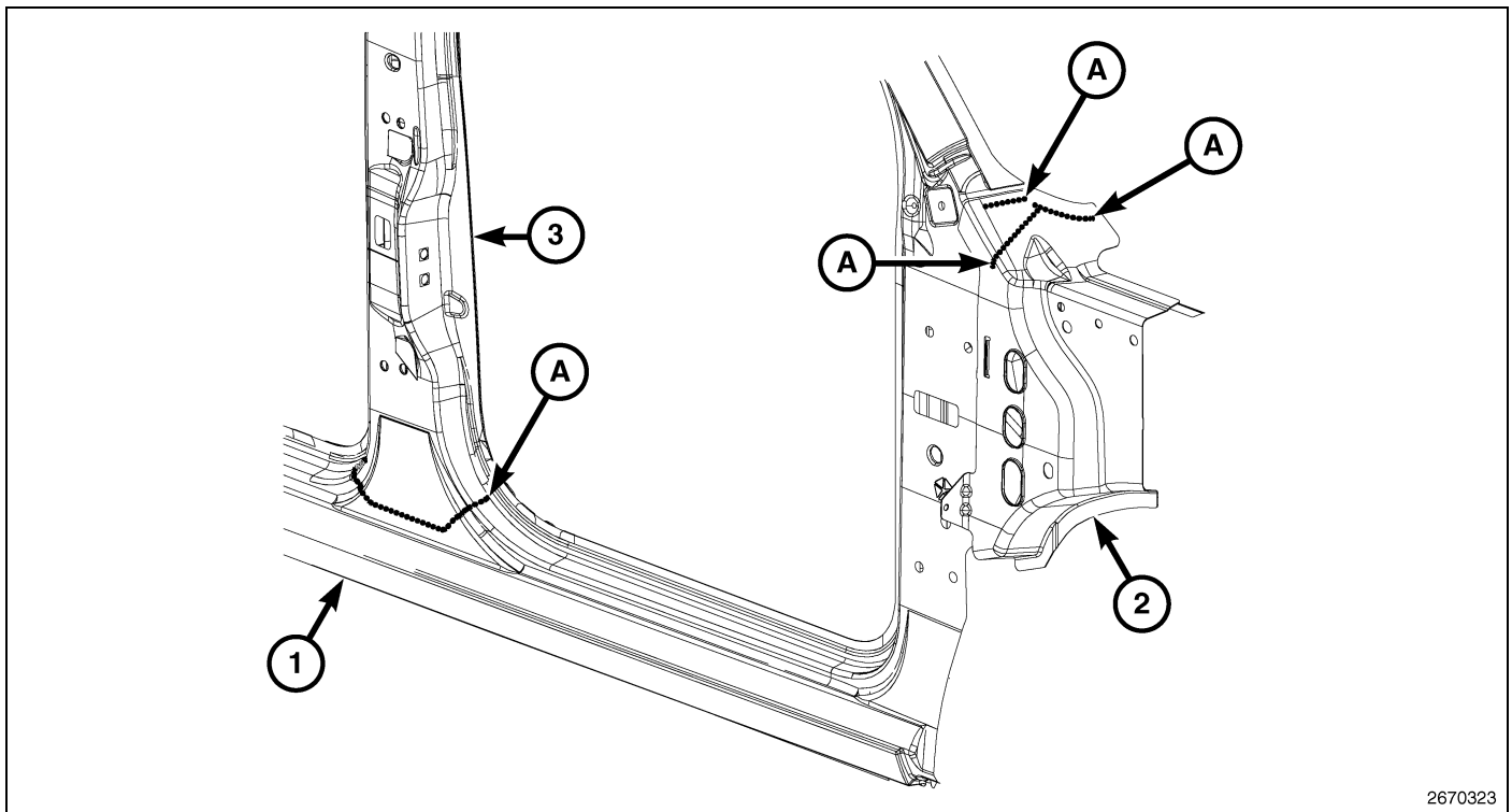
Fig. 70 Body Side Aperture Outer – Crew Cab (2 of 2)
