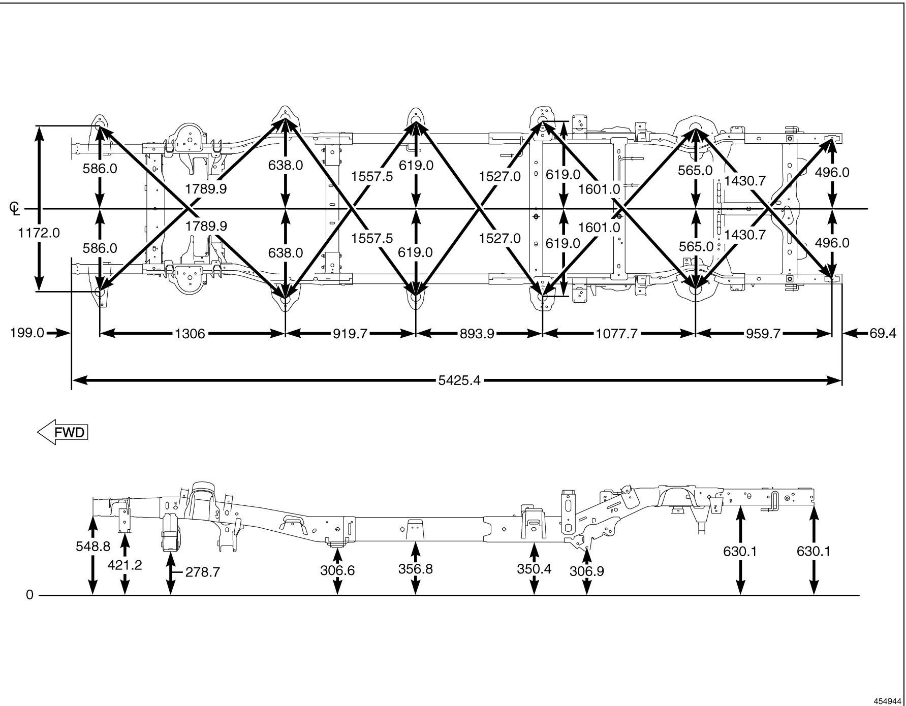
Fig. 15 140.5 In. Wheelbase – Quad Cab – 6.3 Ft. Box
