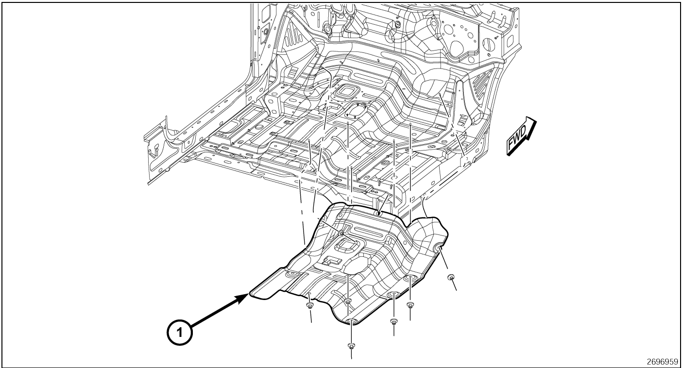
Fig. 35 FLOOR PAN TUNNEL
