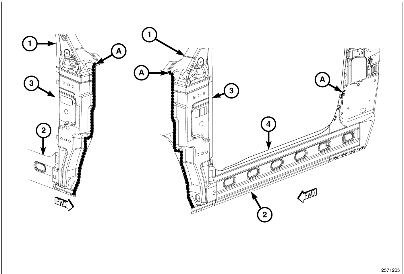
Fig. 68 Body Side Aperture Complete – Standard Cab
