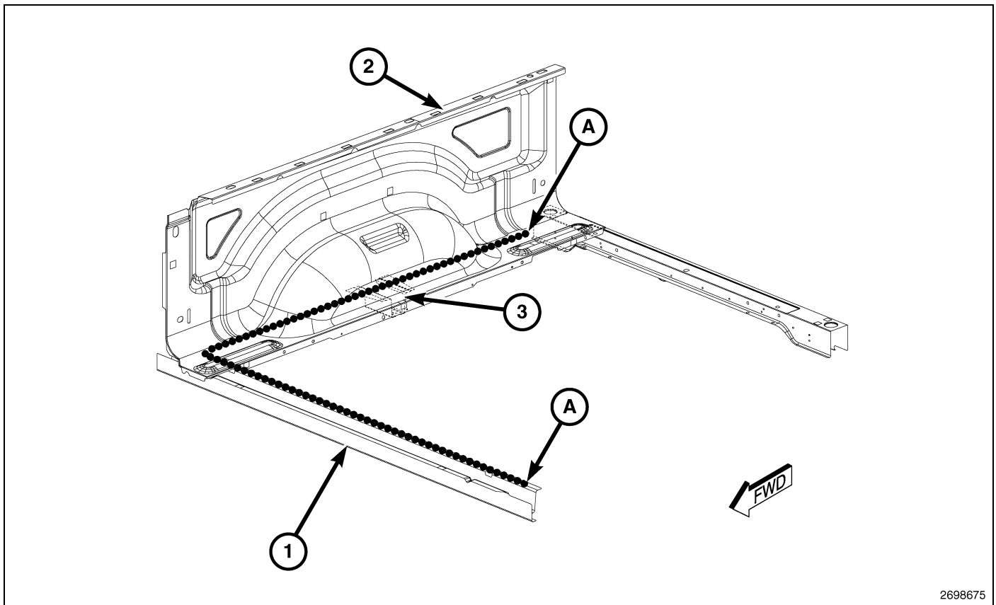
Fig. 84 6.3' Box Floor
