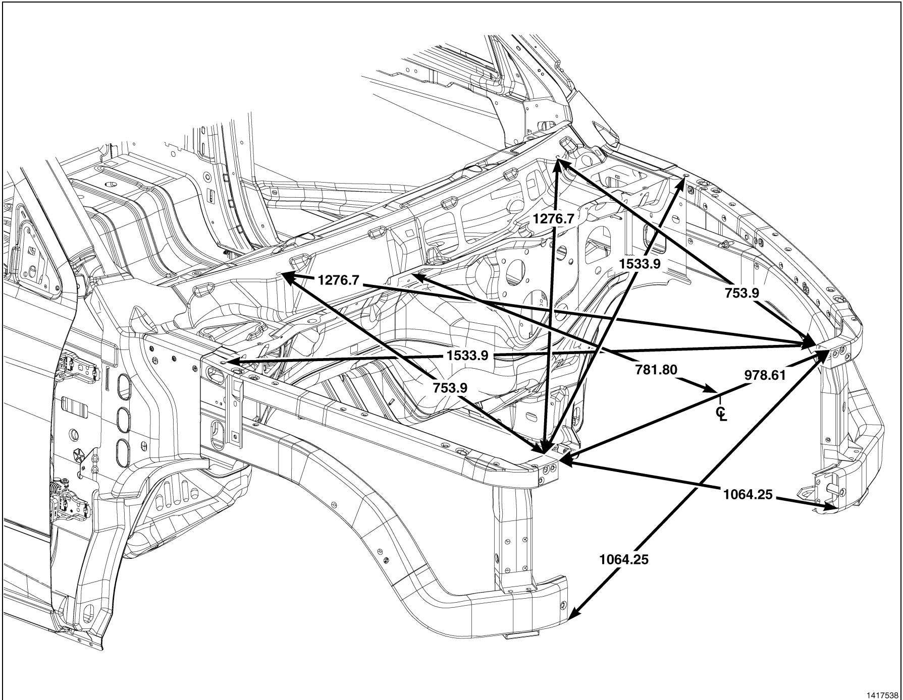
Fig. 30 Engine Compartment/Body Structure
