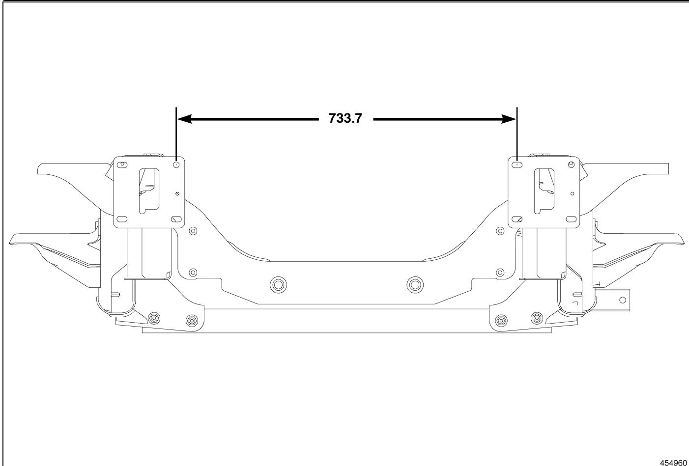
Fig. 12 Front View – All
