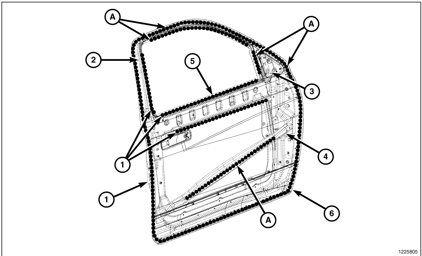
Fig. 89 Front Doors - Long
