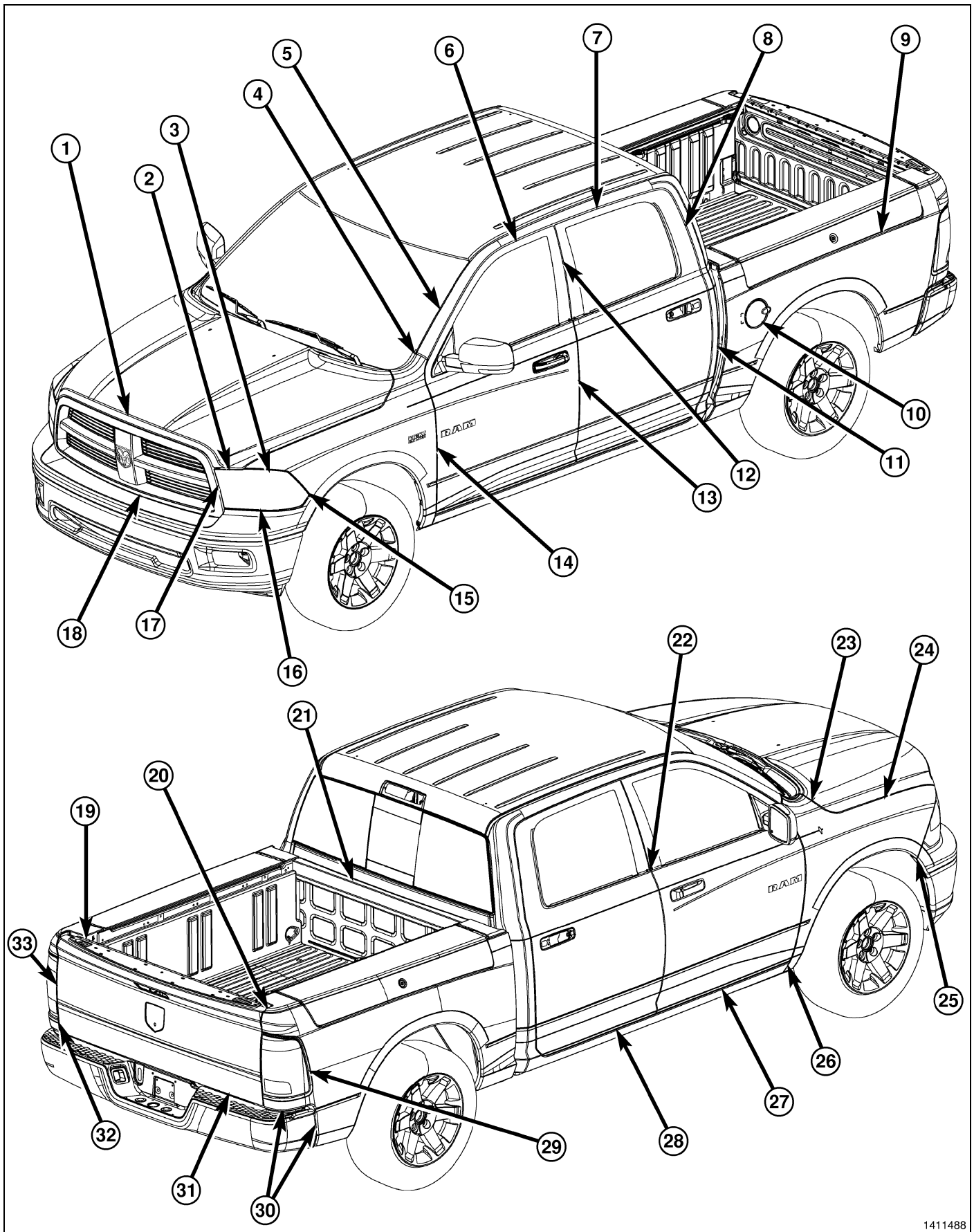
Fig. 19 CREW CAB
