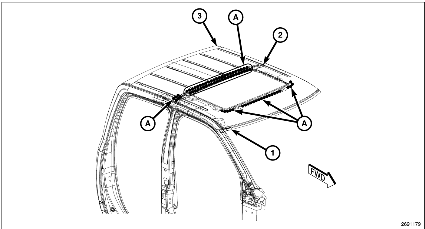
Fig. 81 Cab Complete – Crew (5 of 5)
