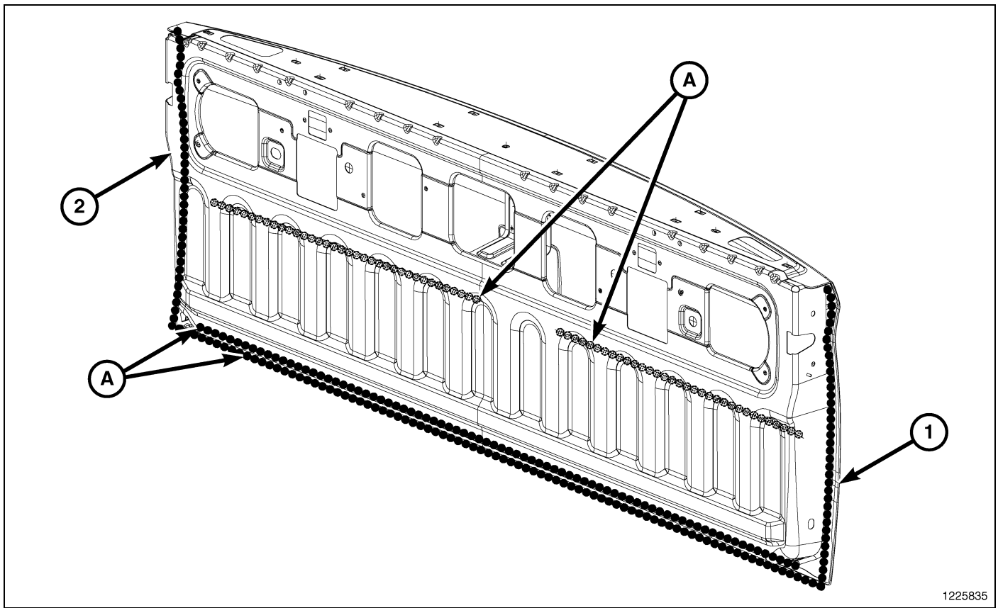
Fig. 92 Tailgate
