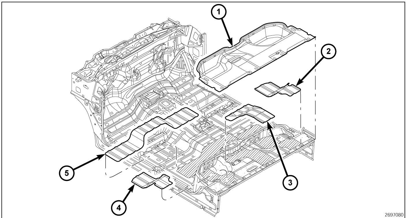
Fig. 38 REAR FLOOR PAN – QUAD CAB
