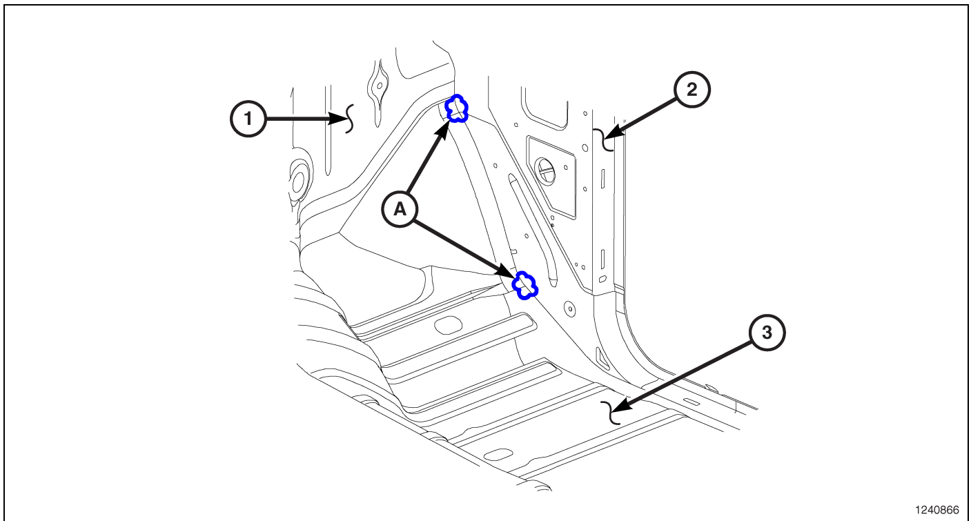
Fig. 49 Dash Panel/Front Floor Pan/Cowl Side Panel (1 of 2)
