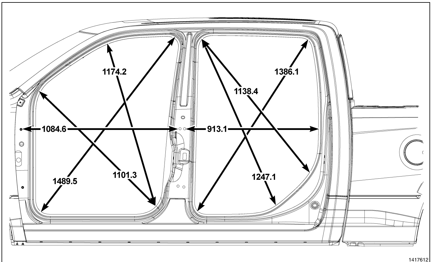
Fig. 5 Door Openings – Crew Cab
