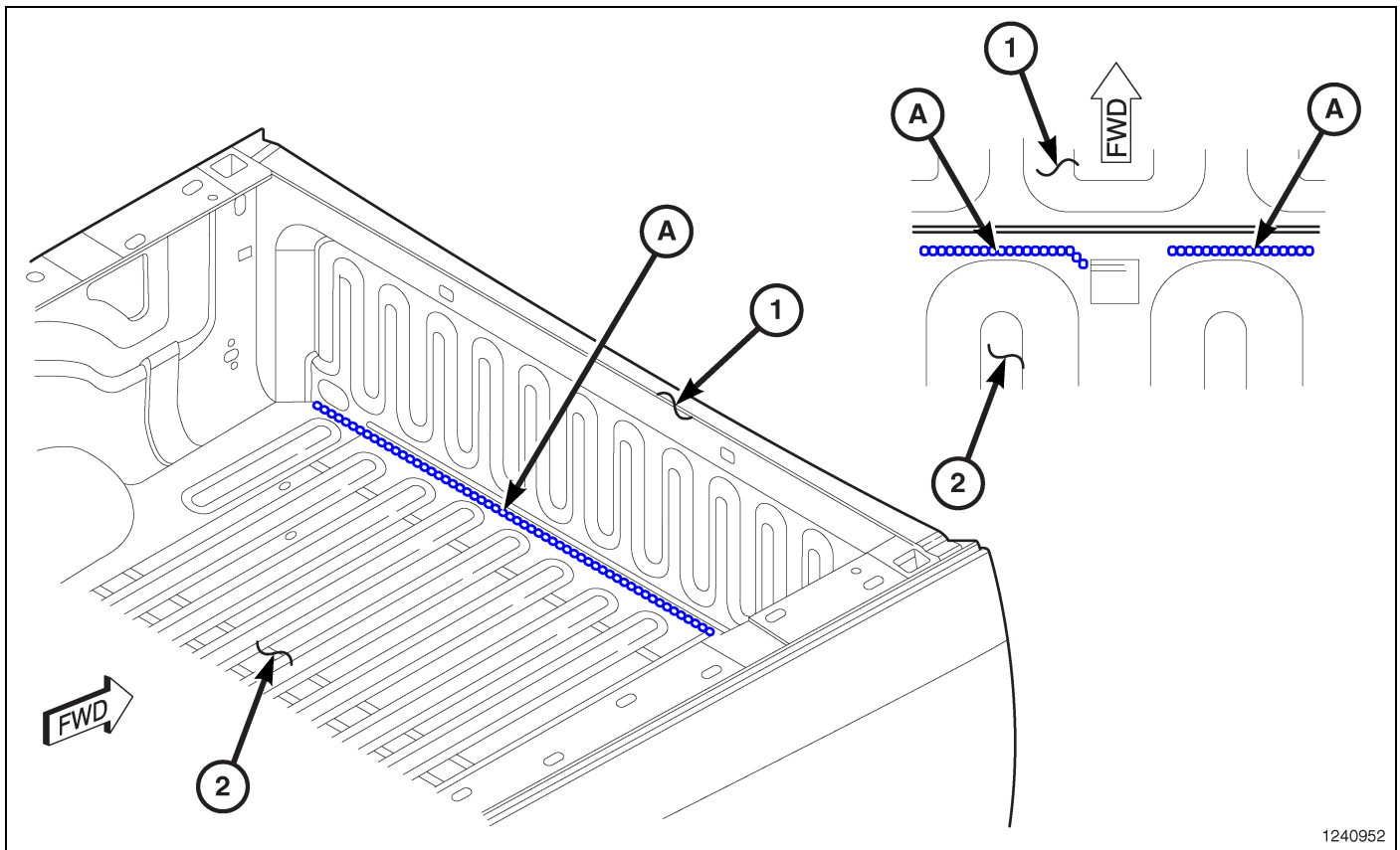
Fig. 56 Box Floor Panel/Box Front Panel
