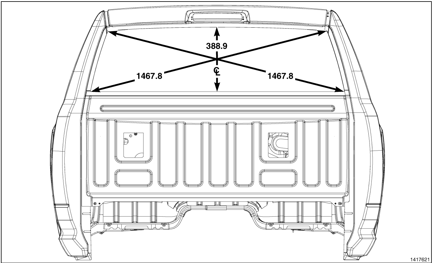
Fig. 6 Rear Window Opening - All
