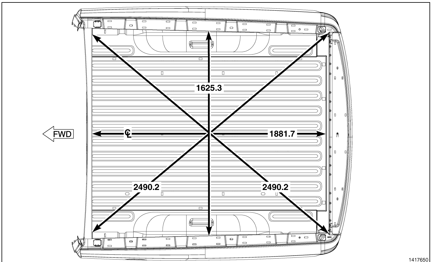
Fig. 9 Pickup Box – 6.3' Box (Plan View)
