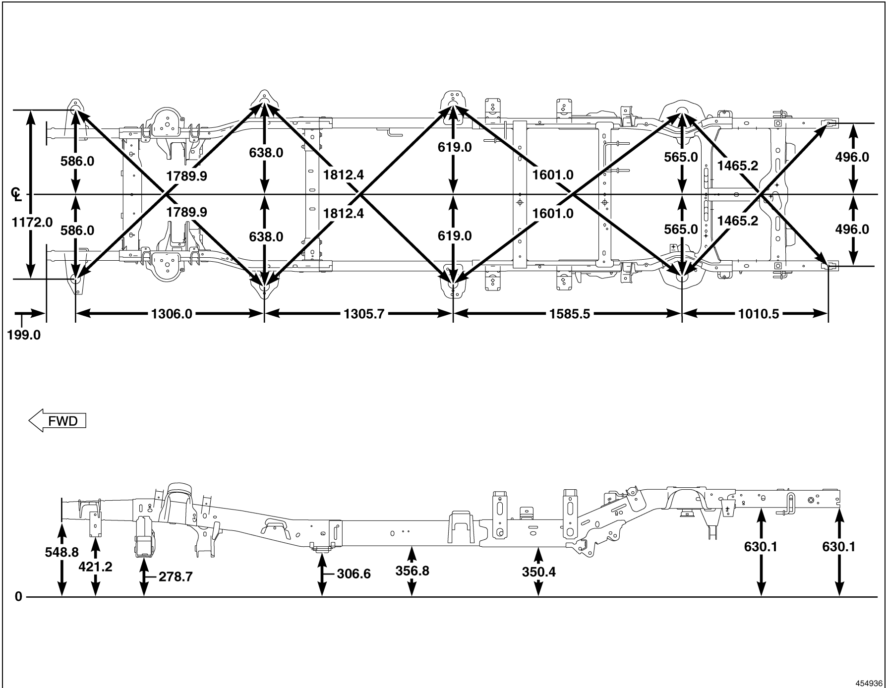
Fig. 14 140.5 In. Wheelbase – Regular Cab – 8.0 Ft. Box
