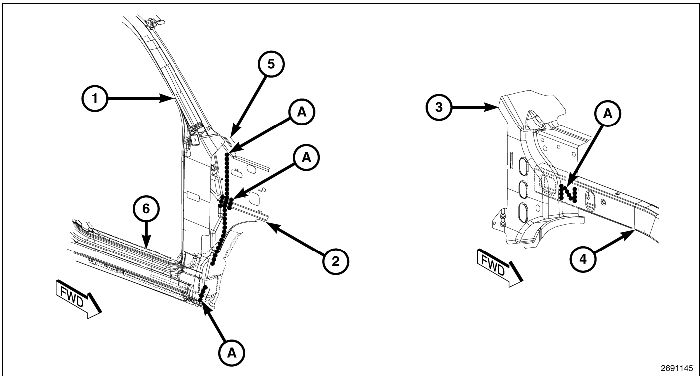
Fig. 77 Cab Complete – Crew (1 of 5)
