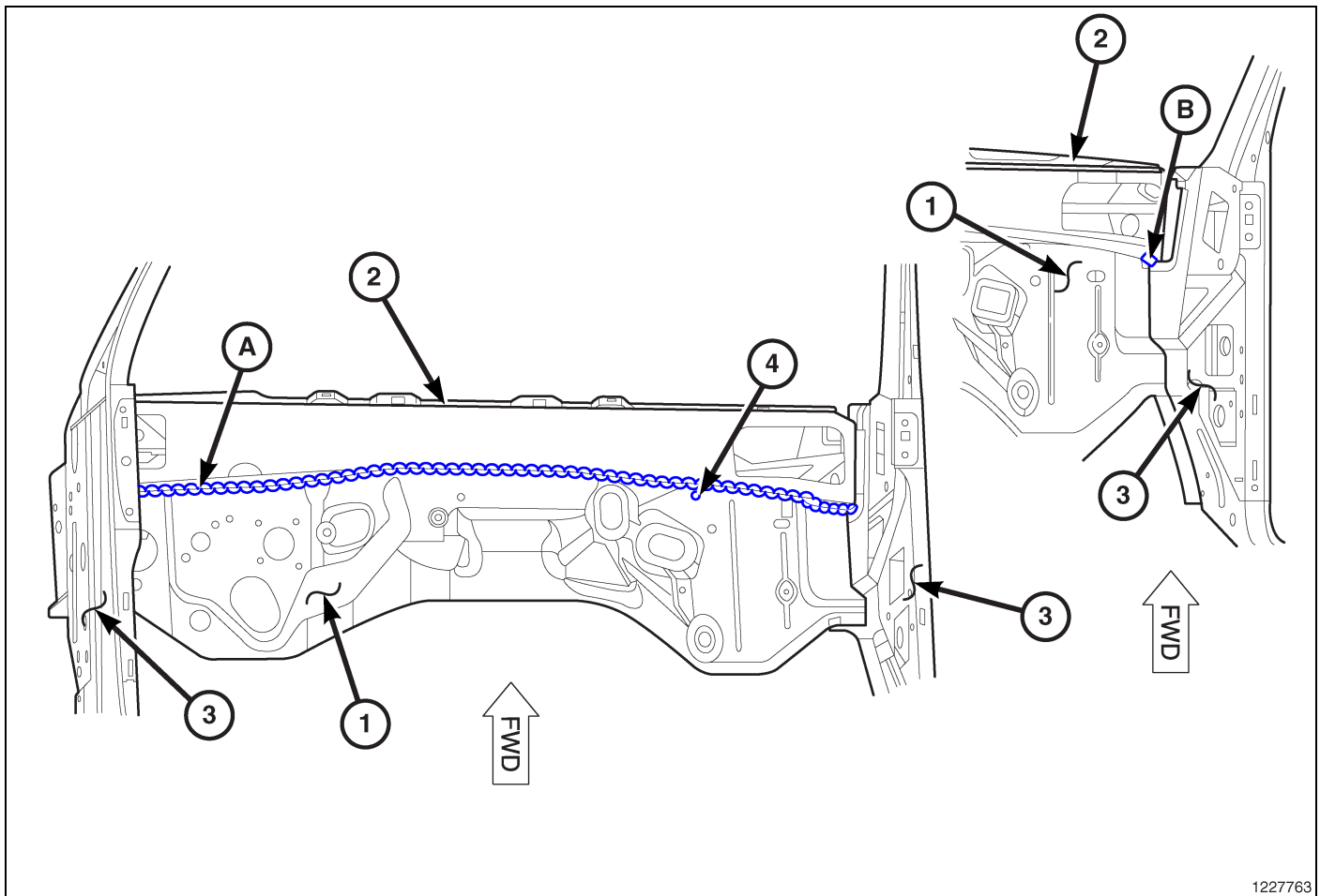
Fig. 47 Dash Panel/Cowl Side Panel (1 of 2)
