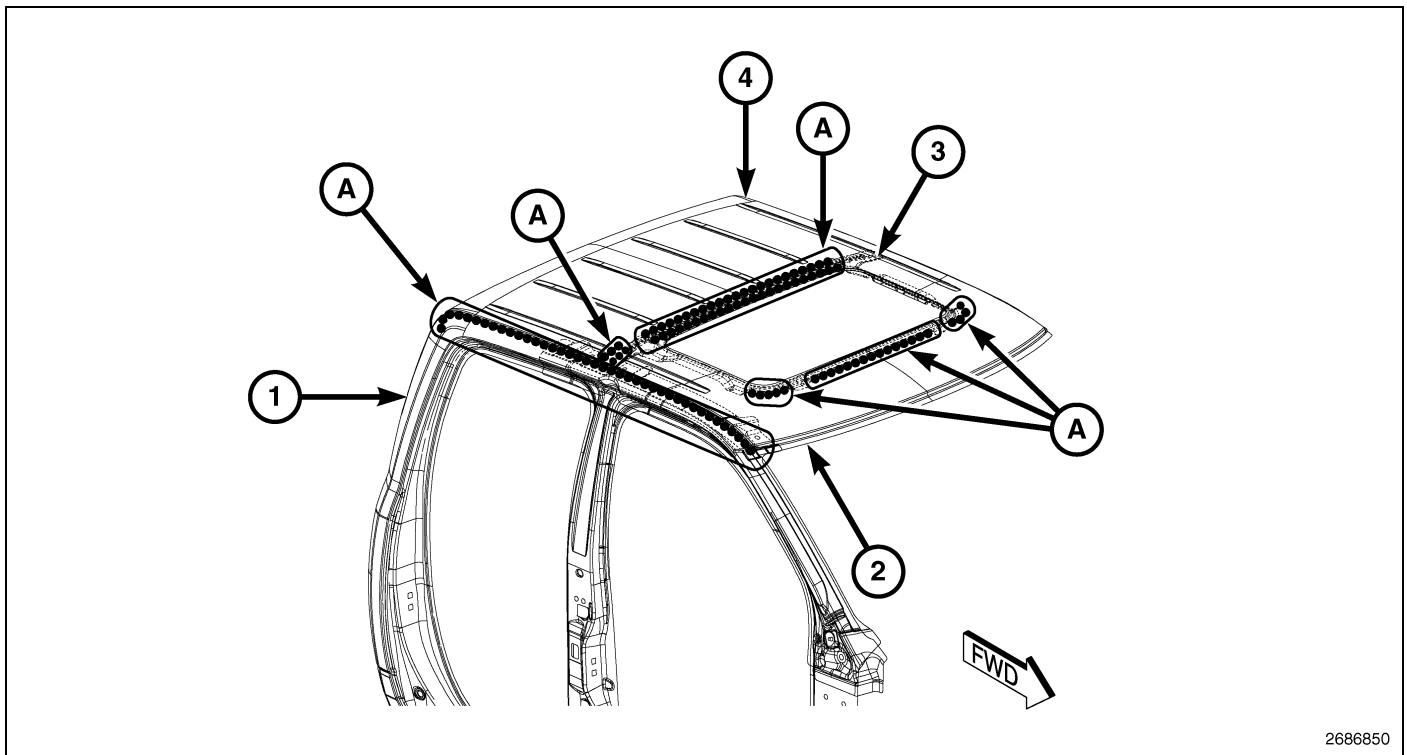
Fig. 76 Cab Complete – Quad (4 of 4)
