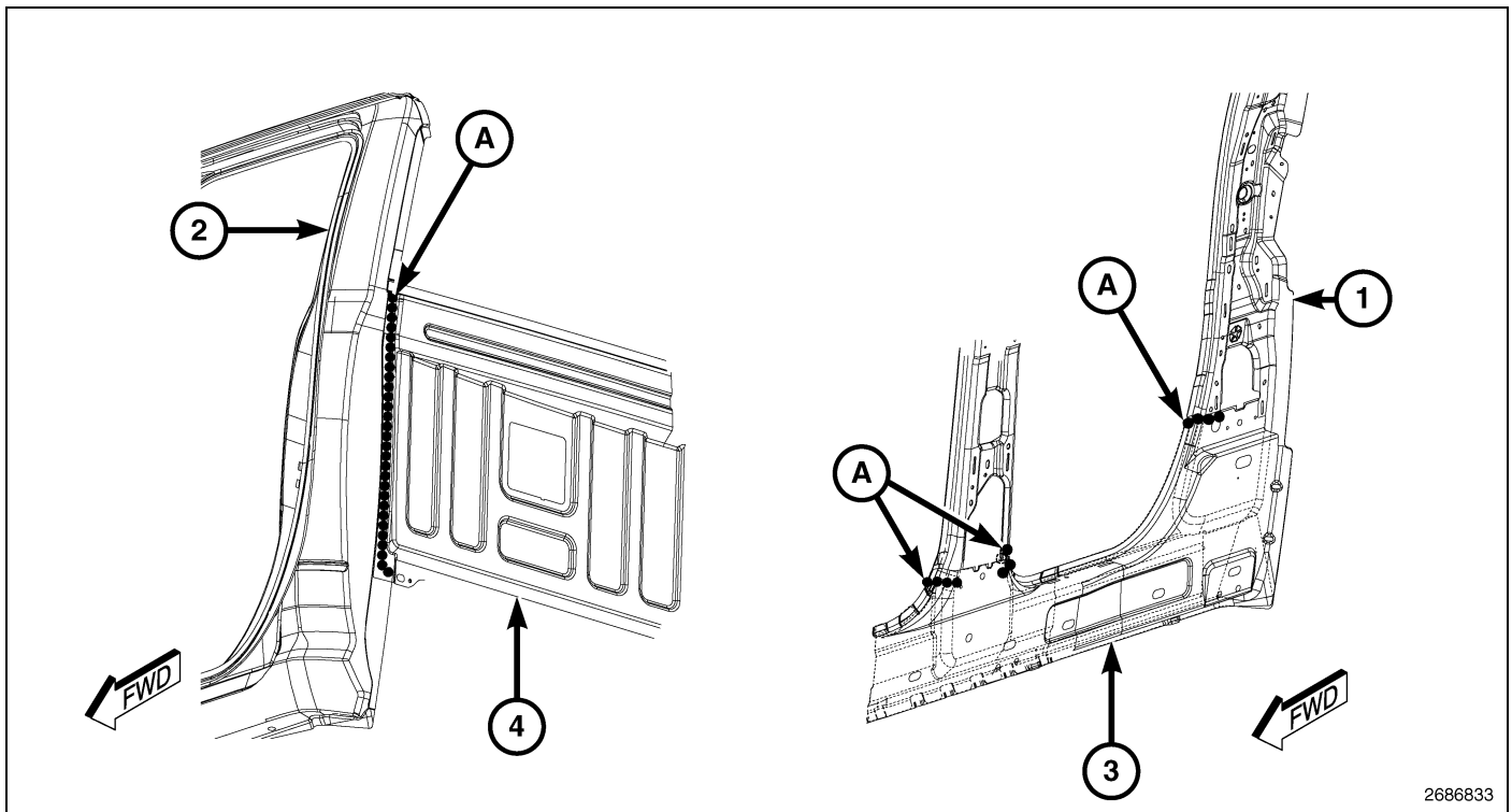
Fig. 74 Cab Complete – Quad (2 of 4)
