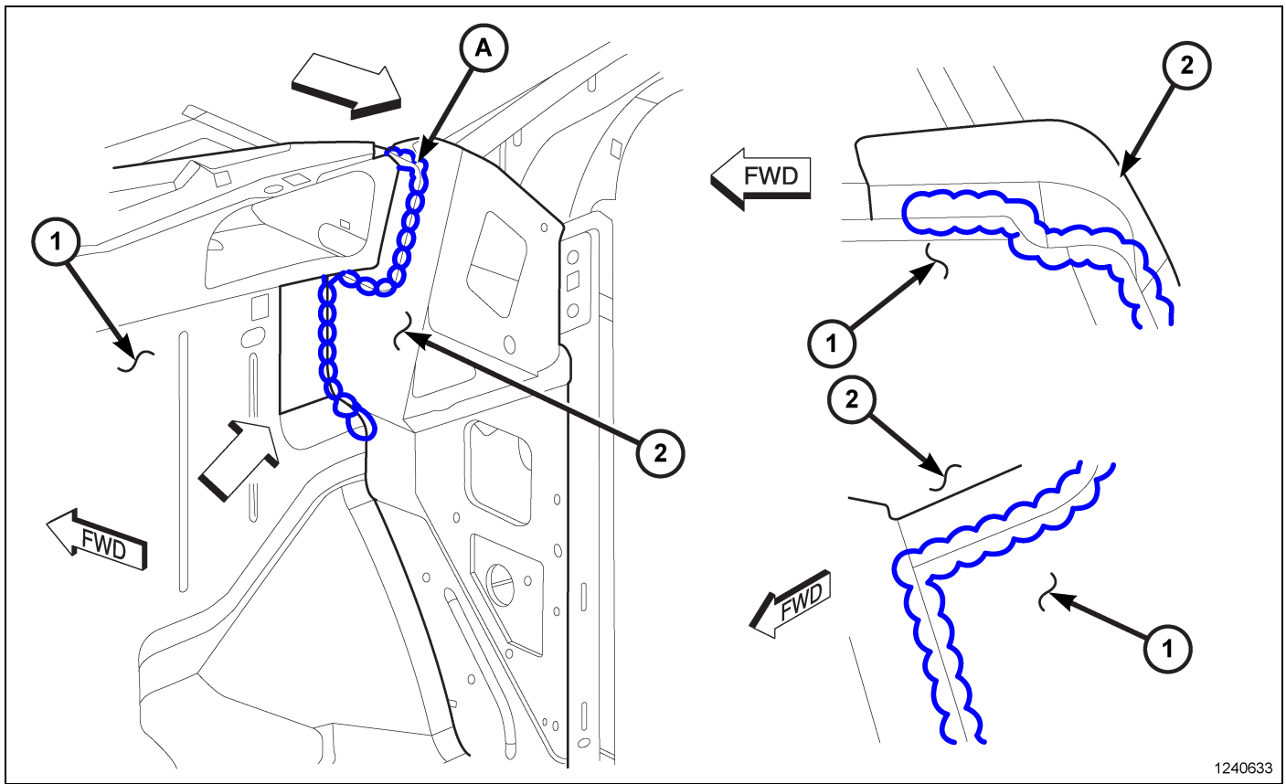
Fig. 48 Dash Panel/Cowl Side Panel (2 of 2)
