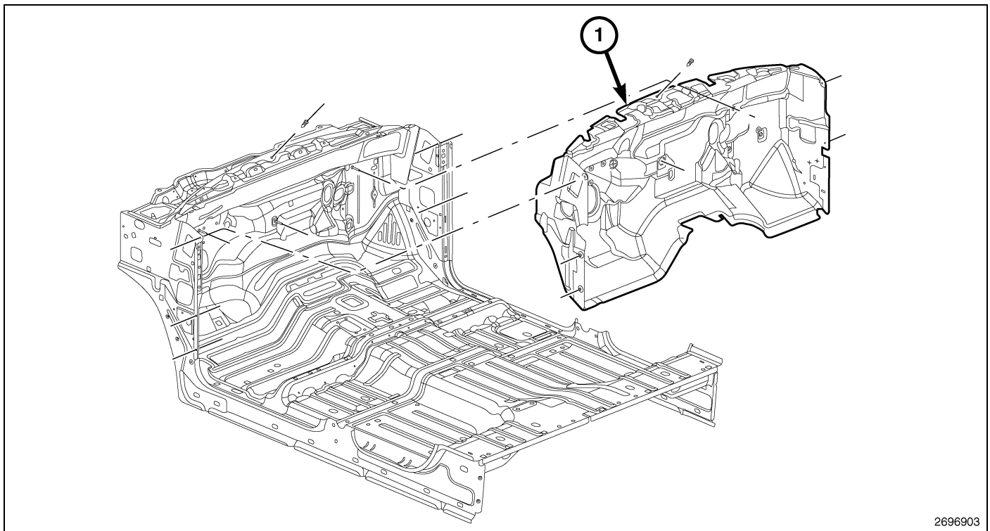
Fig. 33 DASH PANEL (2 OF 2)
