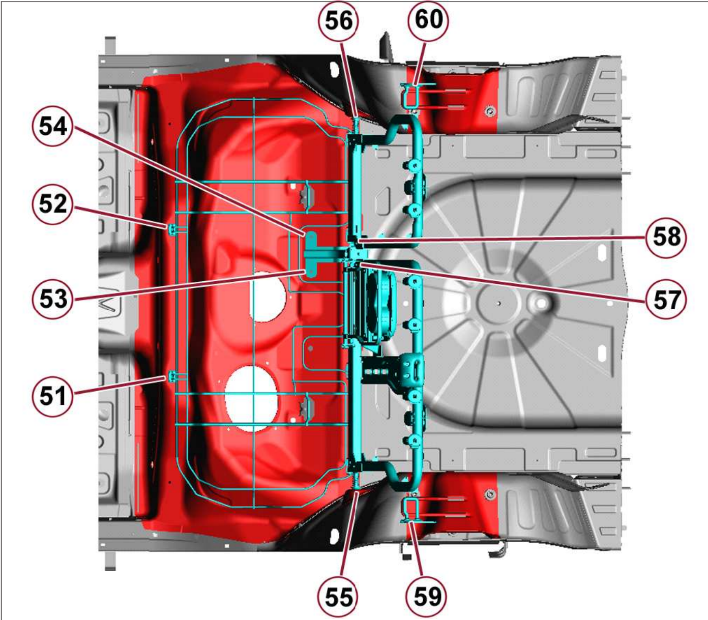
Figure 8 – Rear seat mounting
