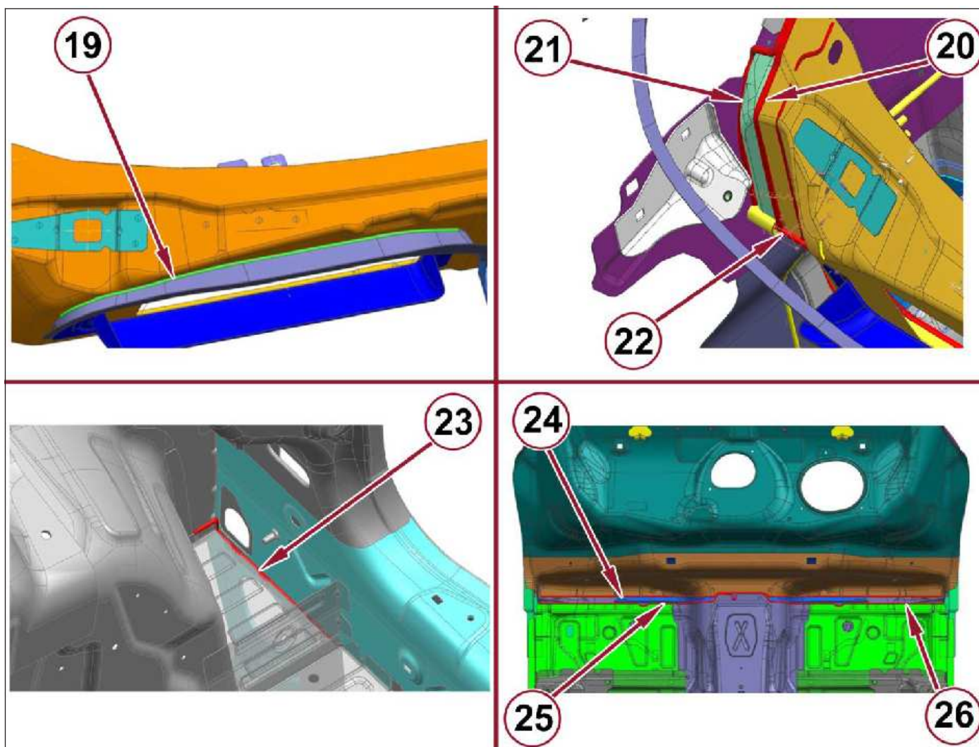
Detailed applications of sealant in areas 19 to 26
