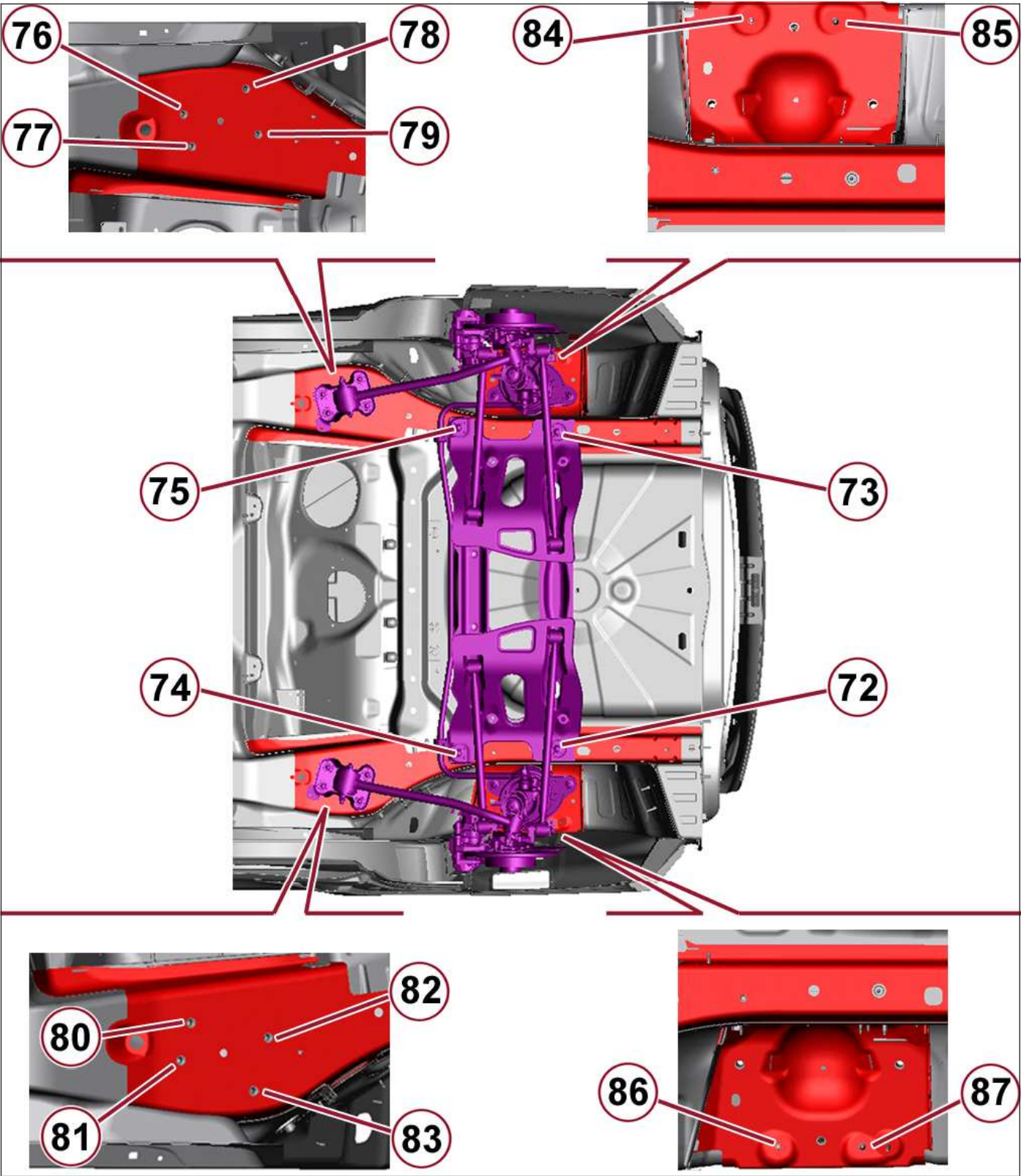
Figure 11 – Rear suspension mounting 1 of 2
