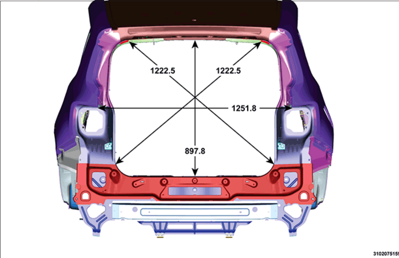
Liftgate Opening
