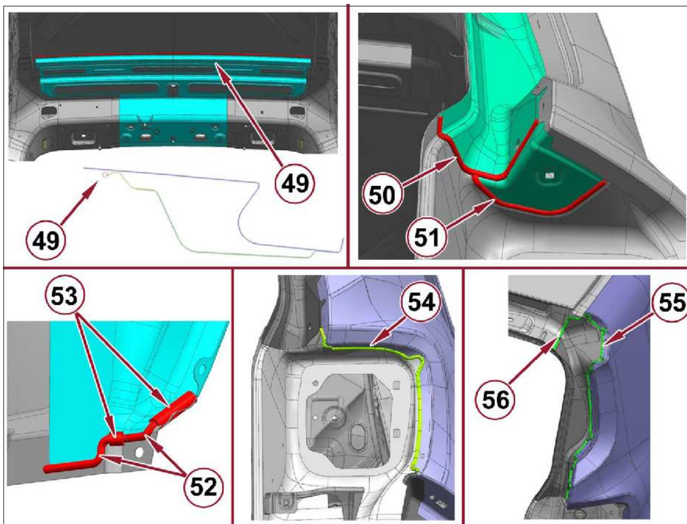
Detailed applications of sealant in areas 49 to 56
