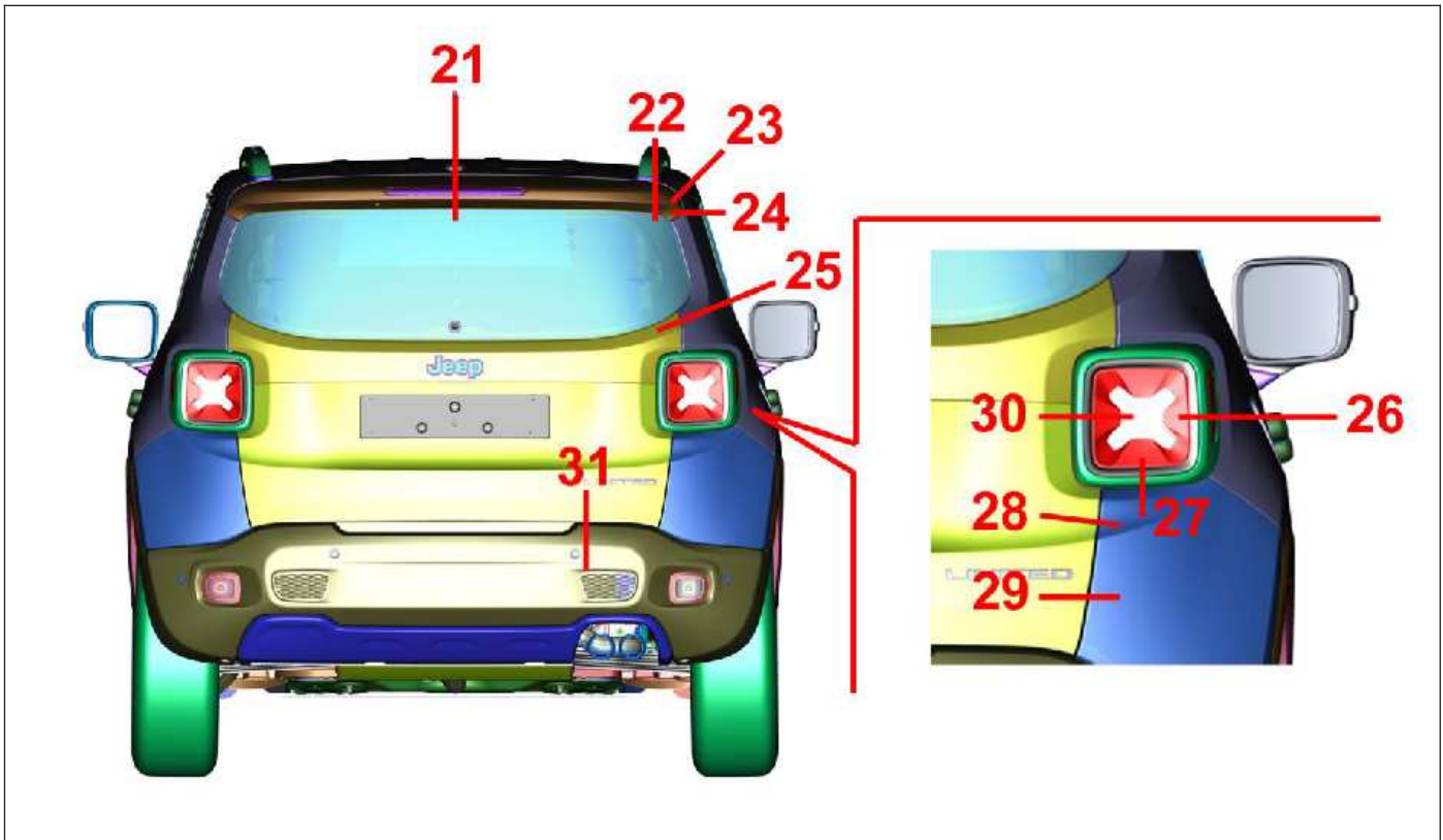
Rear view of the vehicle with measurement positions of the gaps between the moving parts
