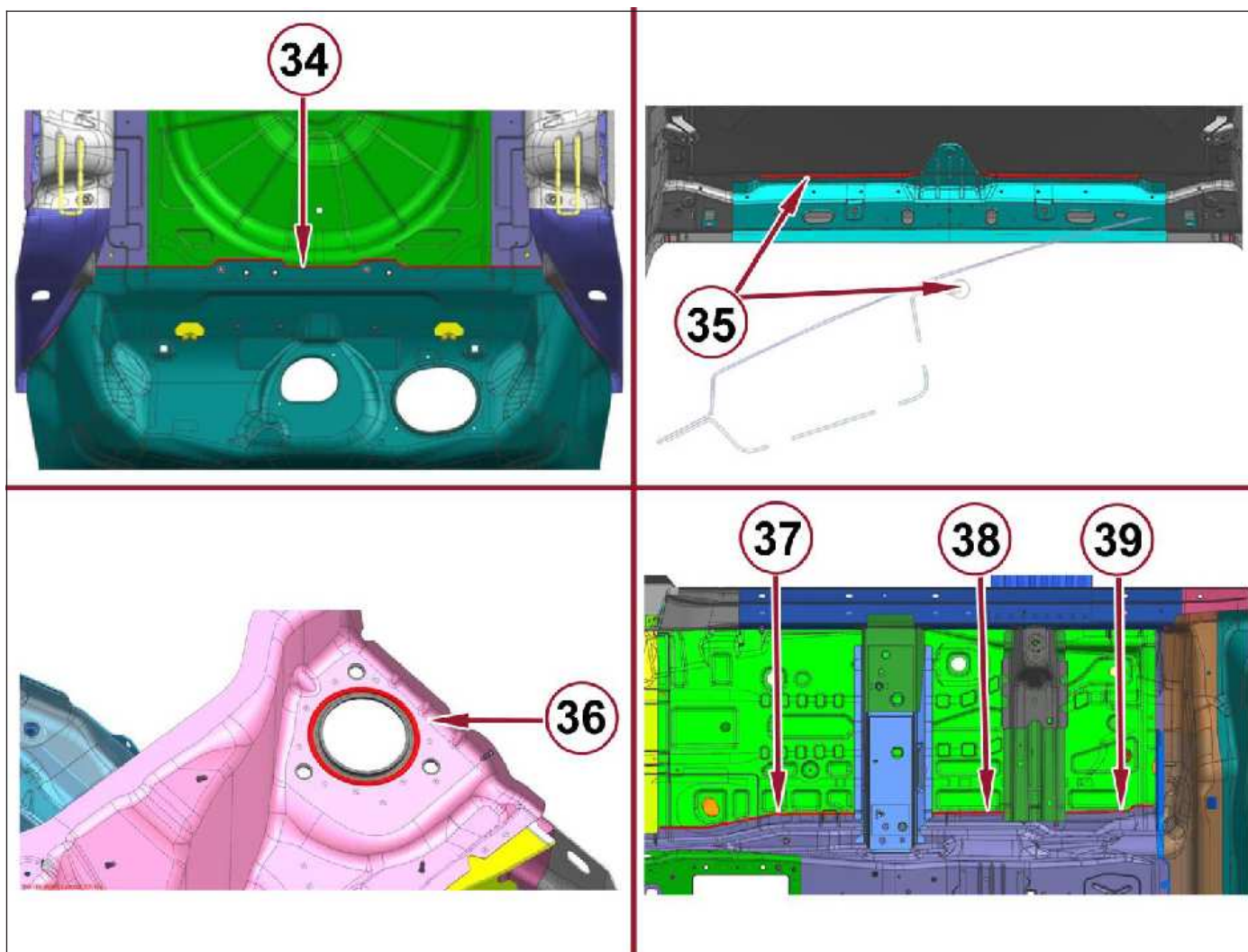
Detailed applications of sealant in areas 34 to 39
