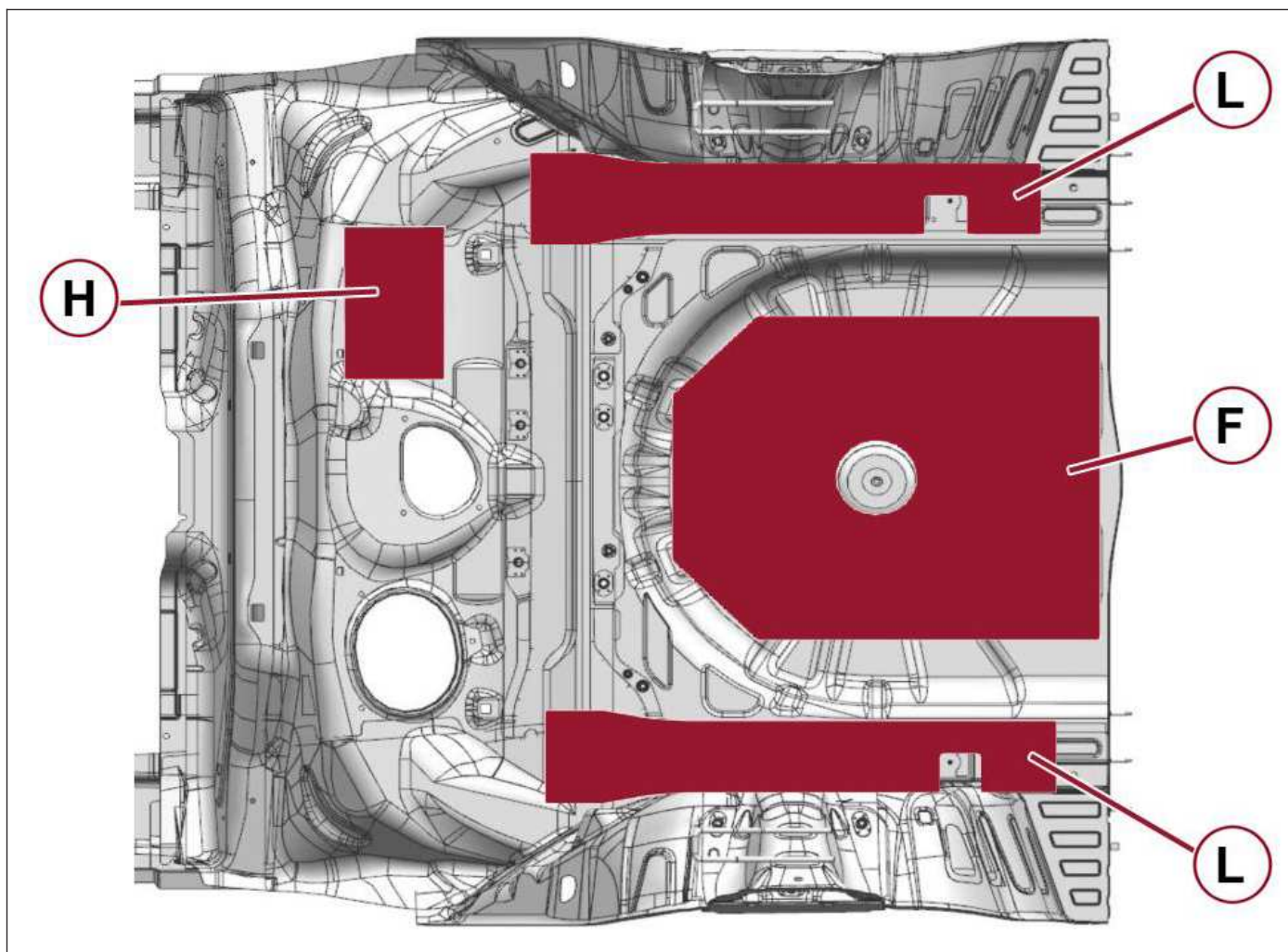
Rear Floor
