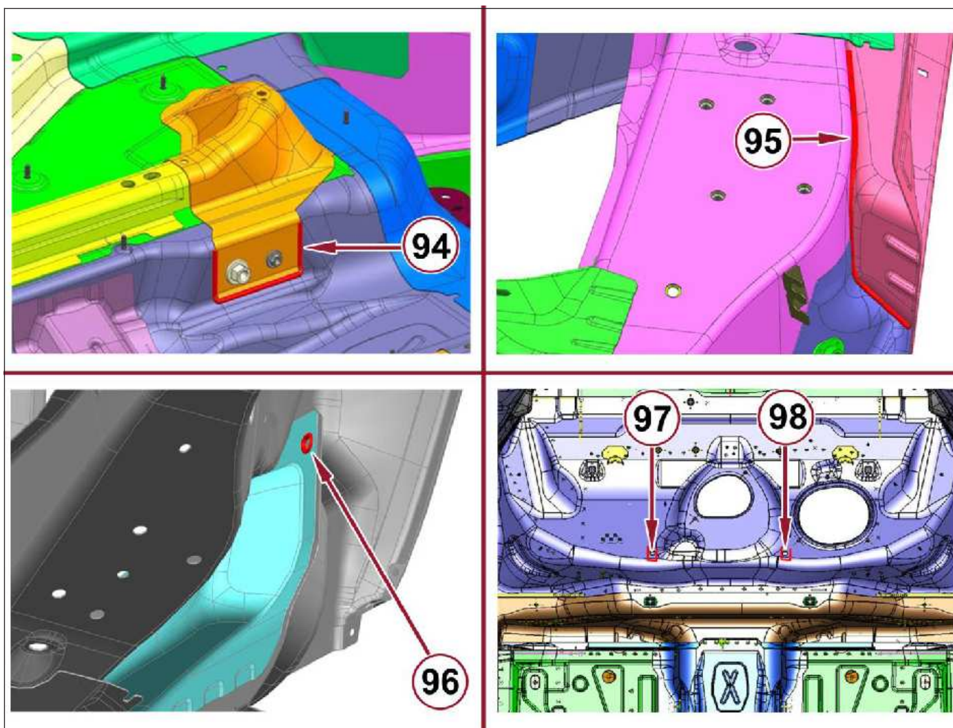
Detailed applications of sealant in areas 94 to 98
