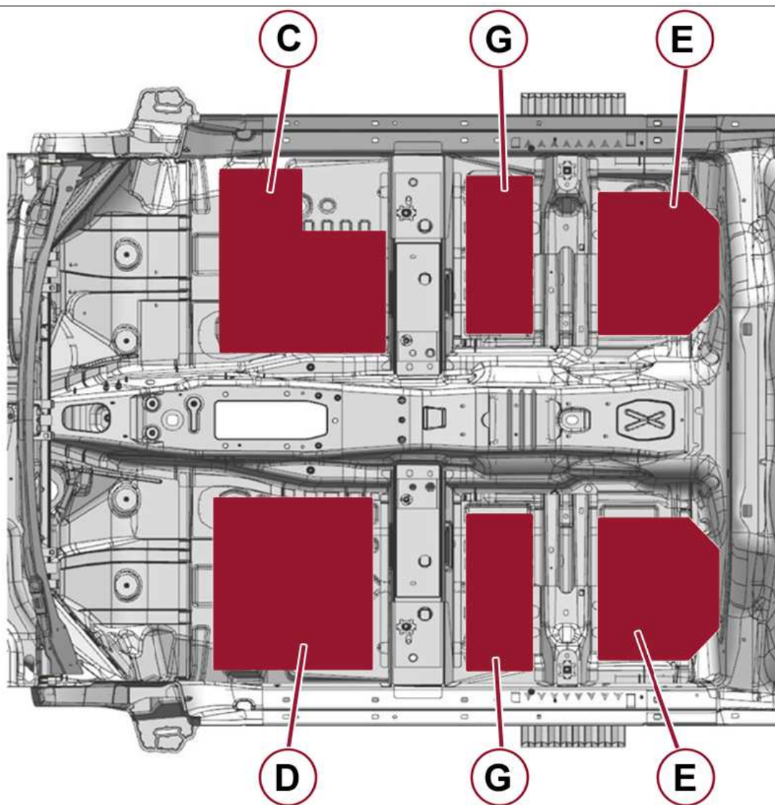
Front Floor
