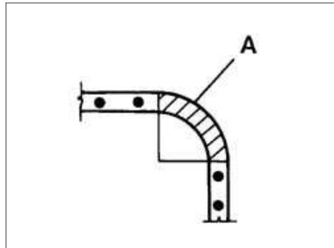
Example of correct spot welding at corners.
