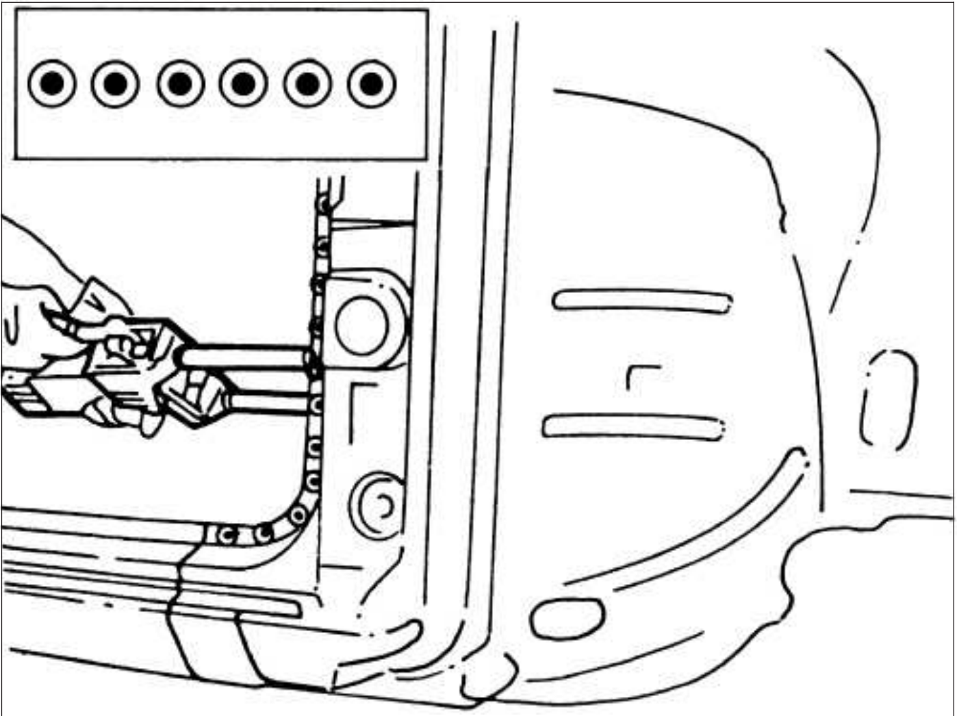
Spot welding (three panels)
