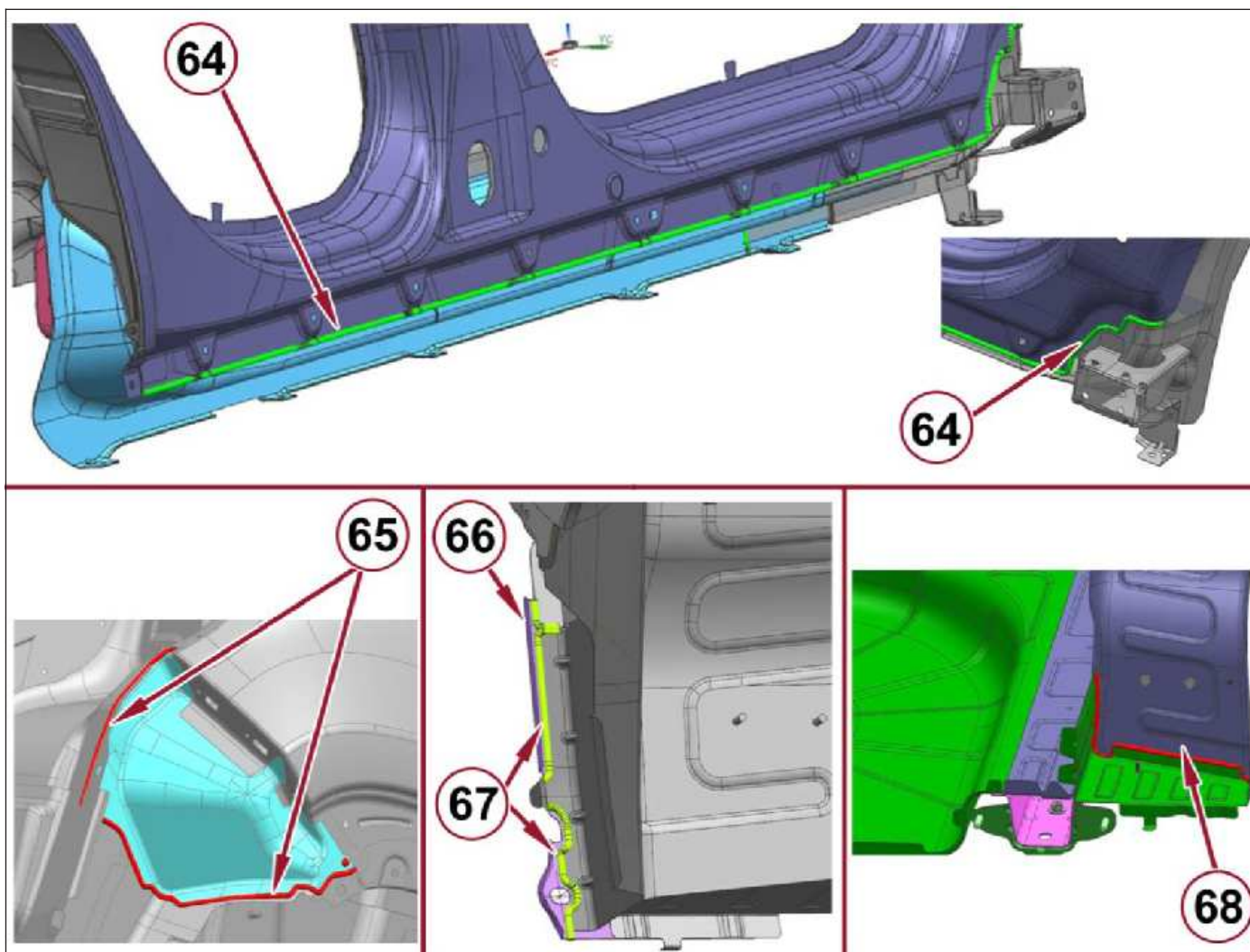
Detailed applications of sealant in areas 64 to 68
