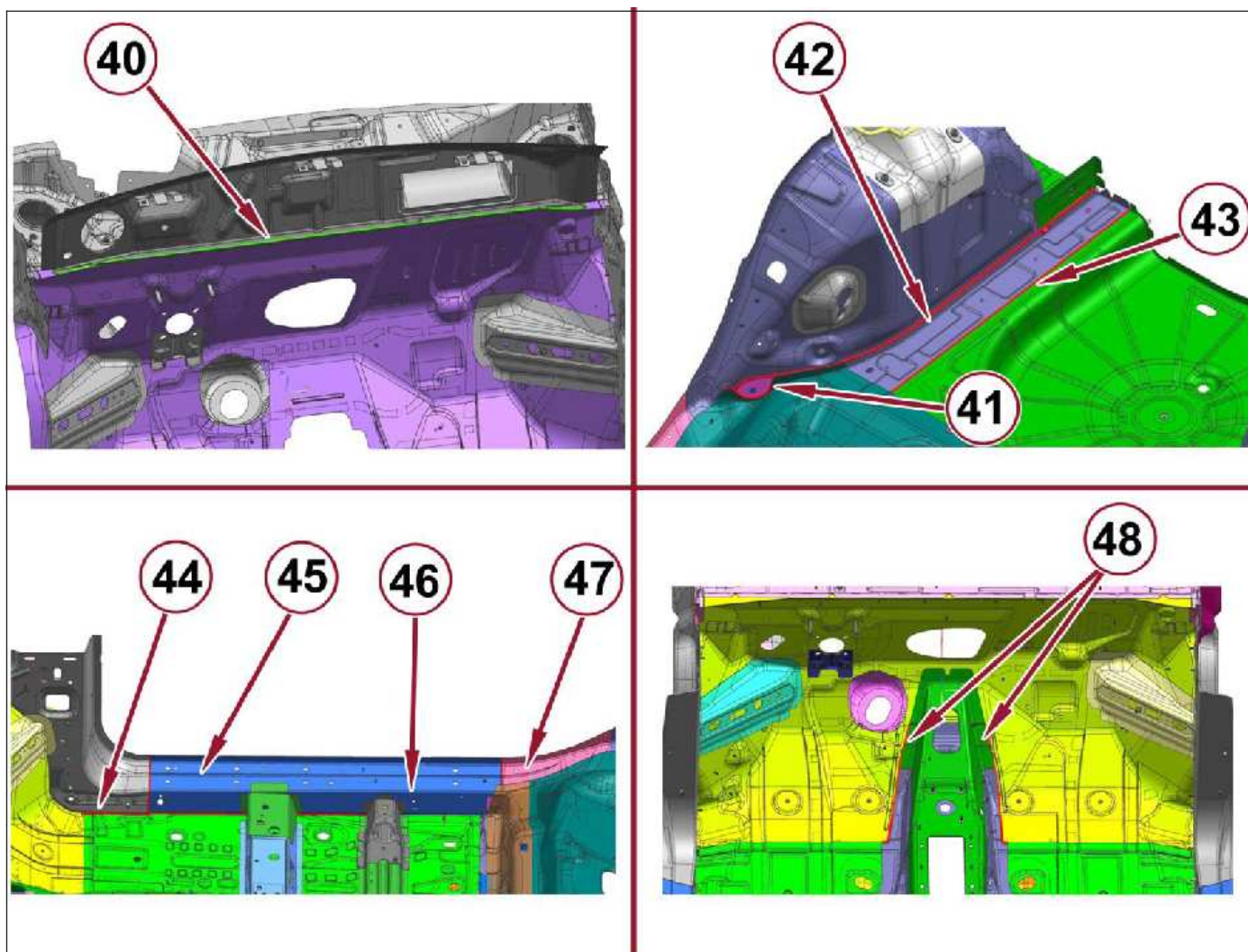
Detailed applications of sealant in areas 40 to 48
