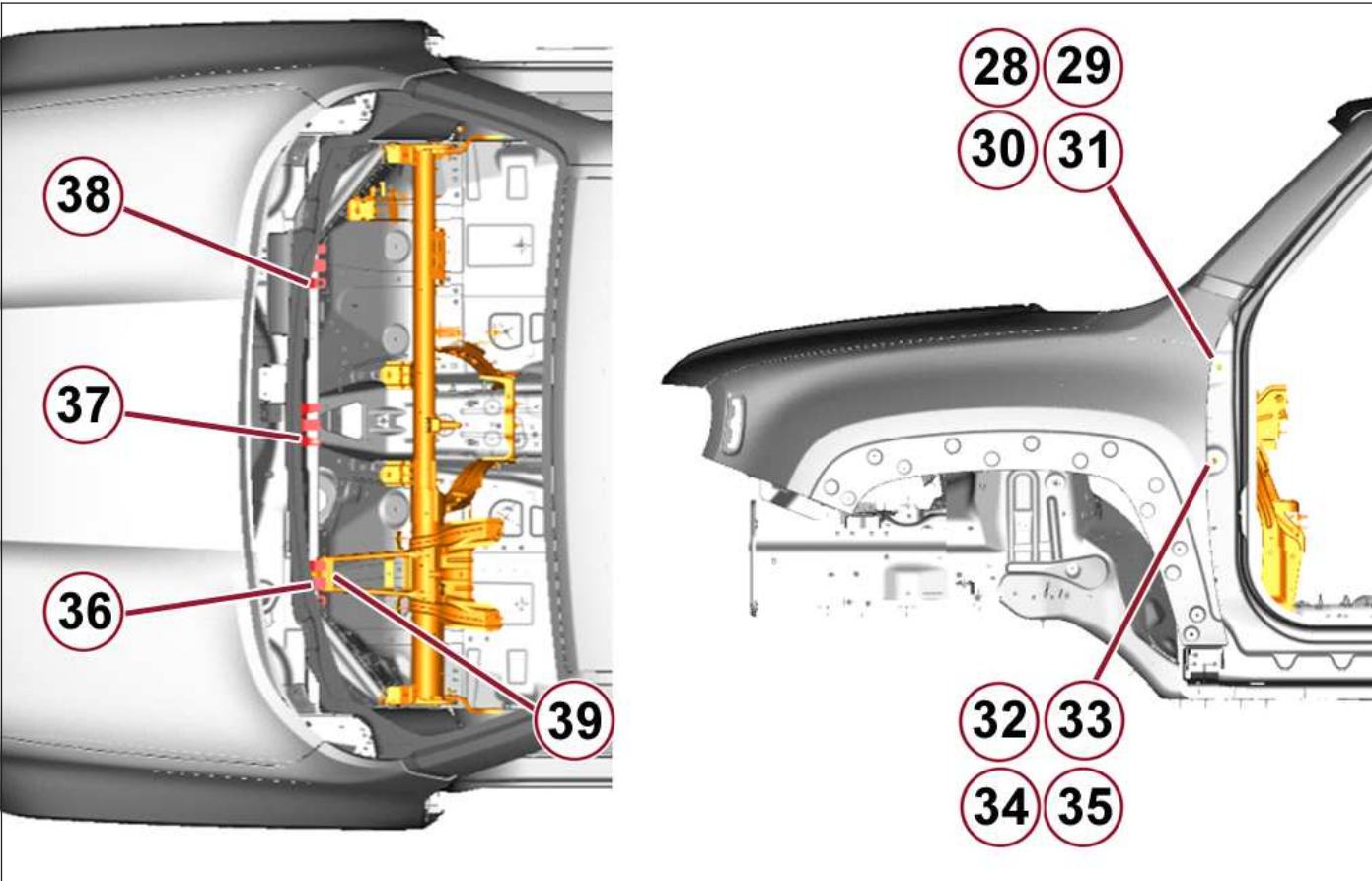
Instrument panel mounting – View 2 of 2
