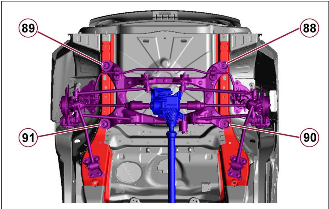
Figure 12 – Rear suspension mounting 2 of 2
