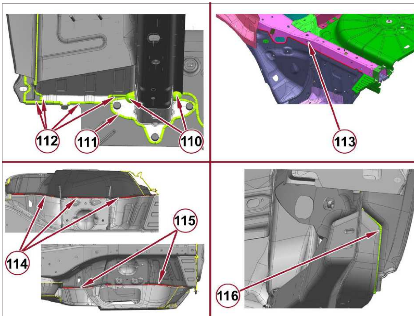
Detailed applications of sealant in areas 110 to 116
