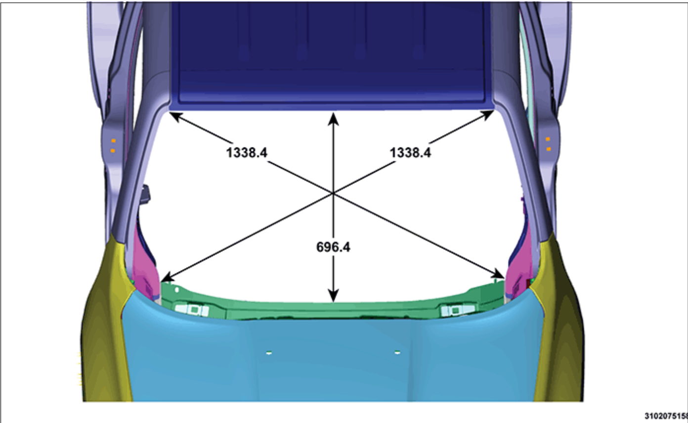
Windshield Opening
