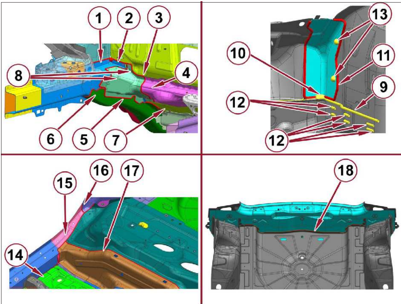
Detailed applications of sealant in areas 1 to 18
