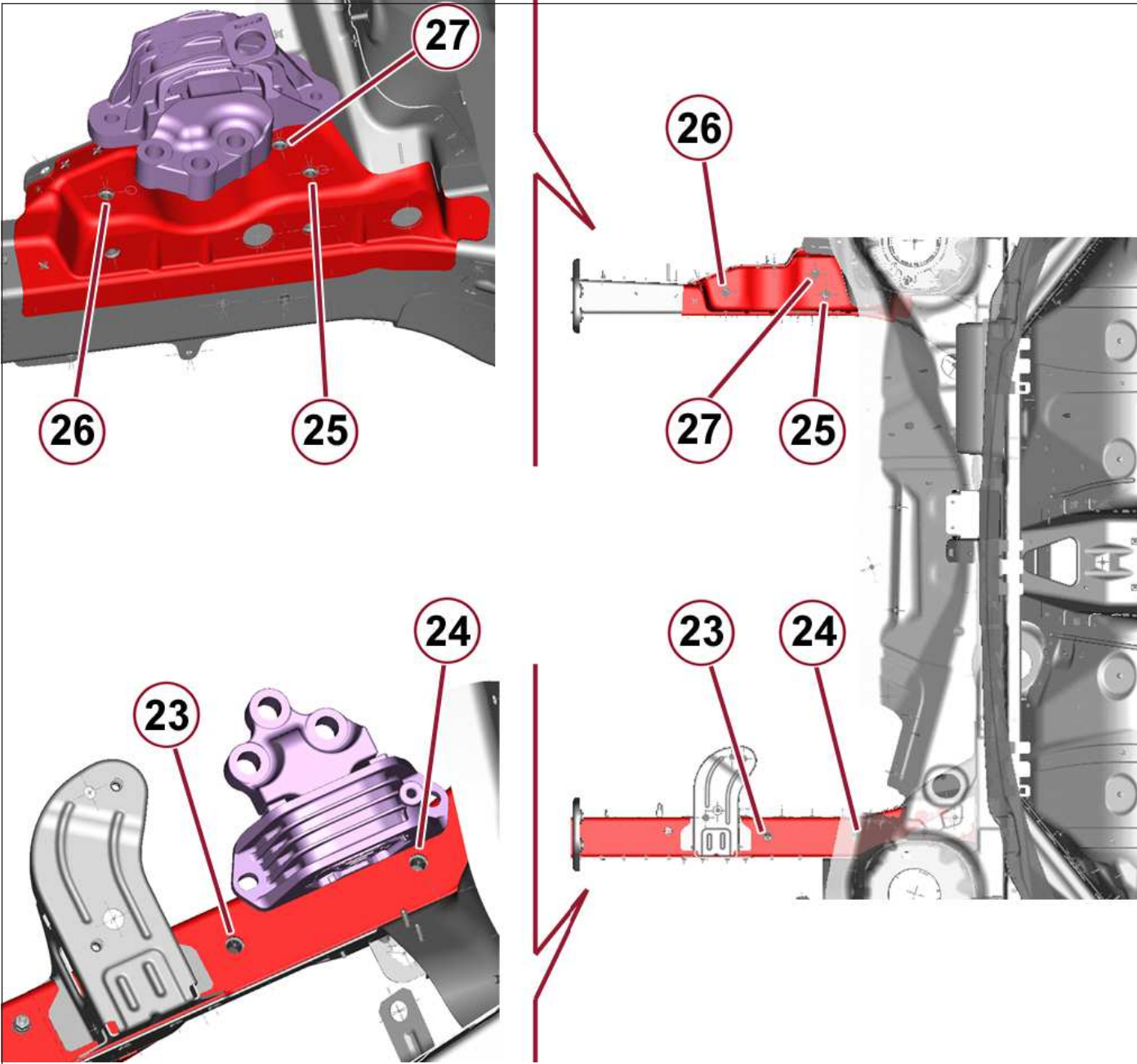
Figure 5 - Engine mounting
