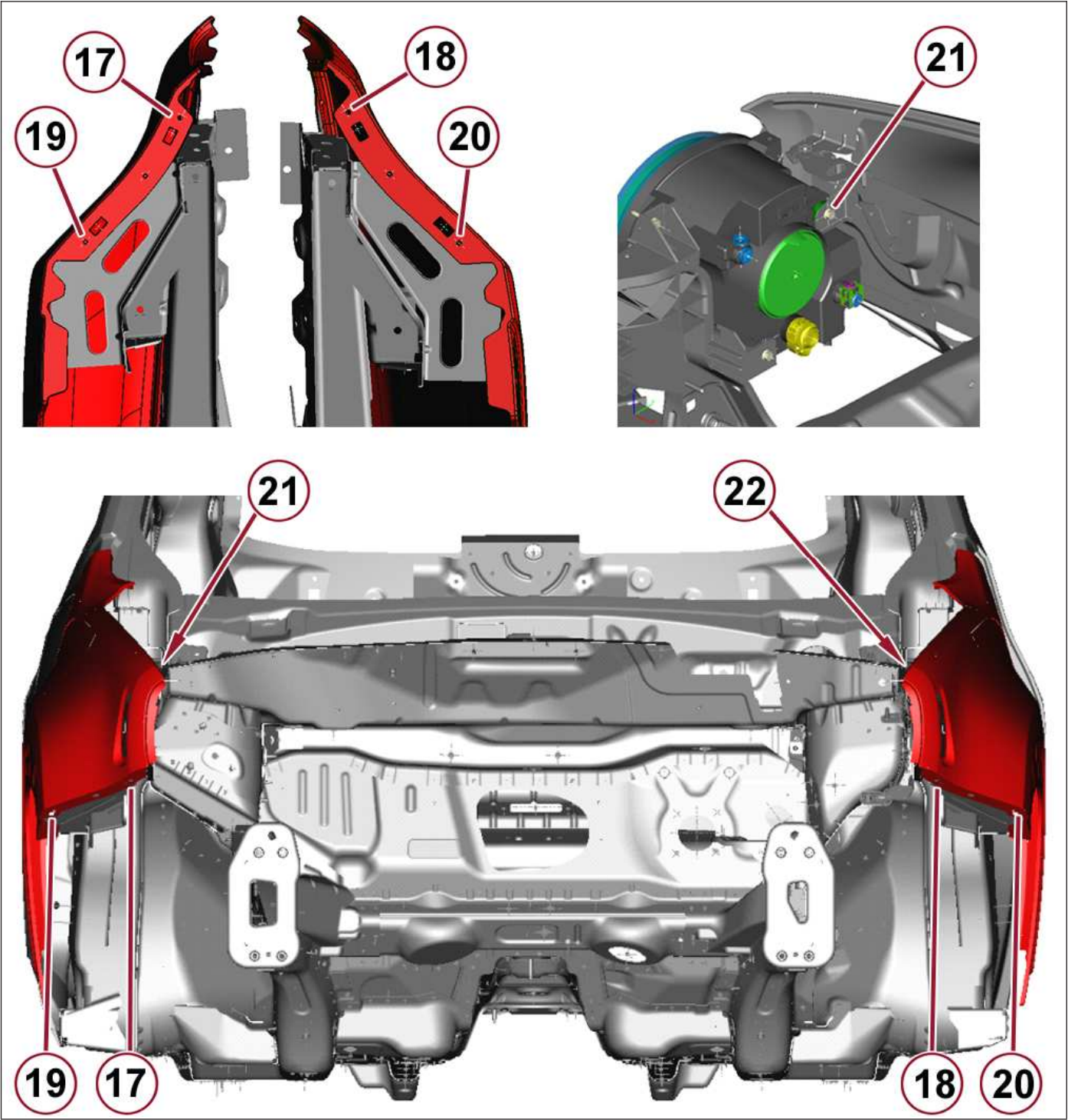
Figure 4 - Fascia mounting to fender and headlight to body
