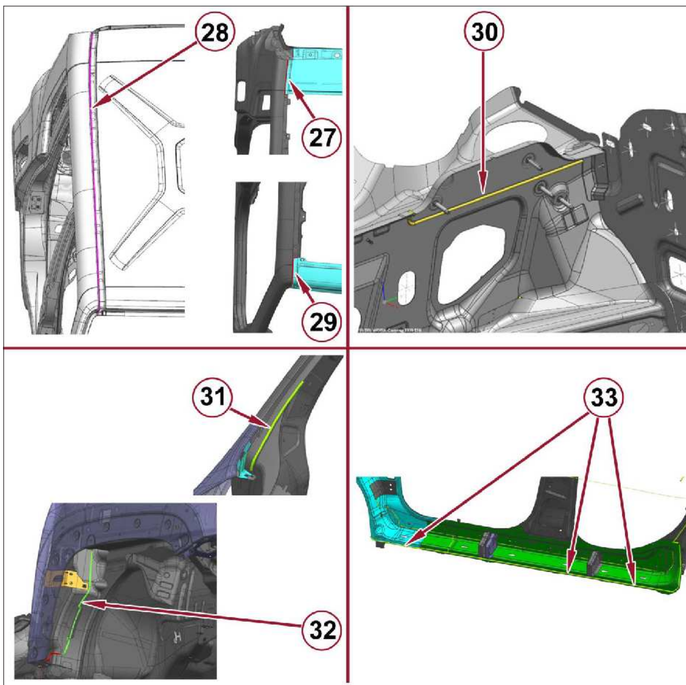
Detailed applications of sealant in areas 27 to 33
