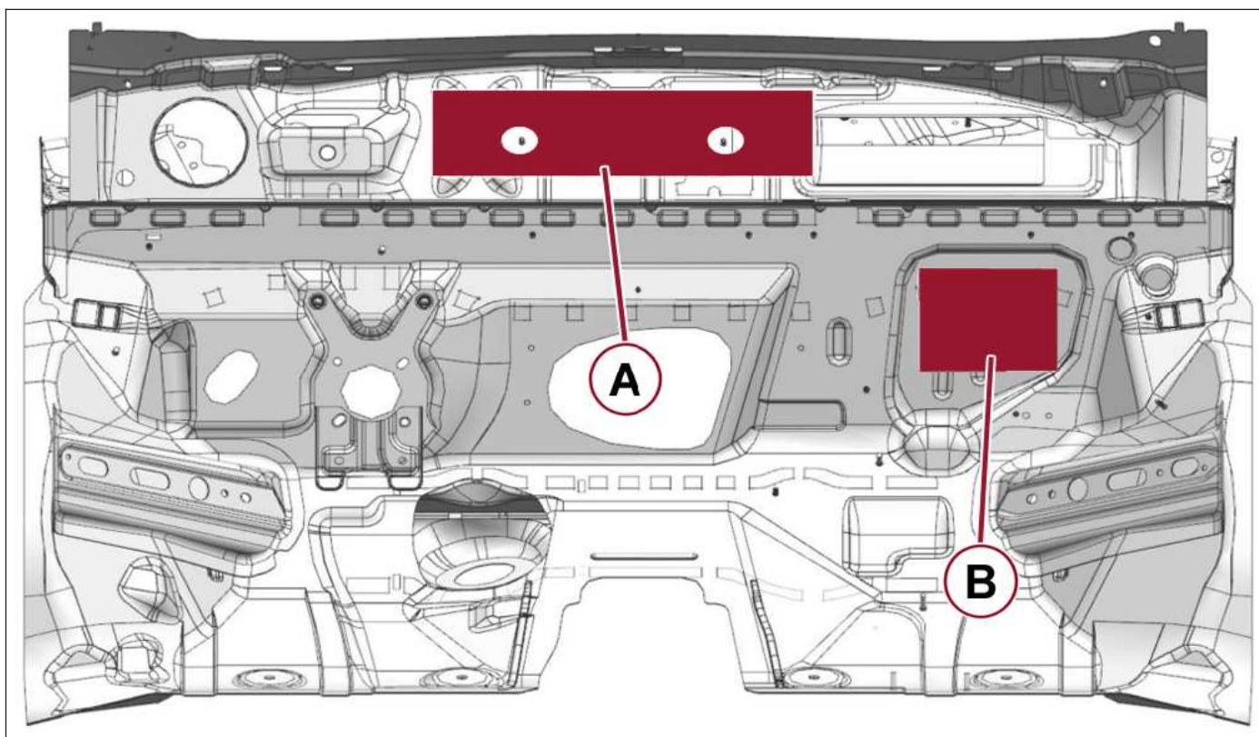
Dash Panel
