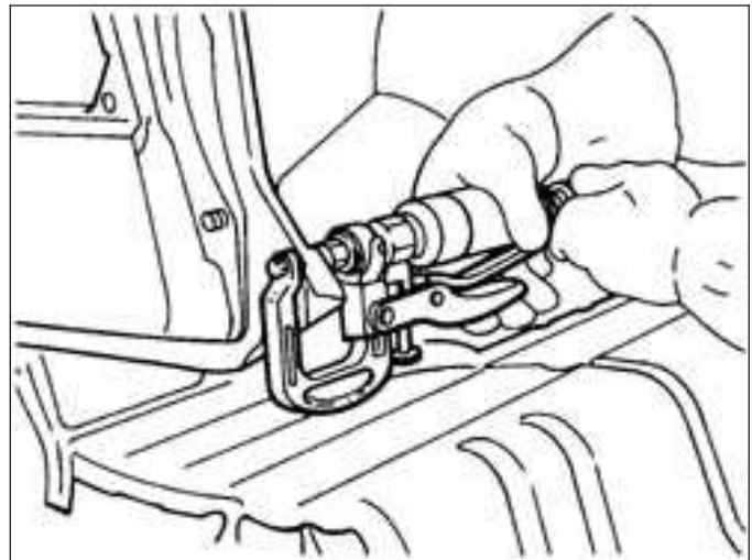
Example of the use of a milling machine.
