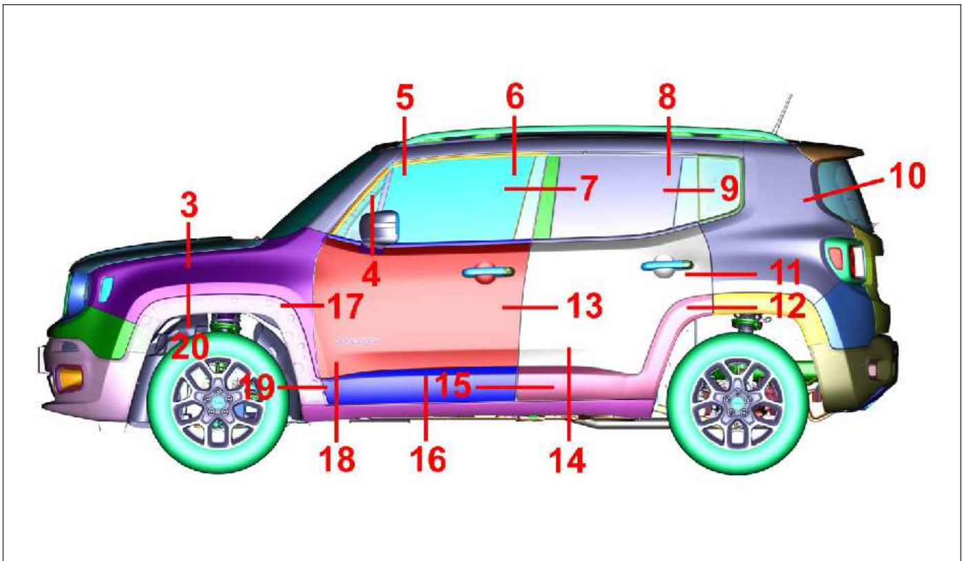
Side view of the vehicle with measurement positions of the gaps between the moving parts
