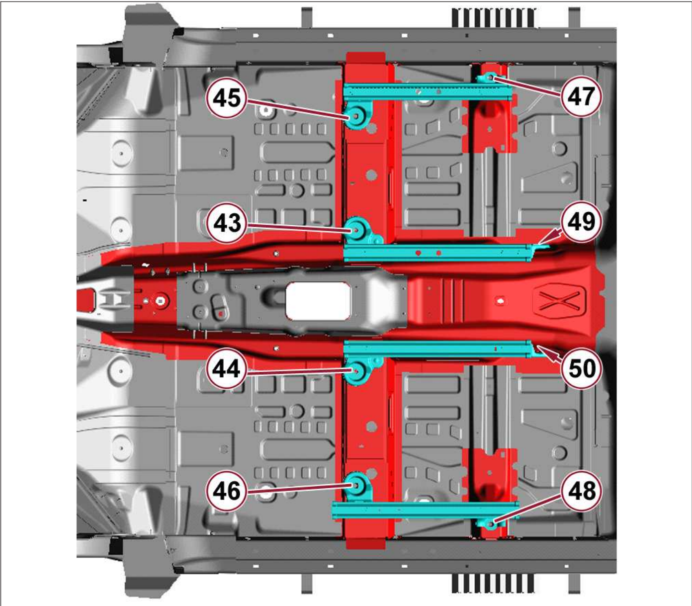
Figure 7 – Front seat mounting
