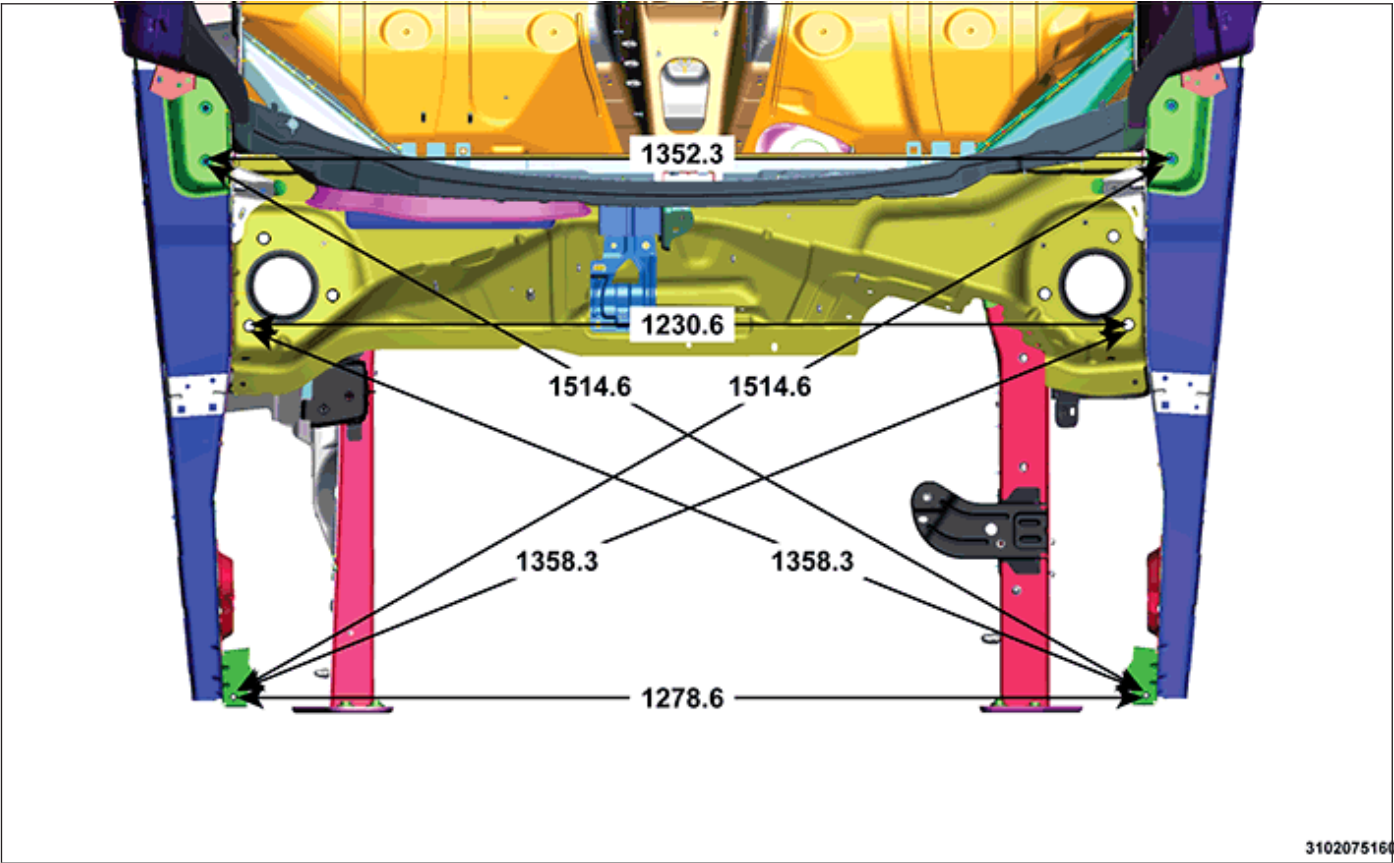
Figure 13 – Under Hood Dimensions
