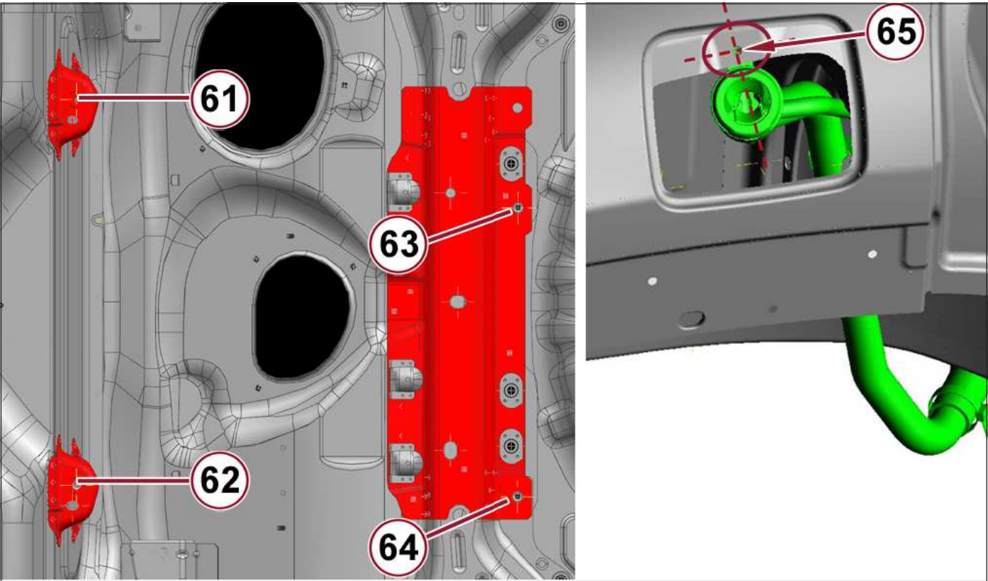
Figure 9 – Fuel tank mounting
