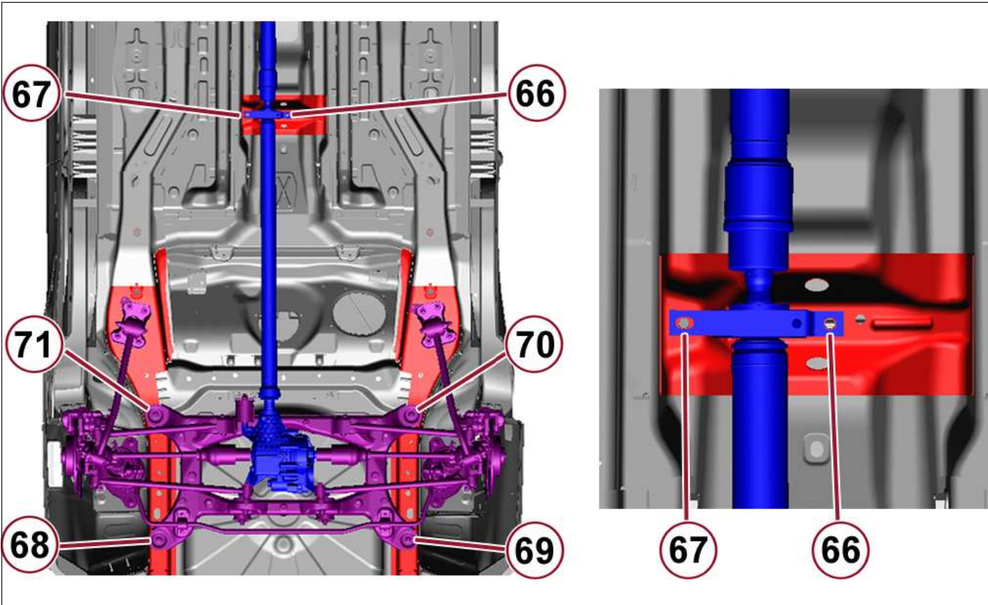
Figure 10 – Rear drive components mounting
