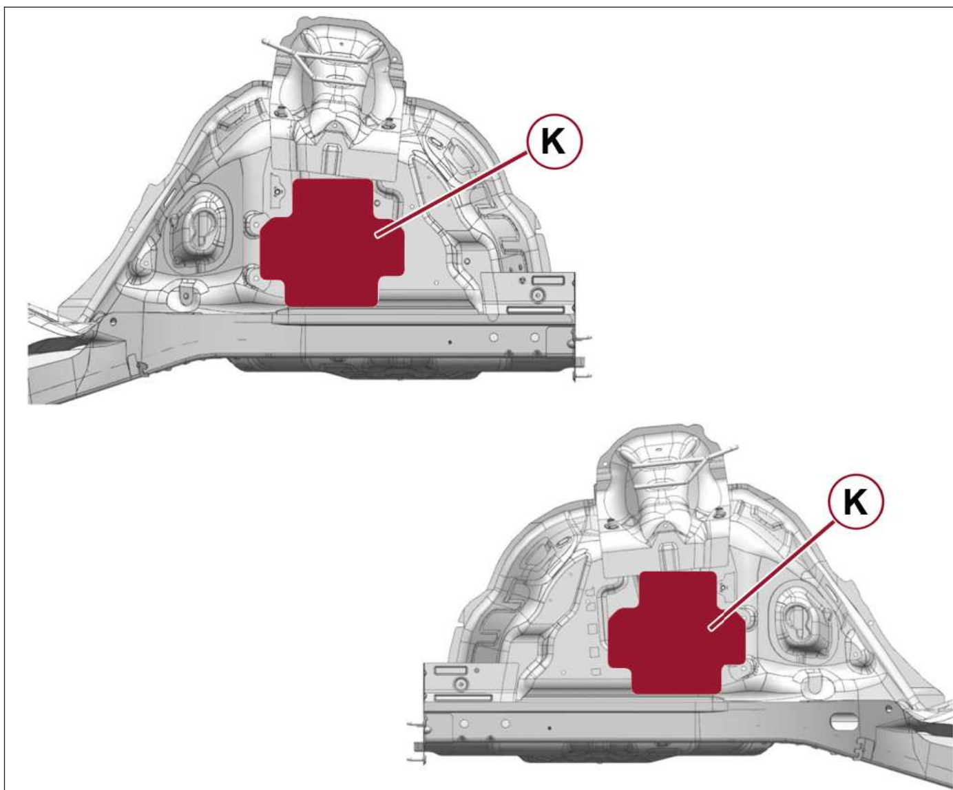
Rear Inner Wheelhouse
