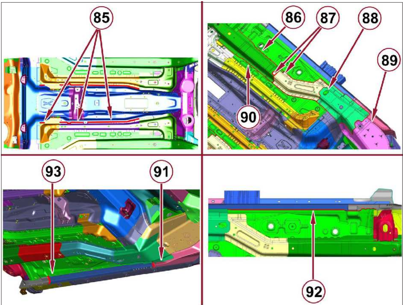
Detailed applications of sealant in areas 85 to 93
