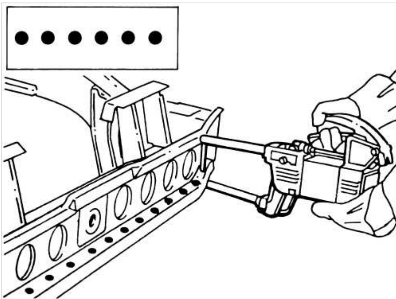
Spot welding
