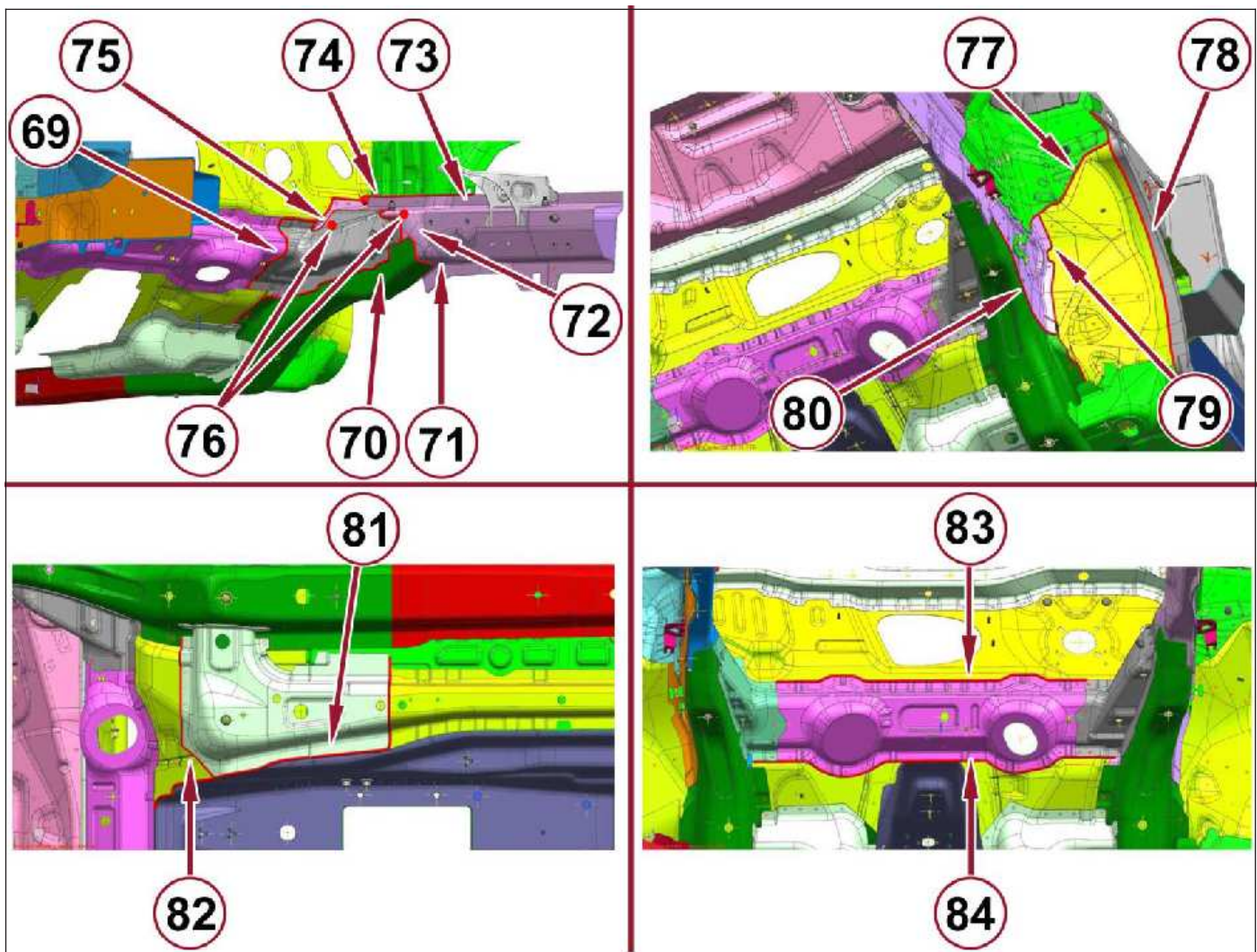
Detailed applications of sealant in areas 69 to 84
