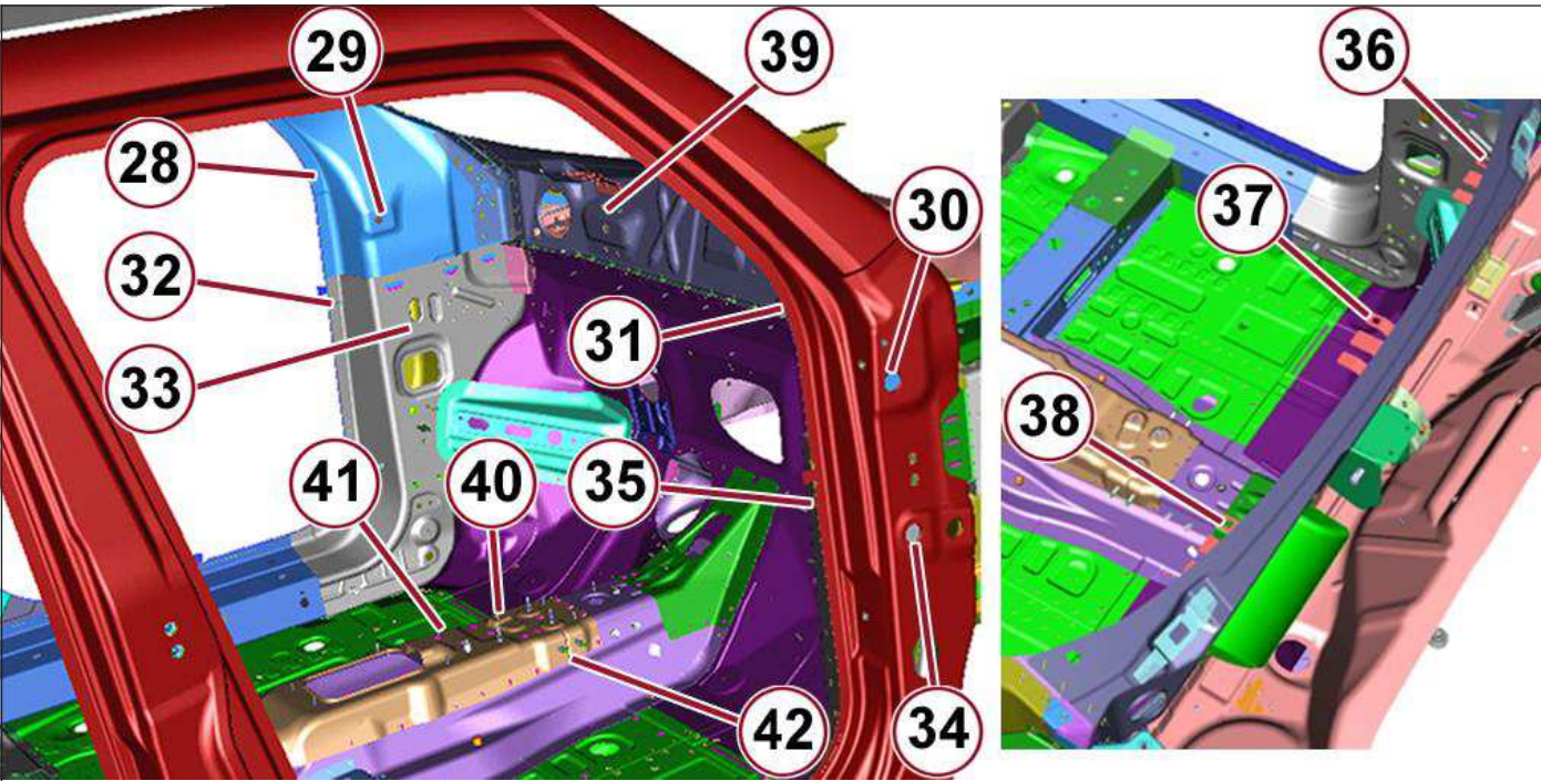
Figure 6 - Instrument panel mounting – View 1 of 2
