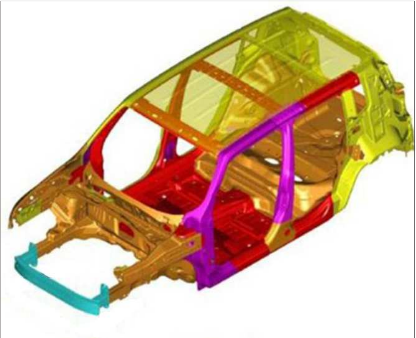
Material used for vehicle body
