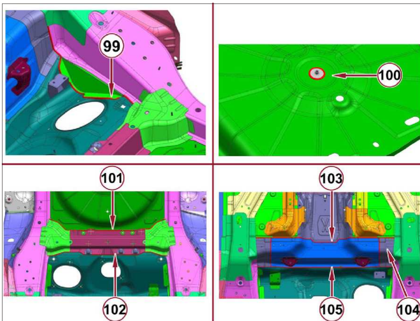
Detailed applications of sealant in areas 99 to 105
