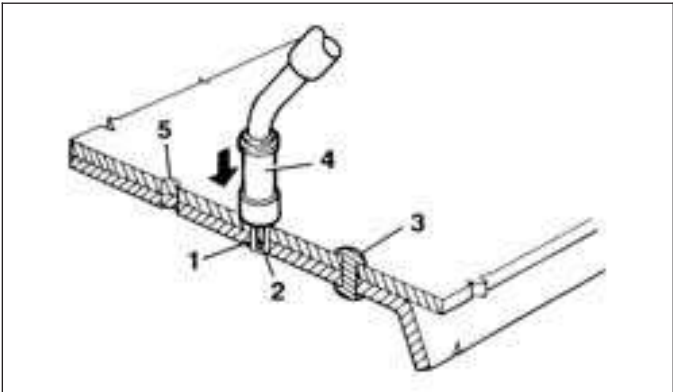
Carrying out welding using an inert gas electrode (MIG) to join overlapping.
