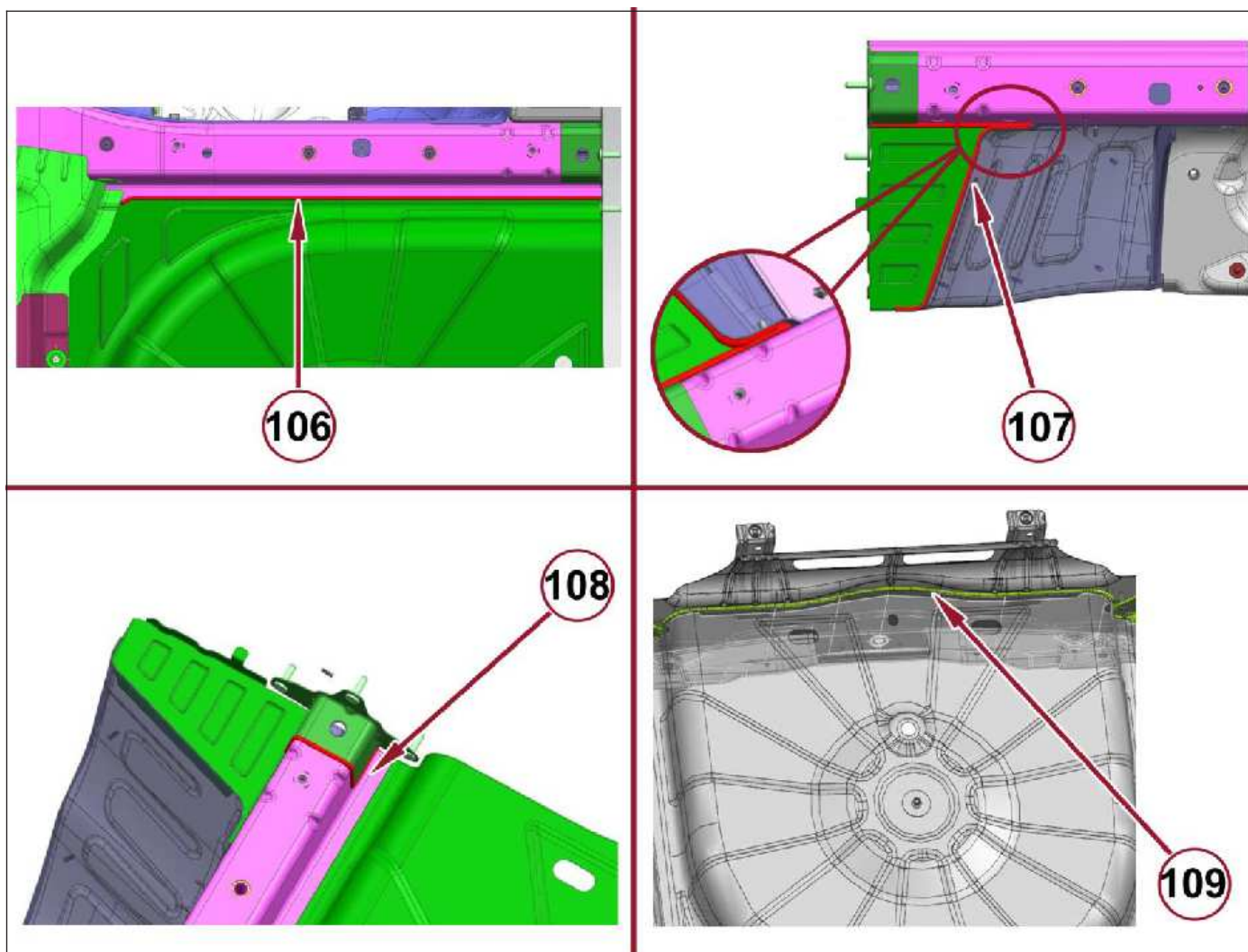
Detailed applications of sealant in areas 106 to 109
