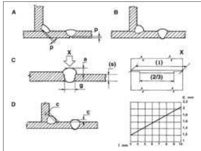
Examples of welding.
