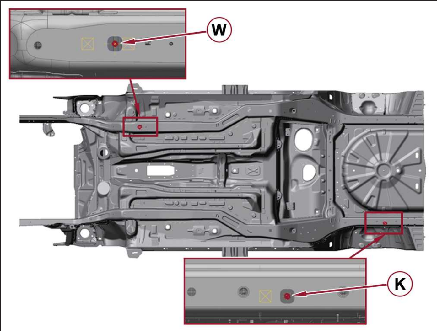
Figure 1 - Reference Point Identification
