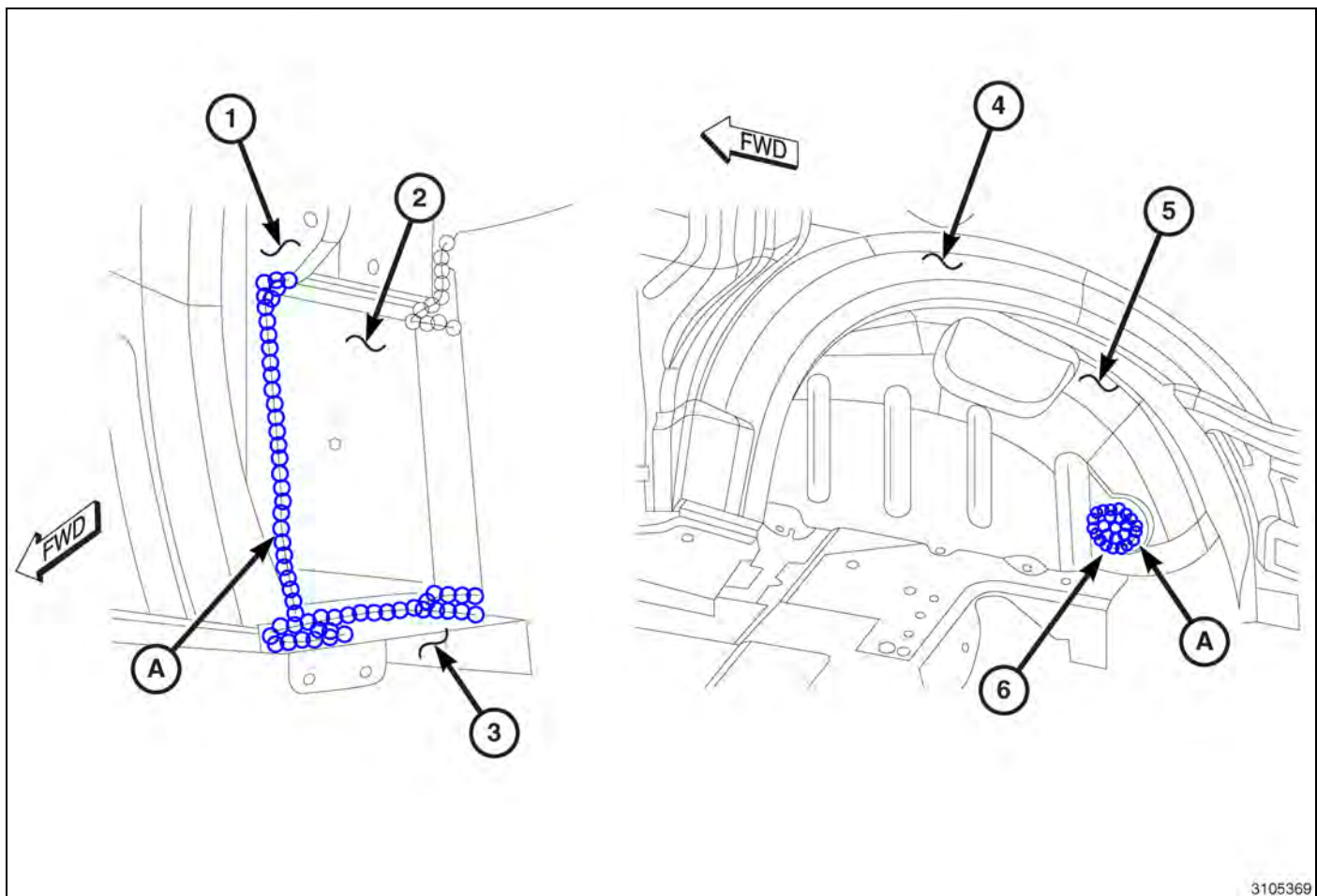
Fig. 43 Outer Wheelhouse / Inner Quarter Rear Jack Reinforcement (1 of 2)
