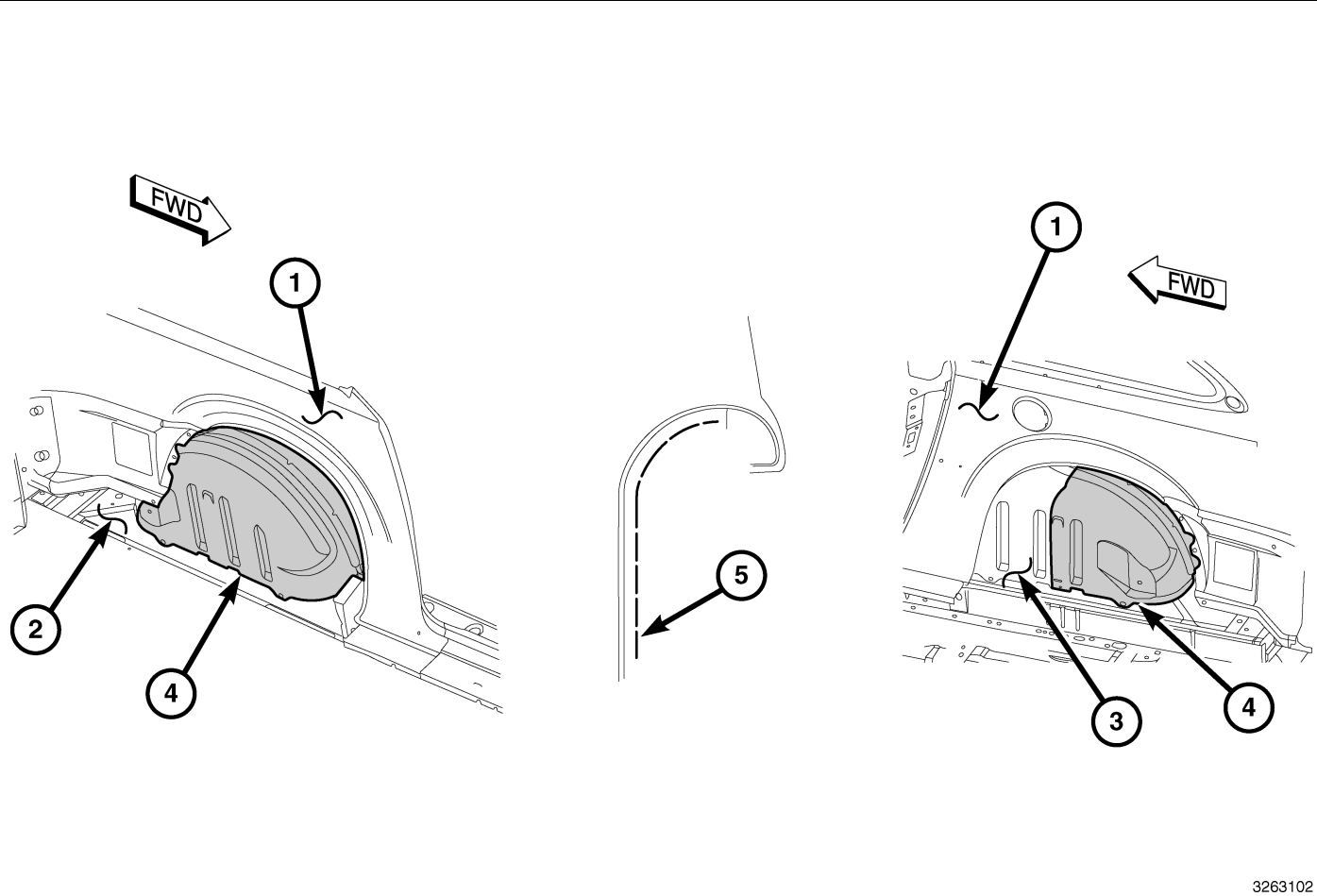
Fig. 30 REAR WHEELHOUSES
