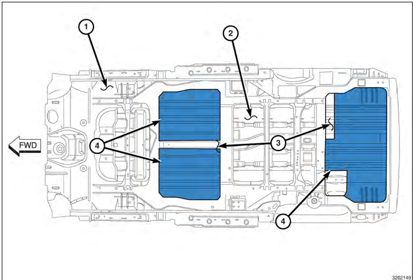
Fig. 26 SEAT TUBS
