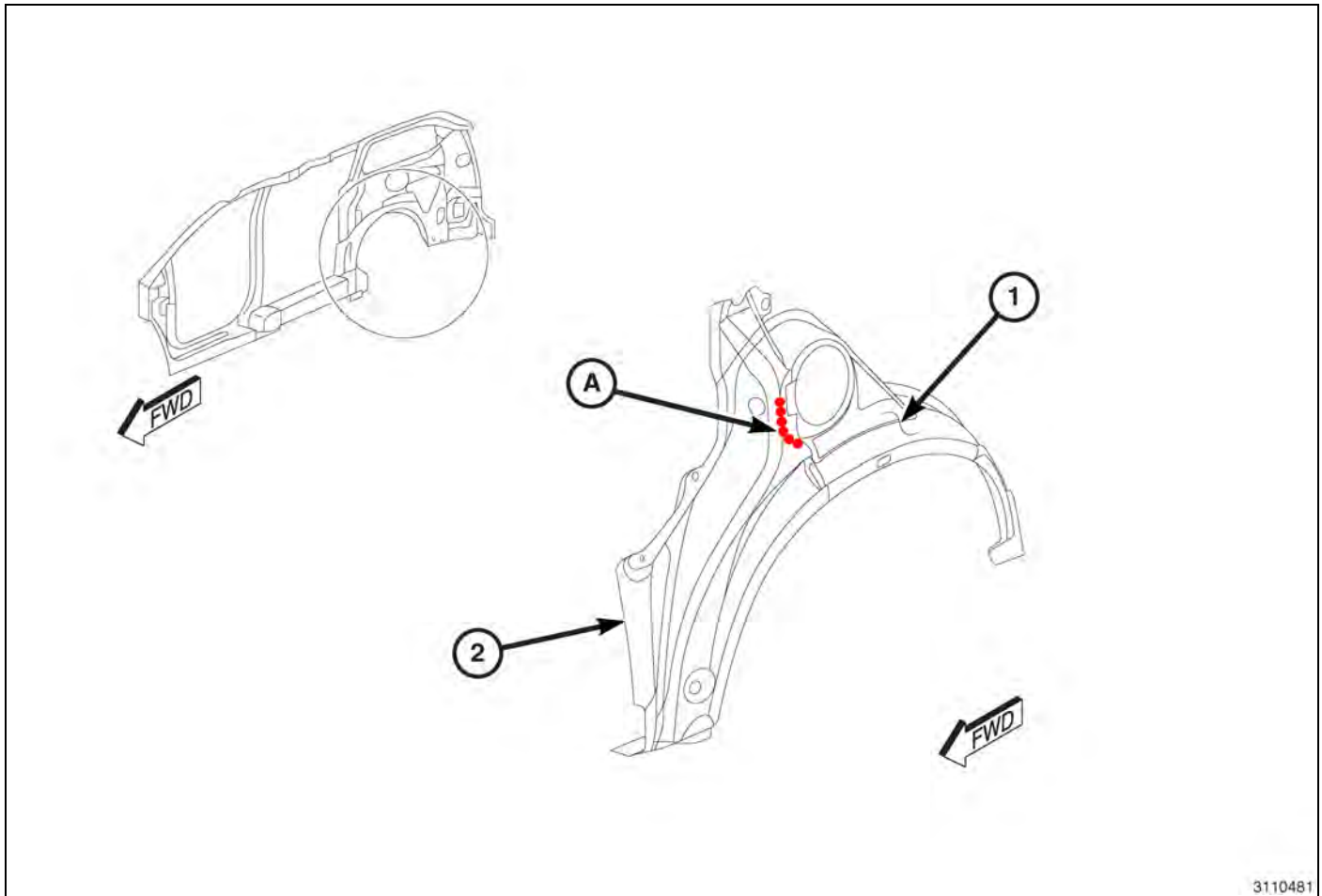
Fig. 63 BODY SIDE APERTURE - INNER (2 of 2)
