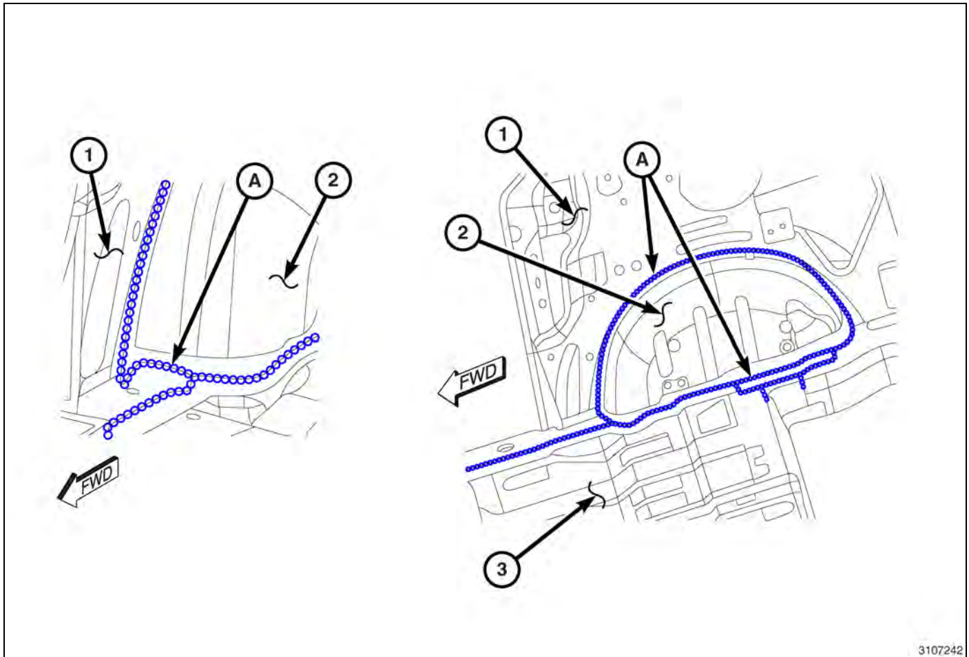
Fig. 46 Rear Wheelhouse Body / Side Aperture Inner Panel (2 of 2)
