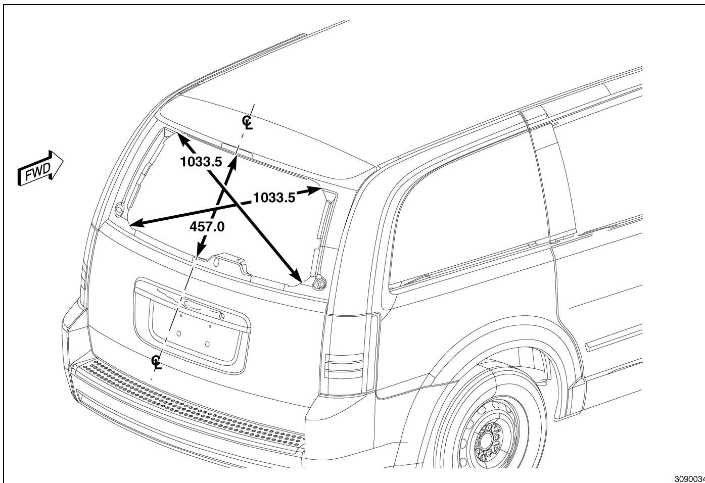
Fig. 4 Liftgate Glass
