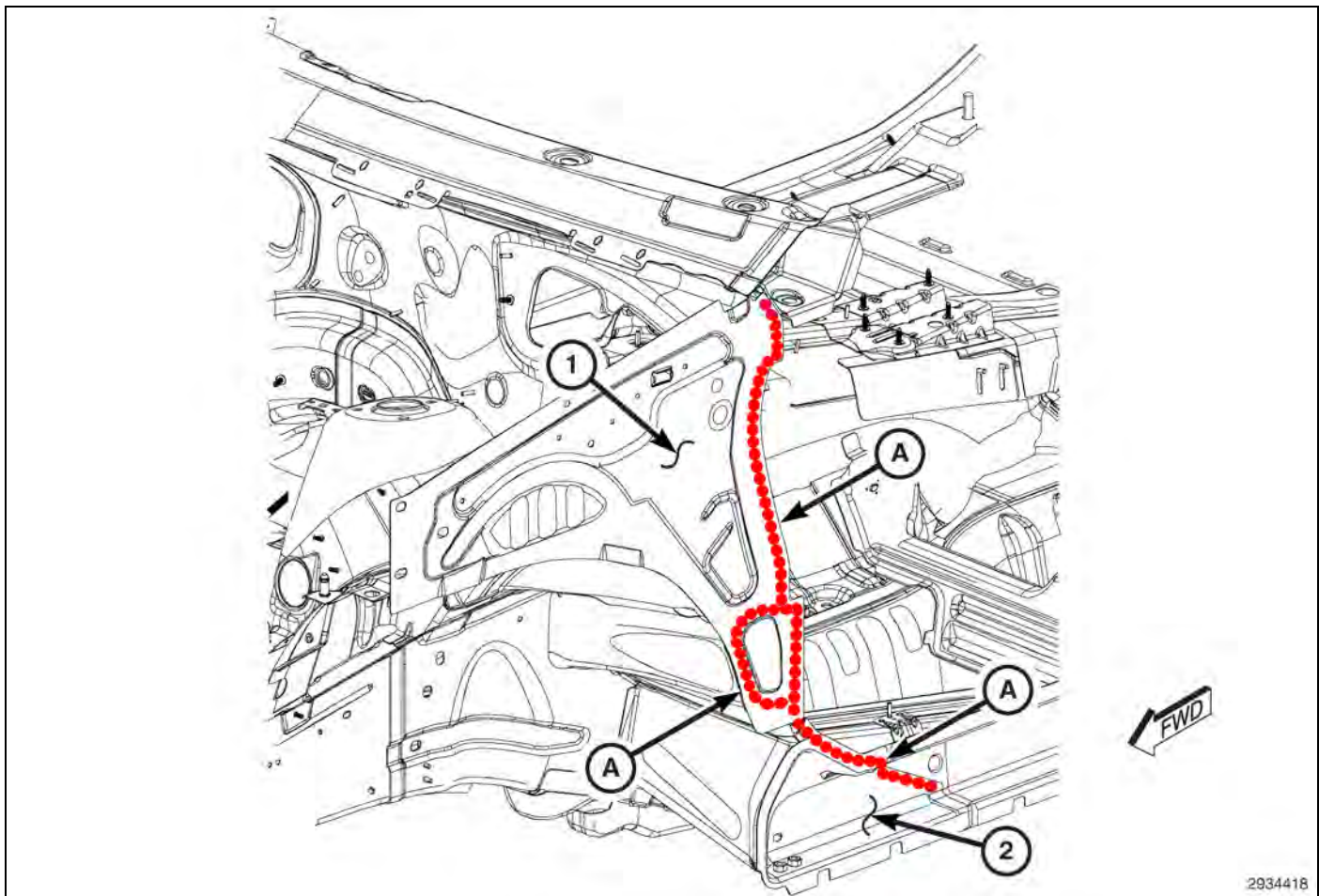
Fig. 71 Cowl Side / Sill Closeout
