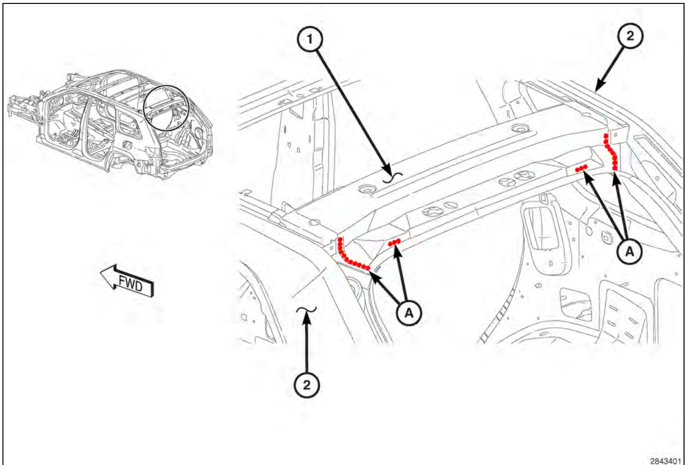
Fig. 59 Rear Roof Crossmember
