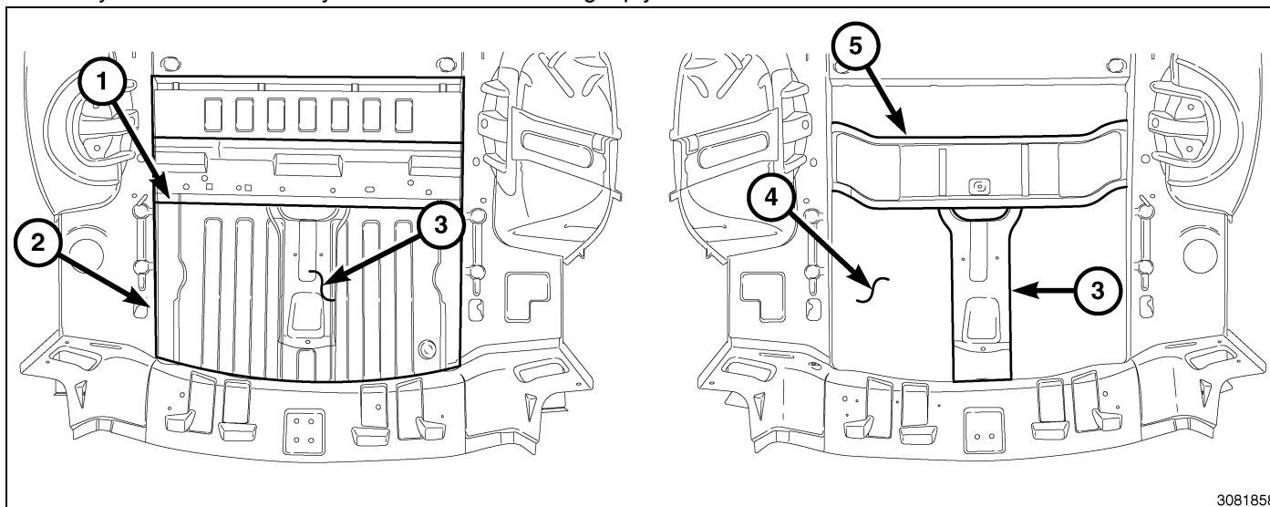
Fig. 24 Rear Floor Section (1 of 2)
