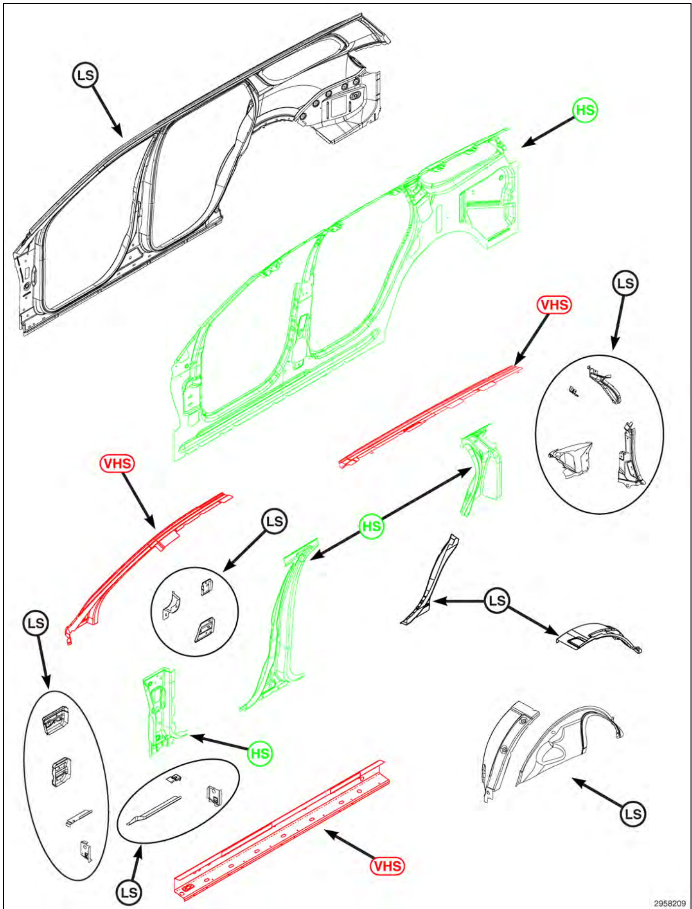
BODY IN WHITE COMPONENT IDENTIFICATION - BODY SIDE
