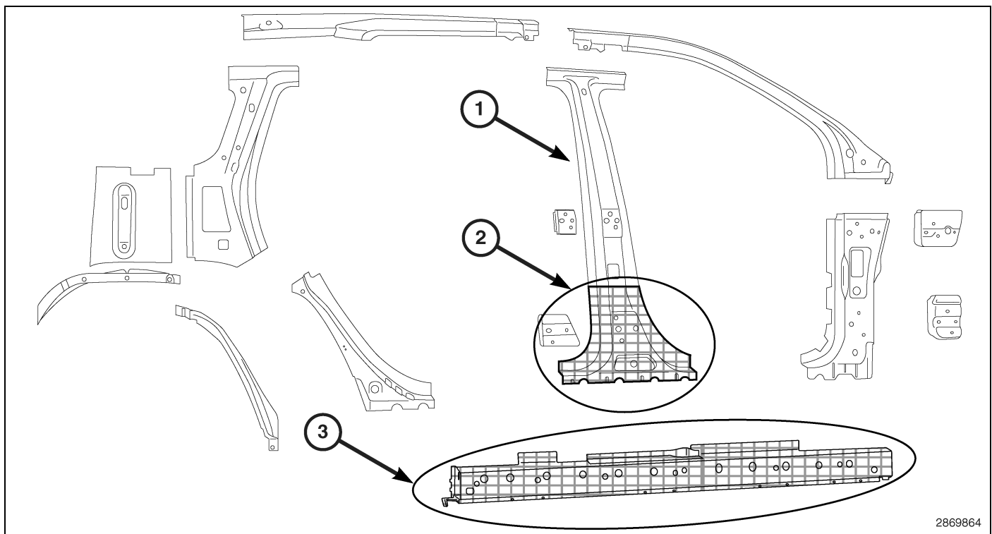
Fig. 20 Do Not Section
