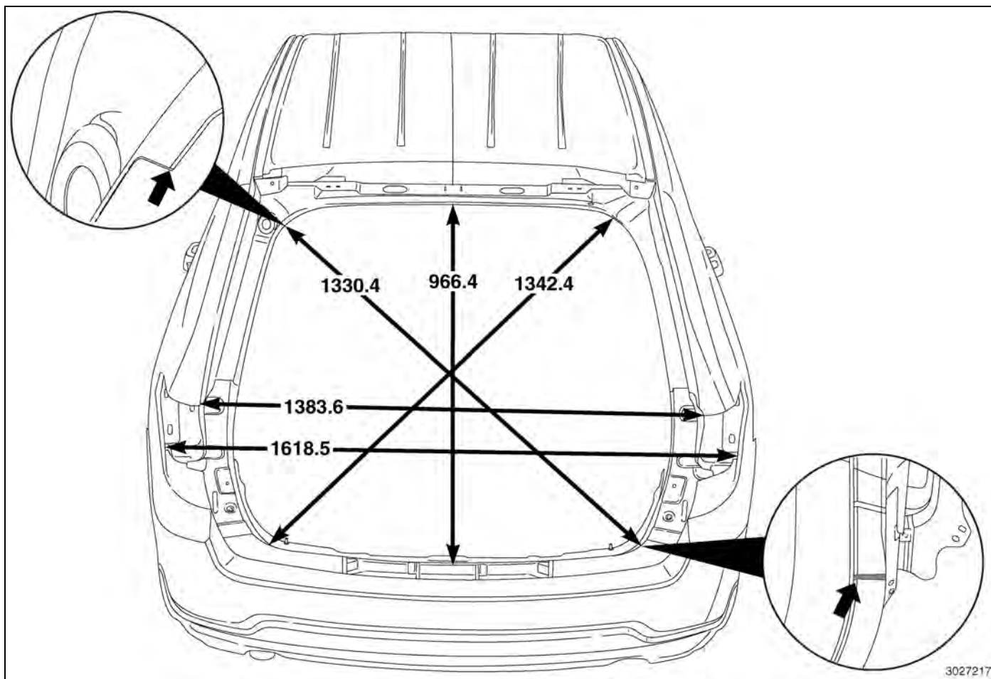
Fig. 3 Liftgate
