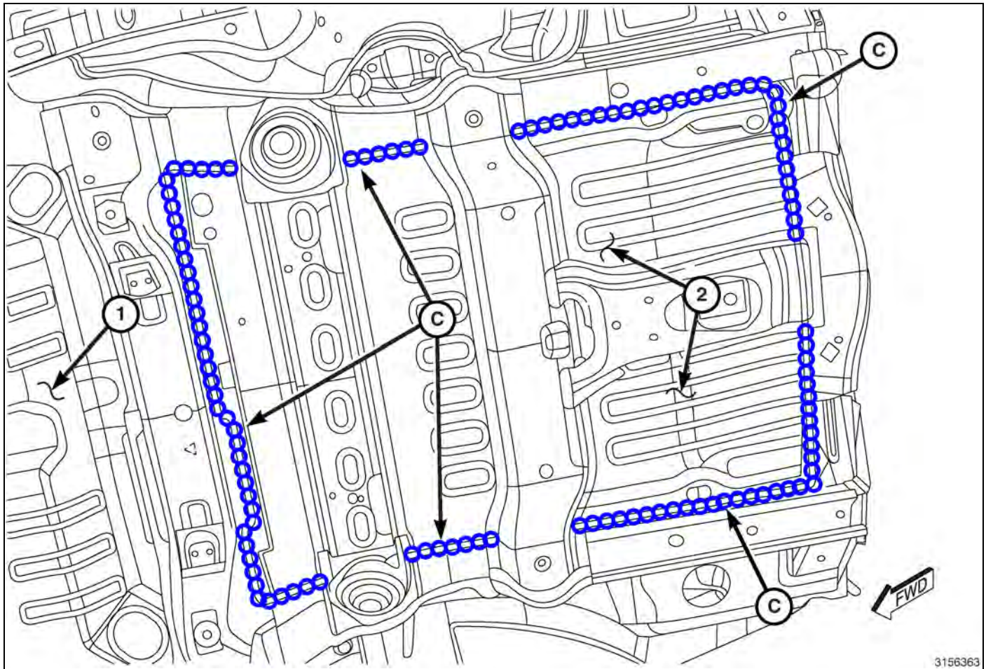
Fig. 82 Rear Floor (3 of 3)
