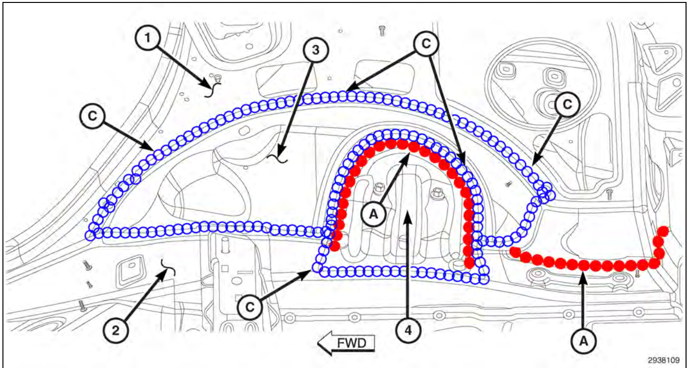
Fig. 88 Right Rear Wheelhouse (Interior)
