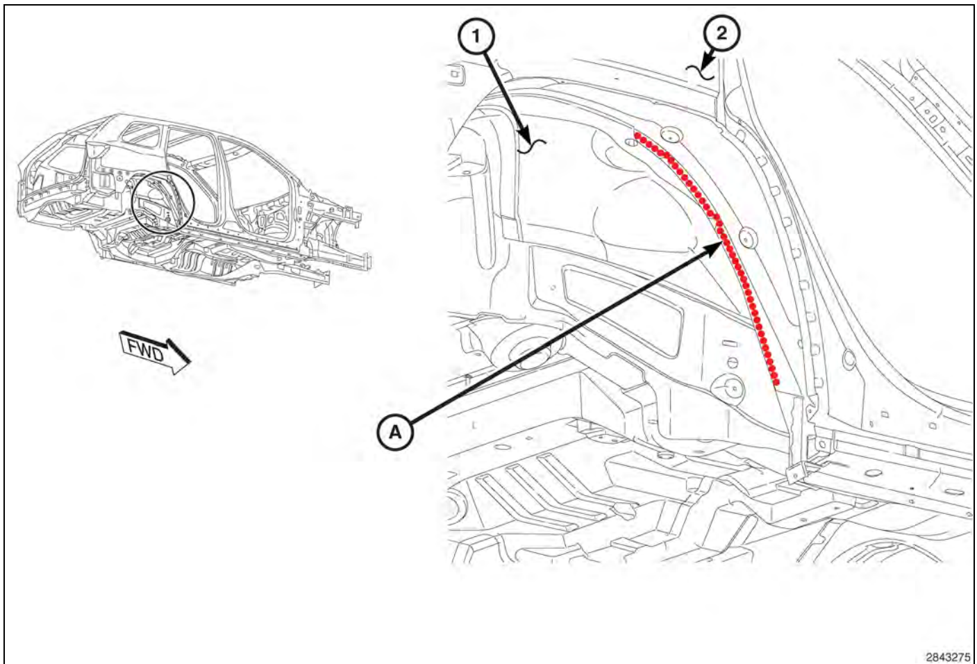
Fig. 92 Outer Wheelhouse / Inner Body Side Panel
