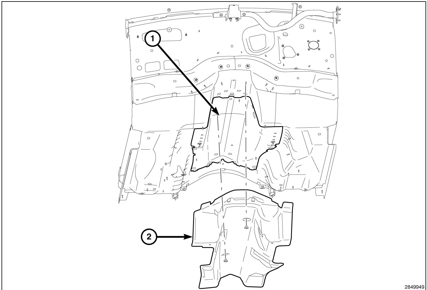
Fig. 38 Exterior Tunnel
