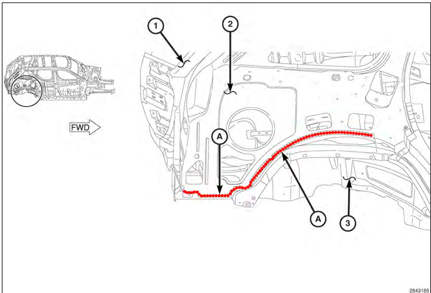
Fig. 91 Right Outer Wheelhouse / Inner Body Side
