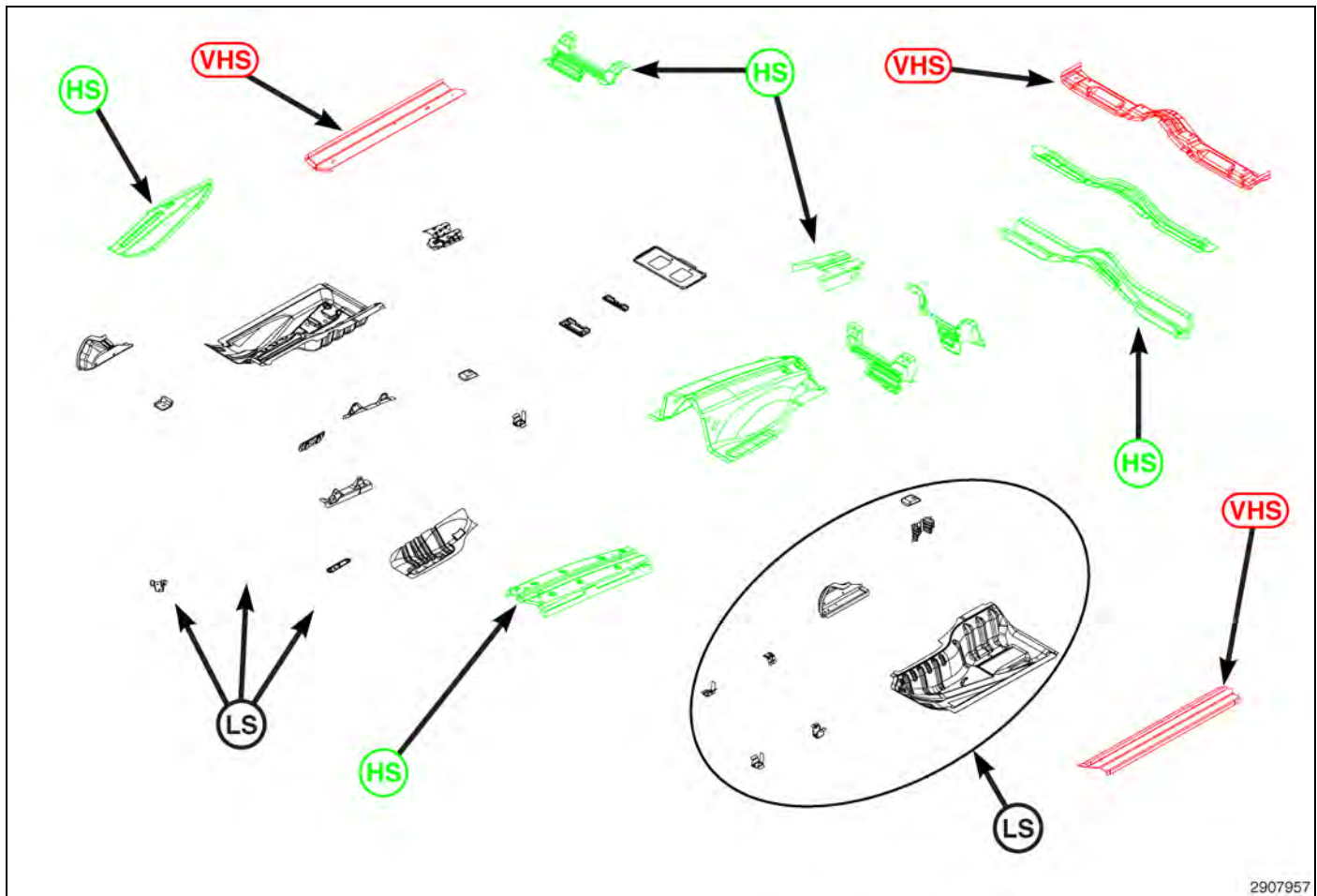
BODY IN WHITE COMPONENT IDENTIFICATION - FRONT / MID FLOOR
