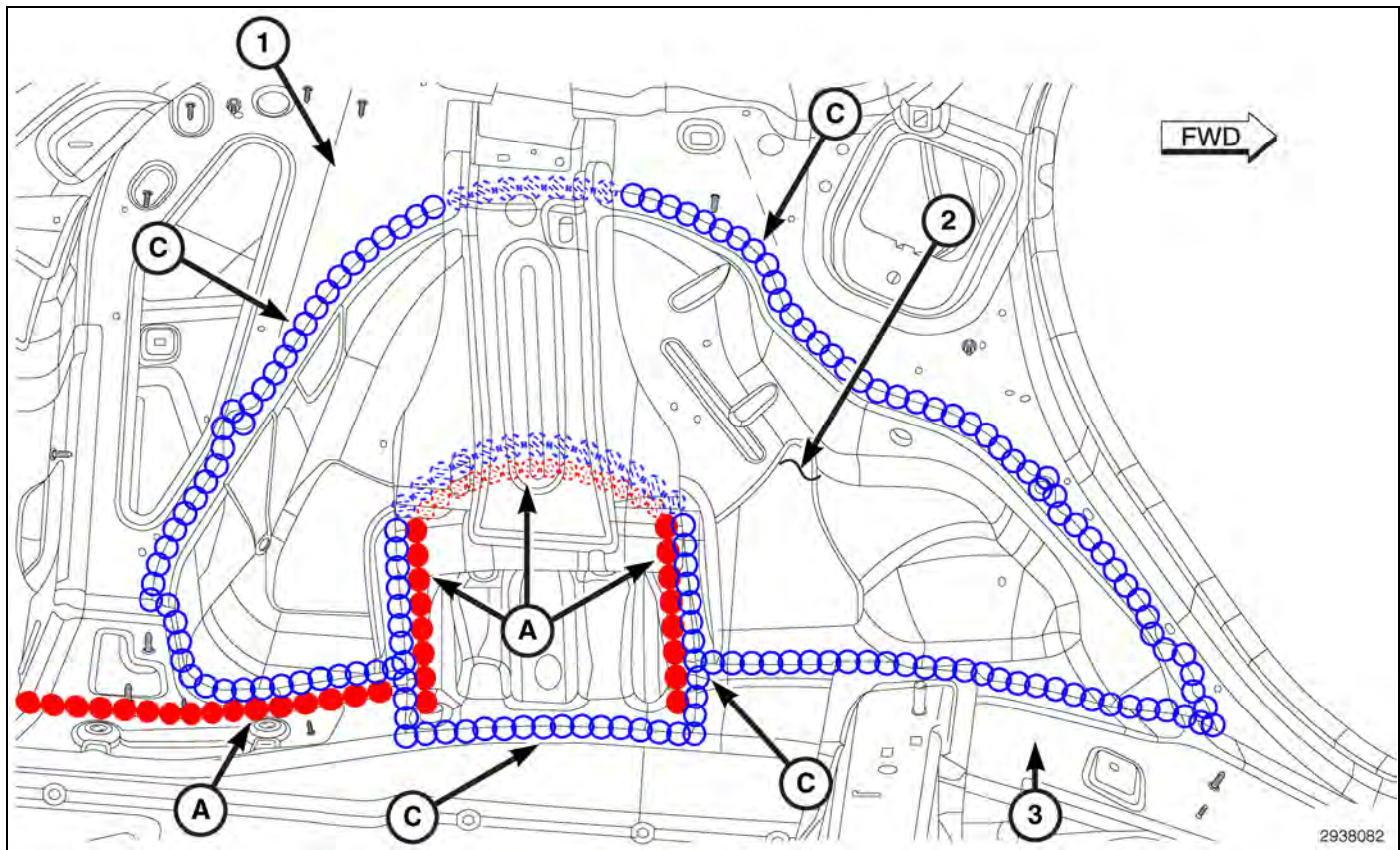
Fig. 84 Left Rear Wheelhouse (Interior)
