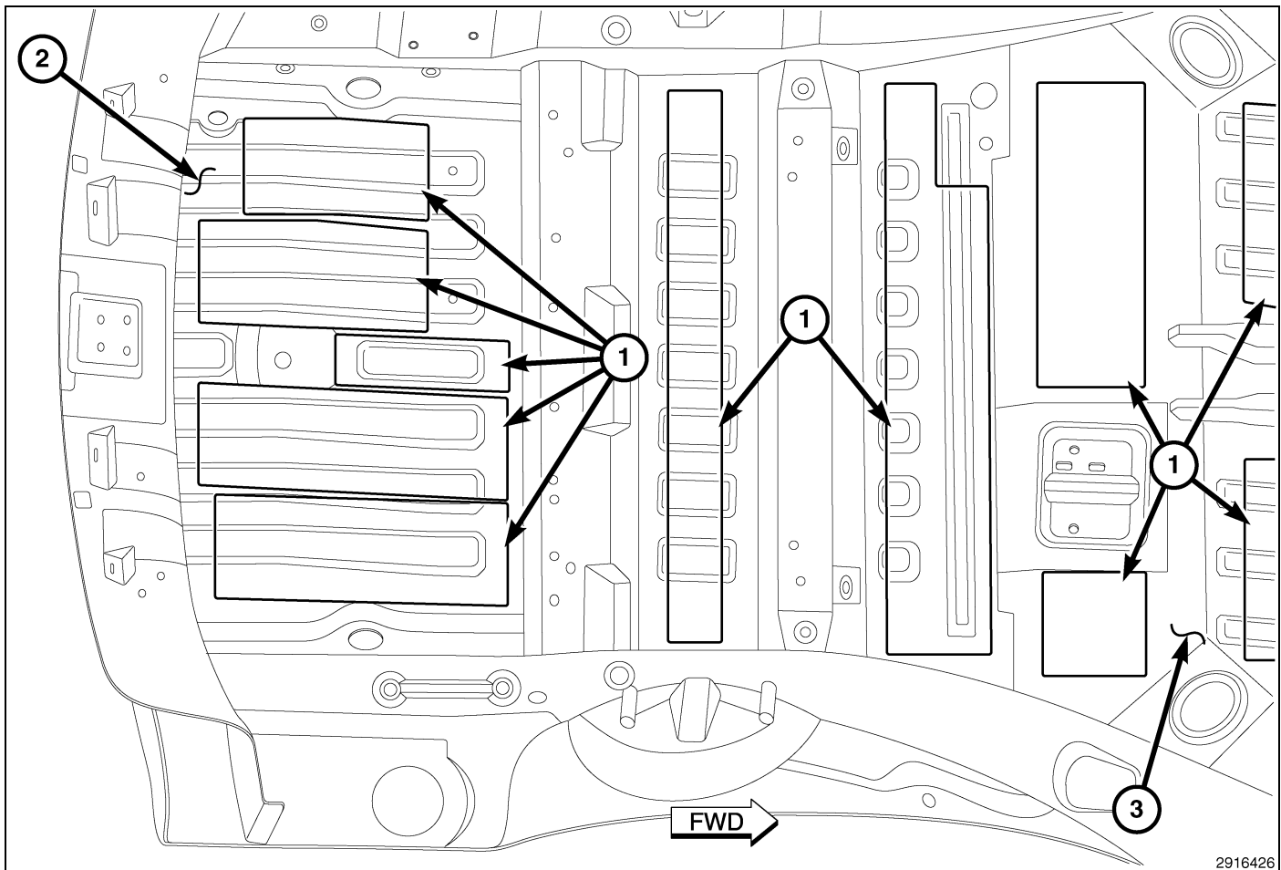
Fig. 48 Rear Floor (2 of 2)
