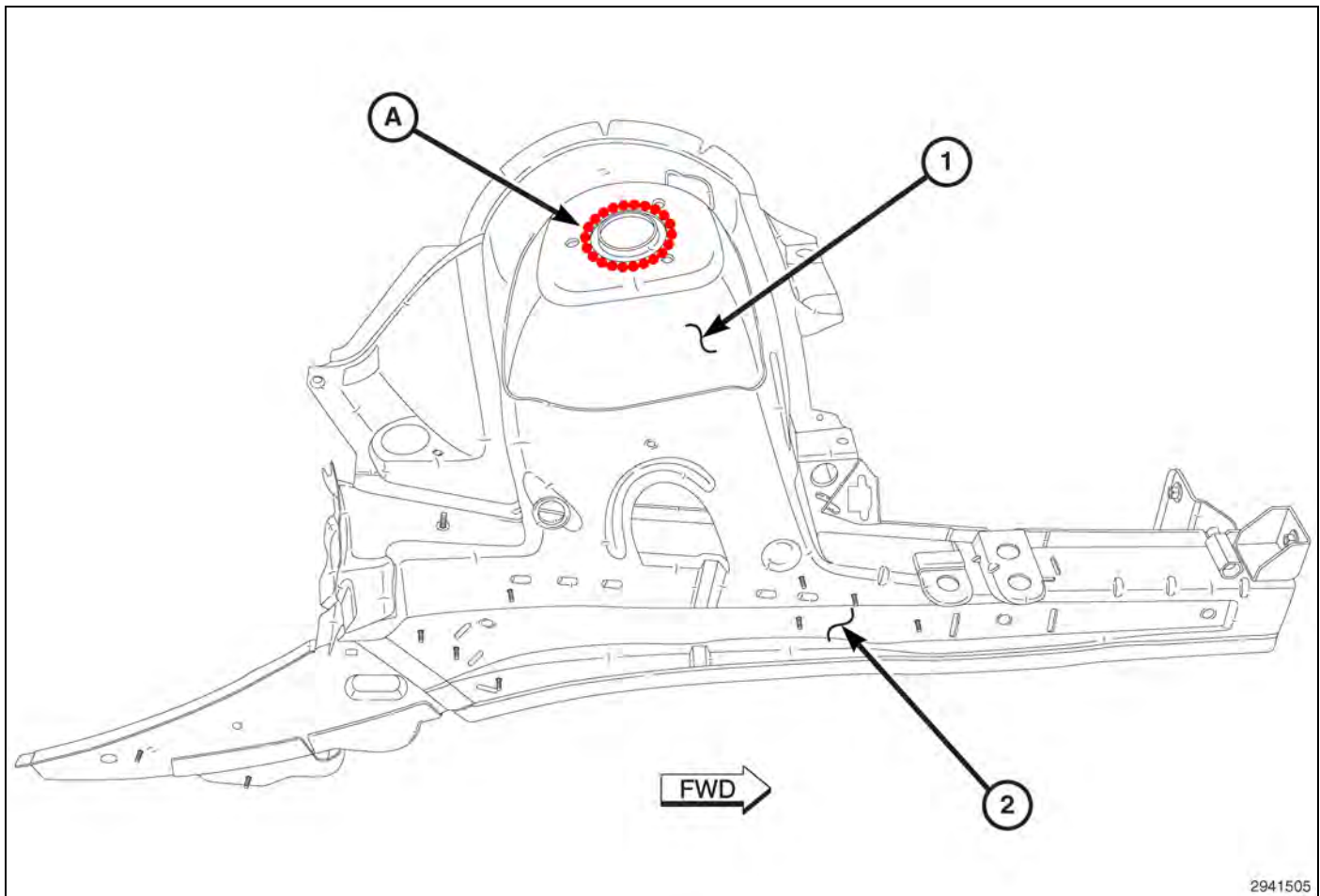
Fig. 62 Strut Tower Reinforcement
