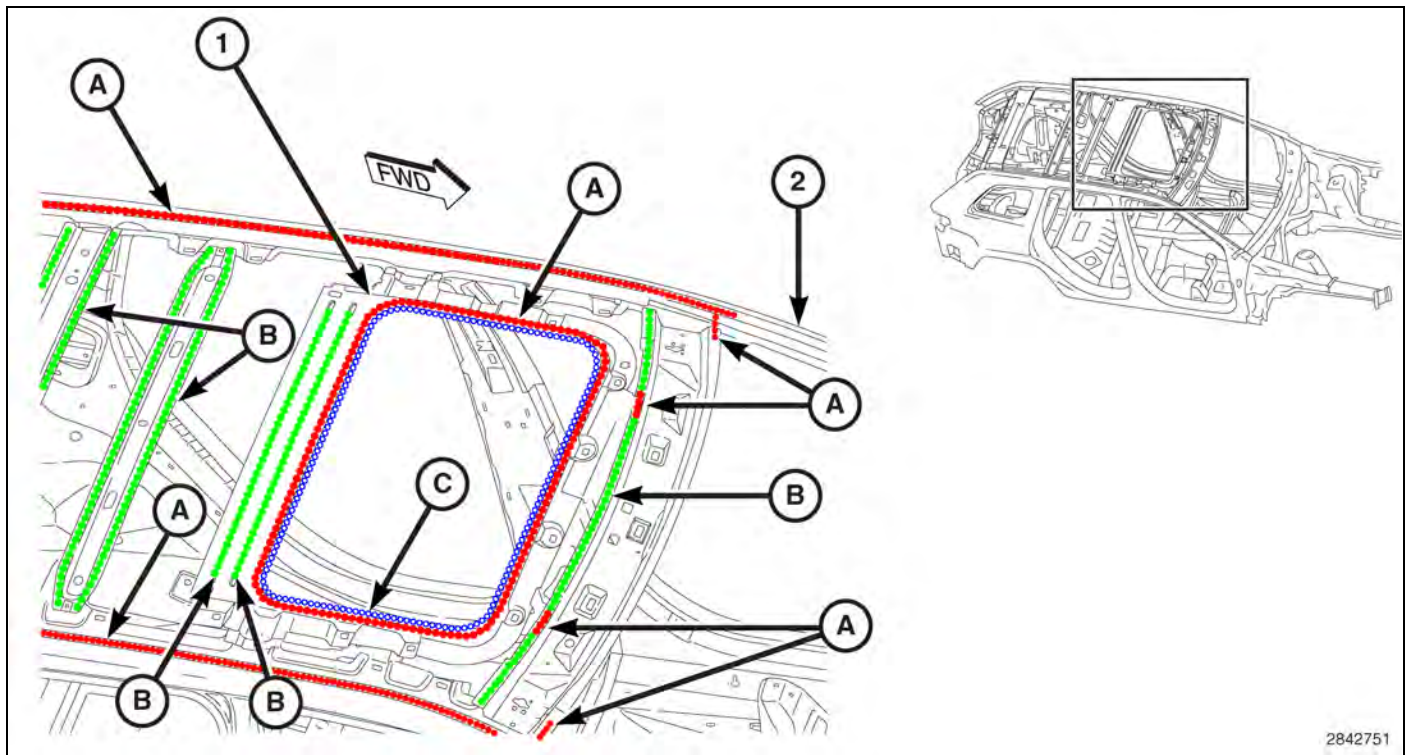
Fig. 58 Single Pane Sunroof Roof with Sunroof Support (2 of 2)
