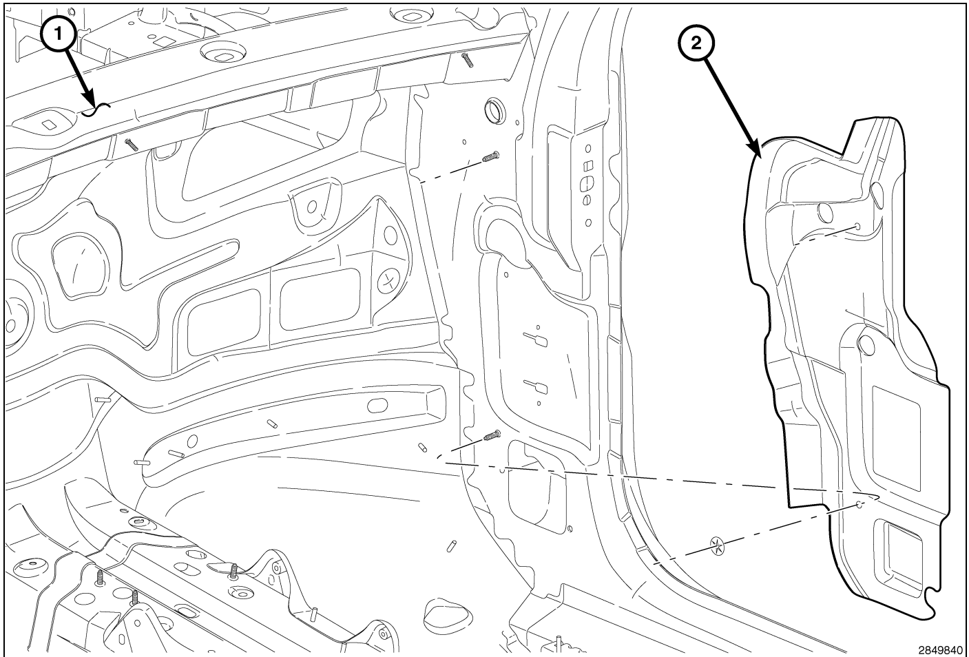
Fig. 36 Right Cowl
