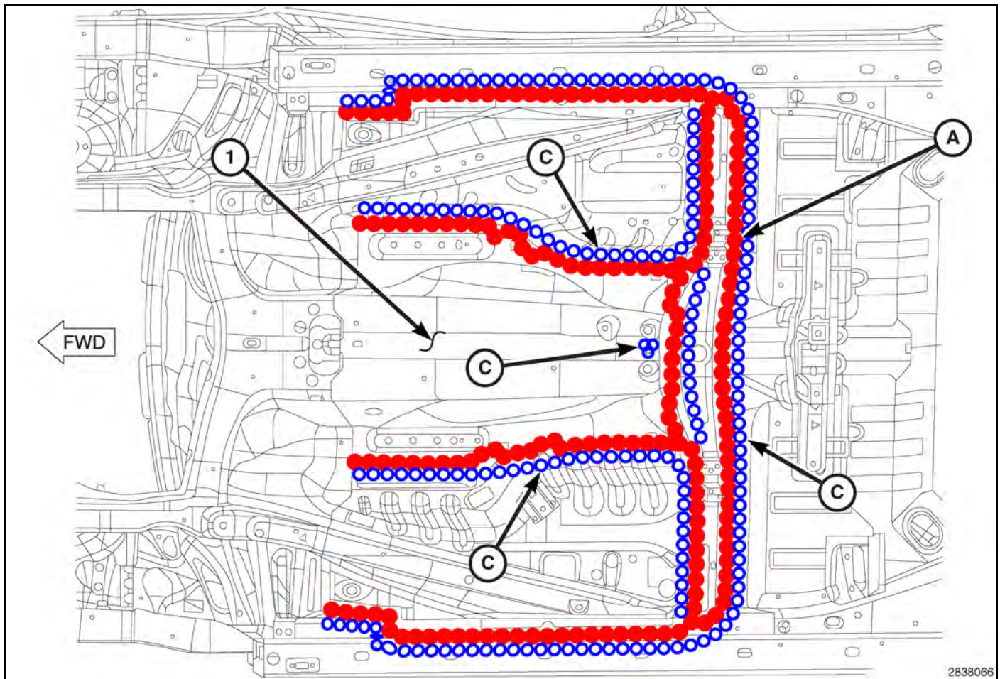
Fig. 72 FRONT FLOOR (1 of 2)
