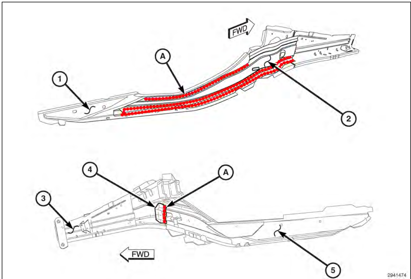
Fig. 61 Lower Rail Inner Bracket / Reinforcement
