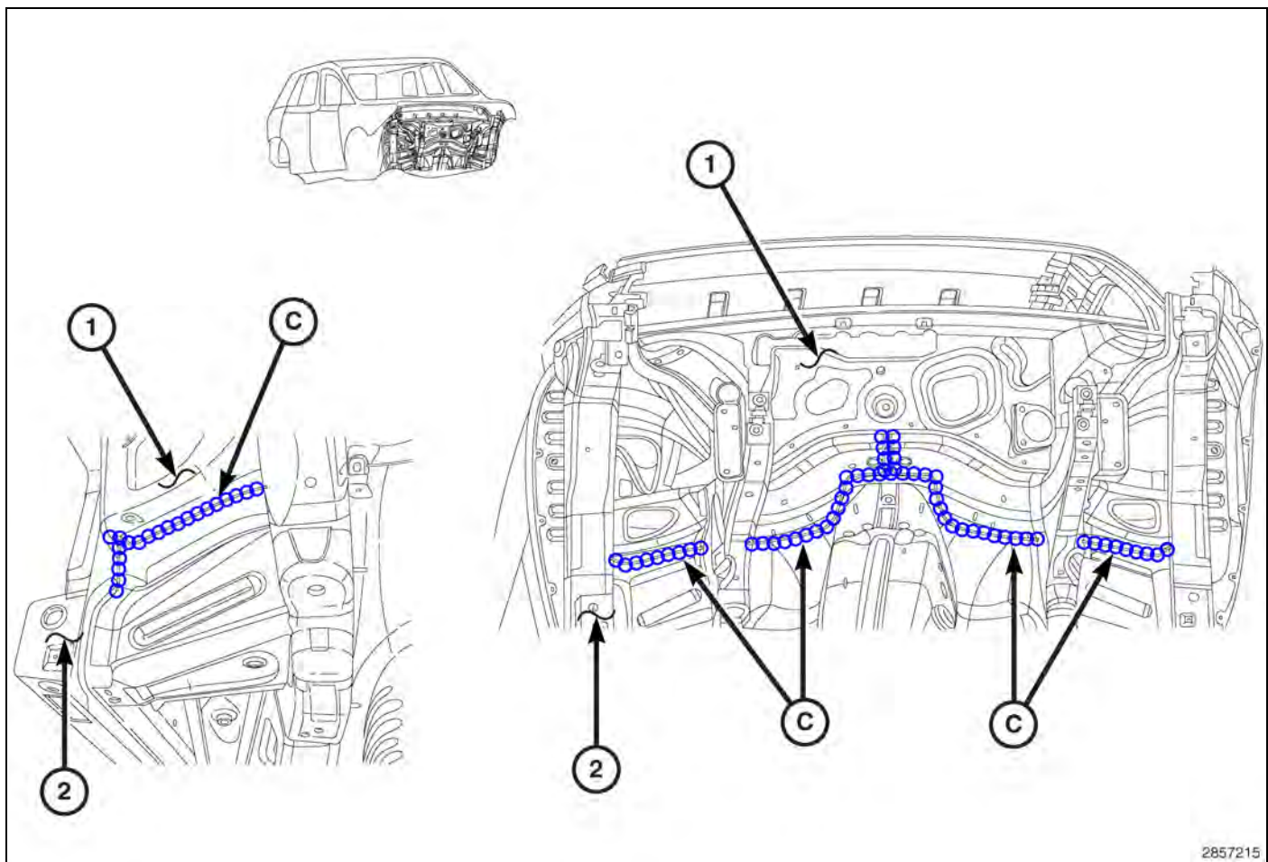
Fig. 67 Reinforcement Panel
