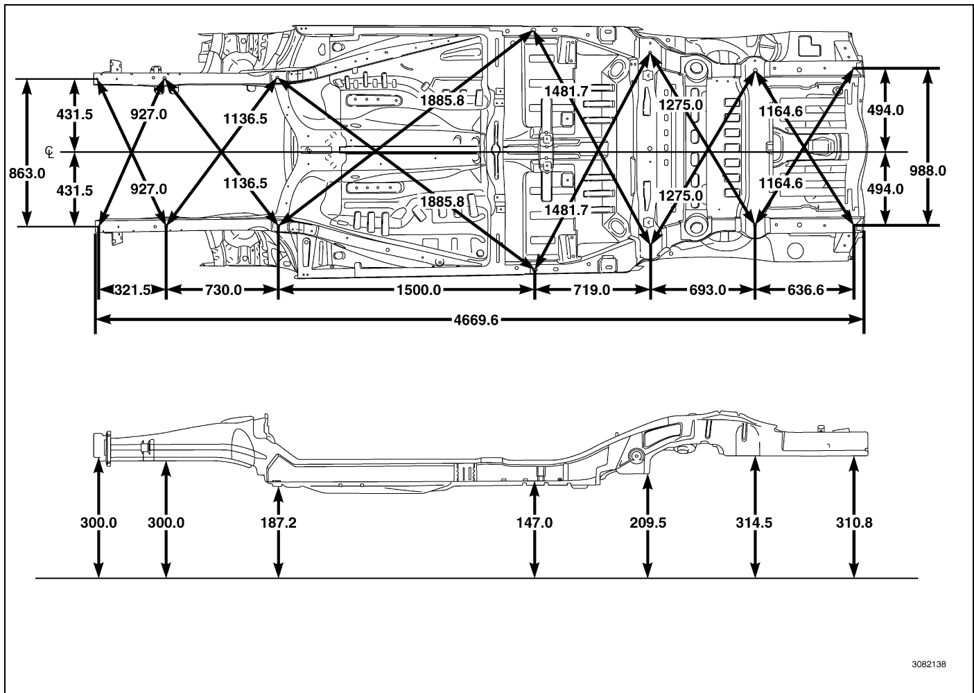
Fig. 4 Underbody Dimensions
