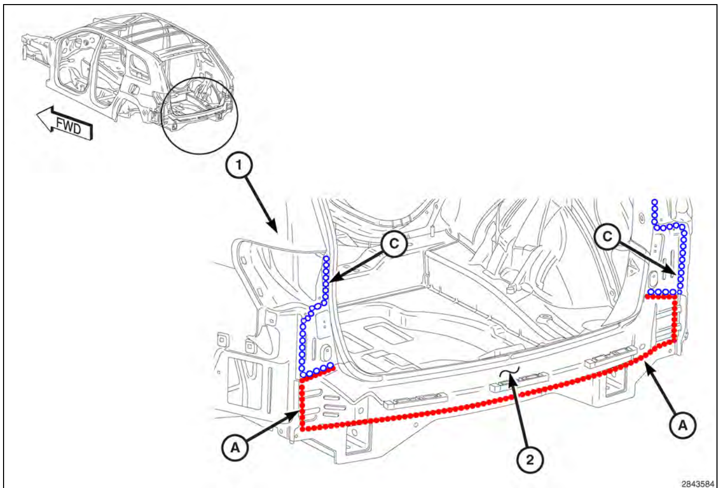
Fig. 97 Rear Crossmember / Body Side Panel
