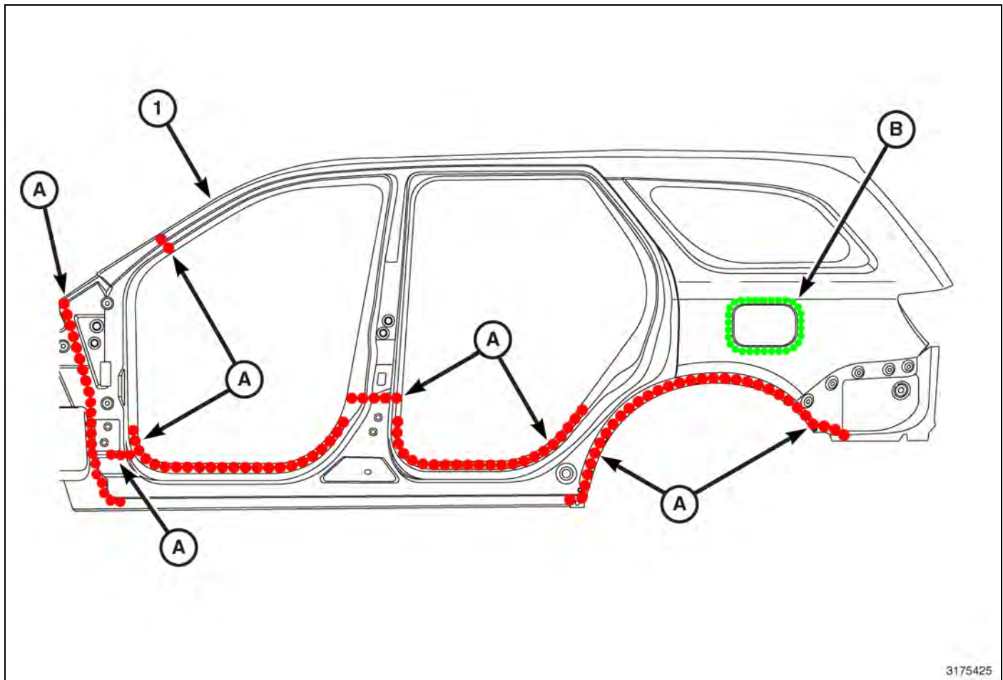
Fig. 52 Left Body Side Aperture
