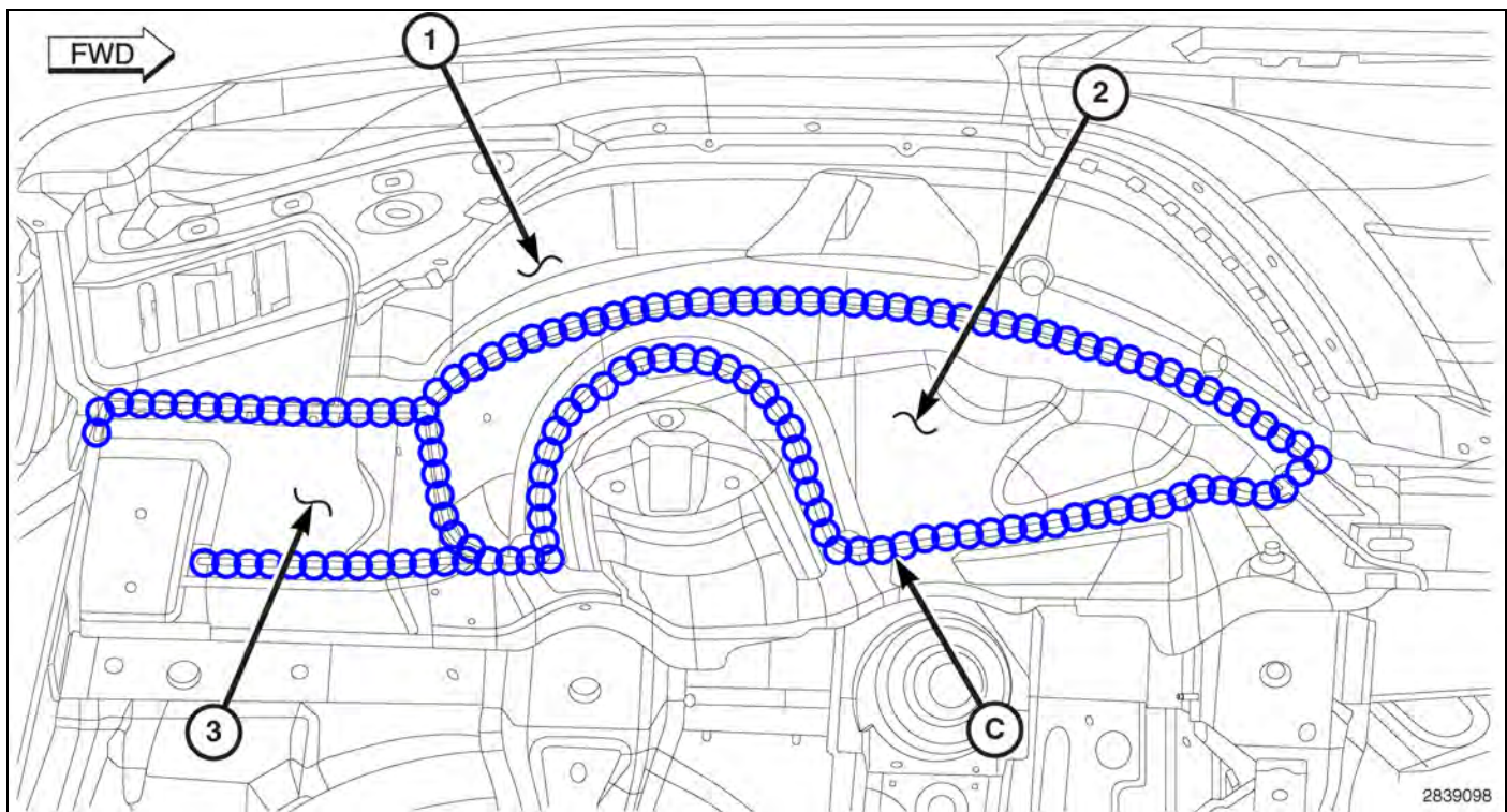
Fig. 89 Right Wheelhouse (Exterior)
