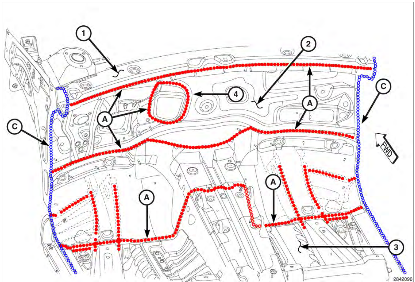
Fig. 66 Lower Dash / Front Floor
