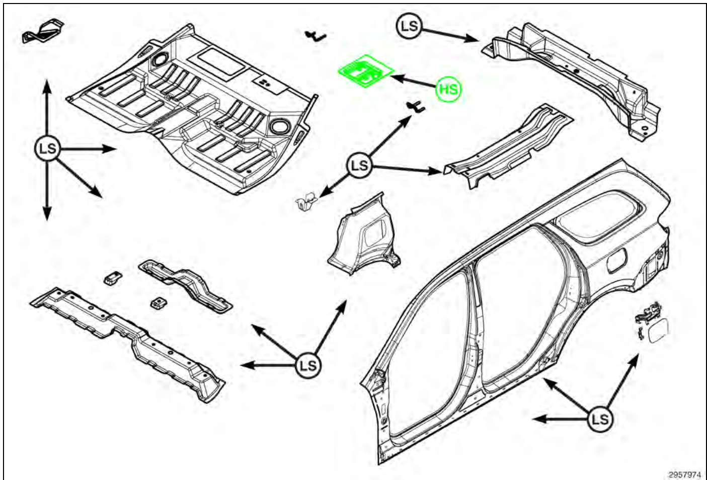
BODY IN WHITE COMPONENT IDENTIFICATION - BODY SIDE / MID FLOOR
