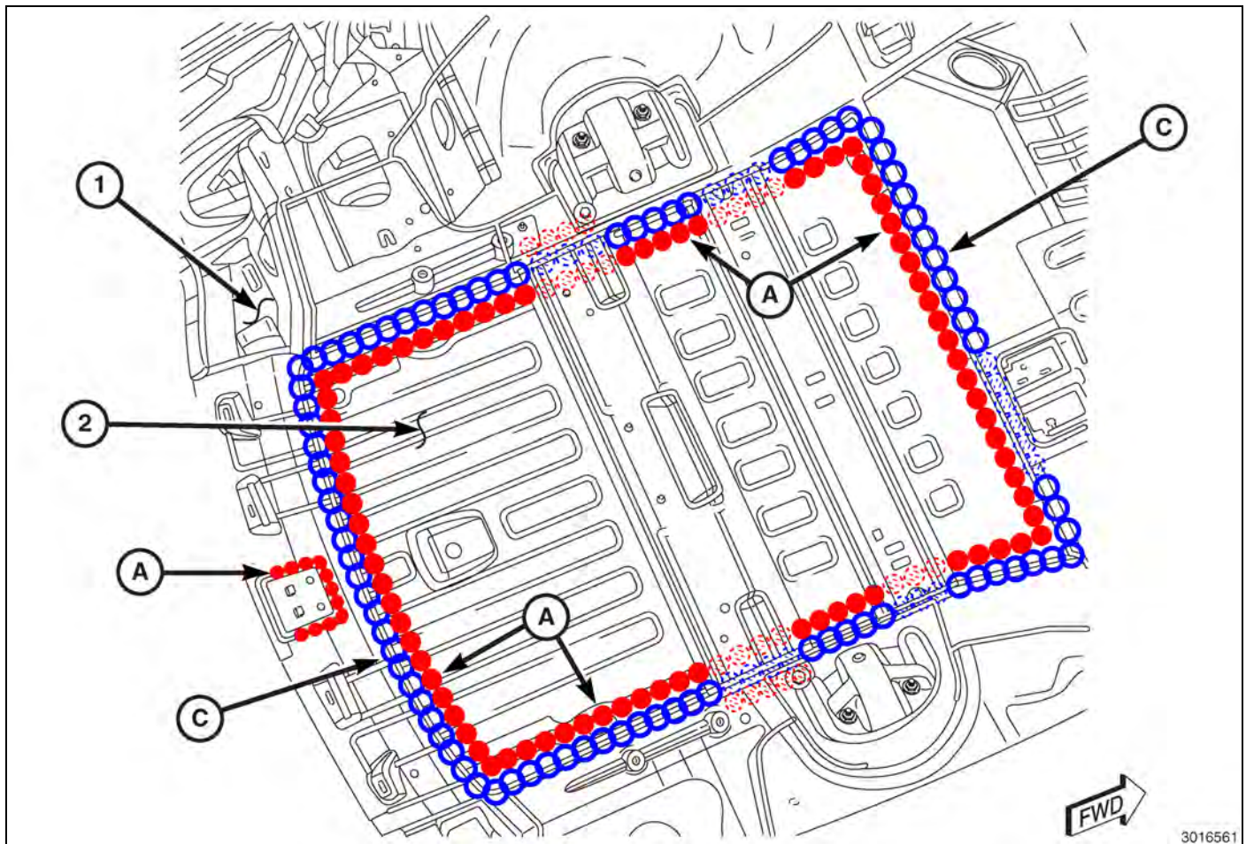
Fig. 80 Rear Floor (1 of 3)
