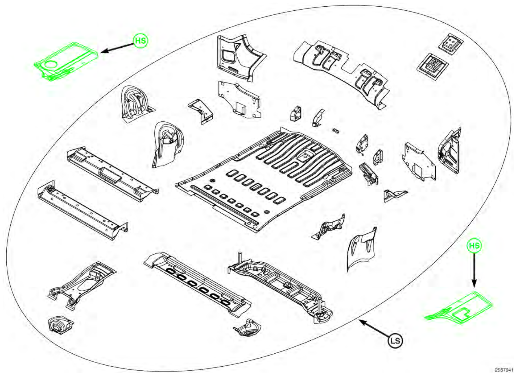
BODY IN WHITE COMPONENT IDENTIFICATION - REAR FLOOR
