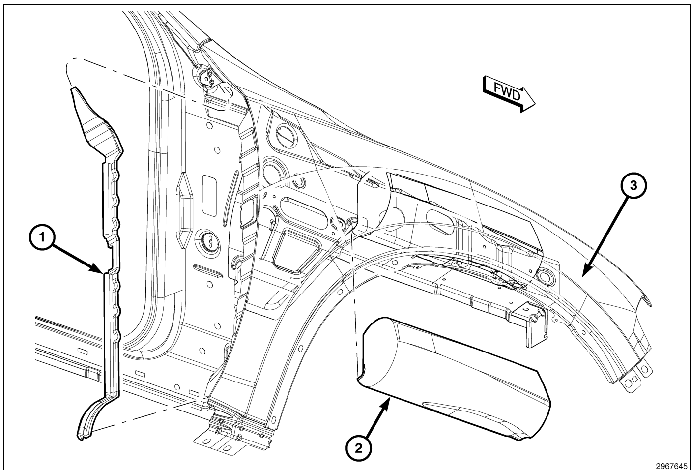
Fig. 31 Fender (2 of 2)
