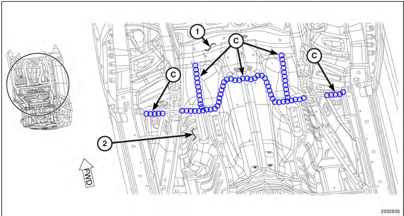
Fig. 70 Dash Reinforcement / Front Floor (2 of 2)
