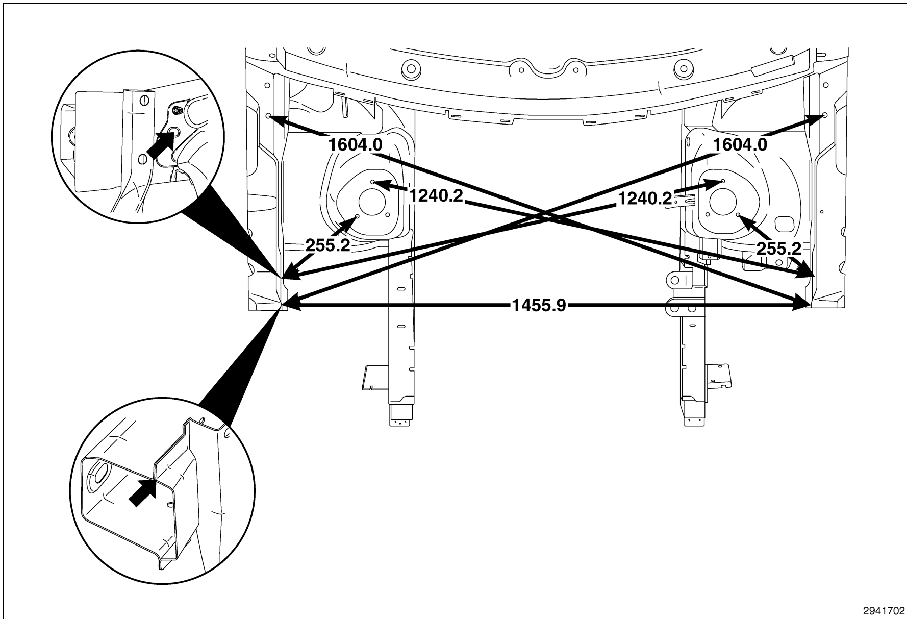
Fig. 5 Under Hood Quick Reference
