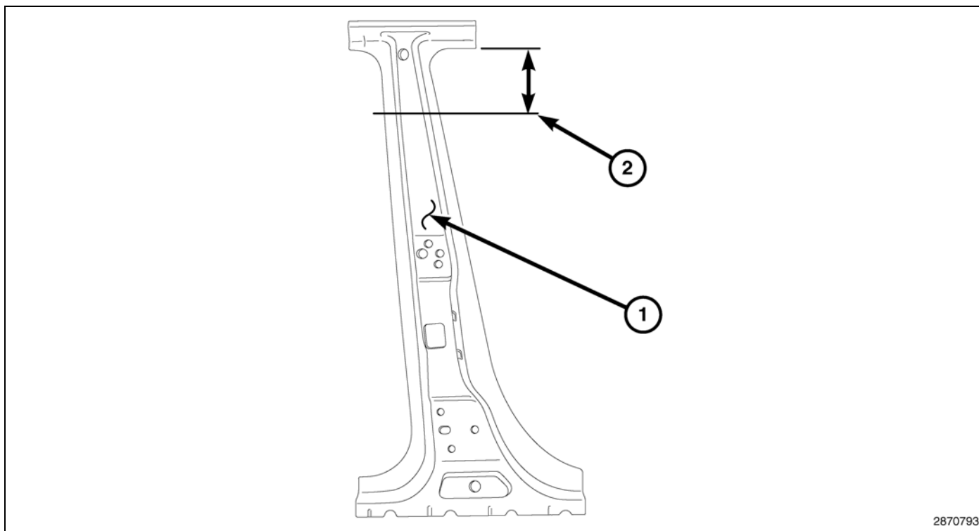
Fig. 22 B-Pillar Reinforcement
