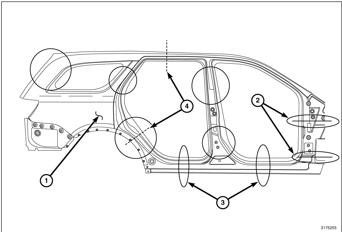
Fig. 19 Outer Body Side Aperture
