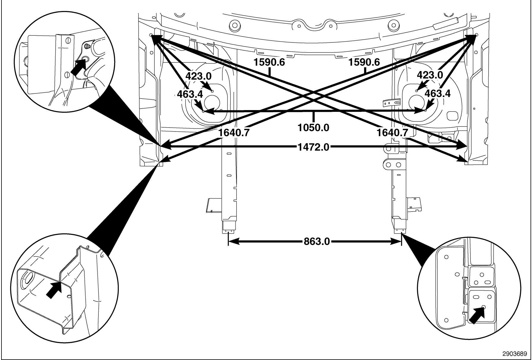
Fig. 6 Under Hood
