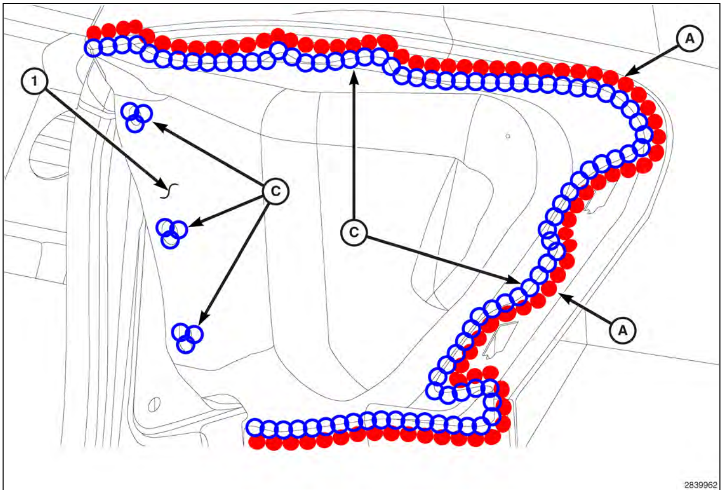
Fig. 96 Tail Lamp Pocket
