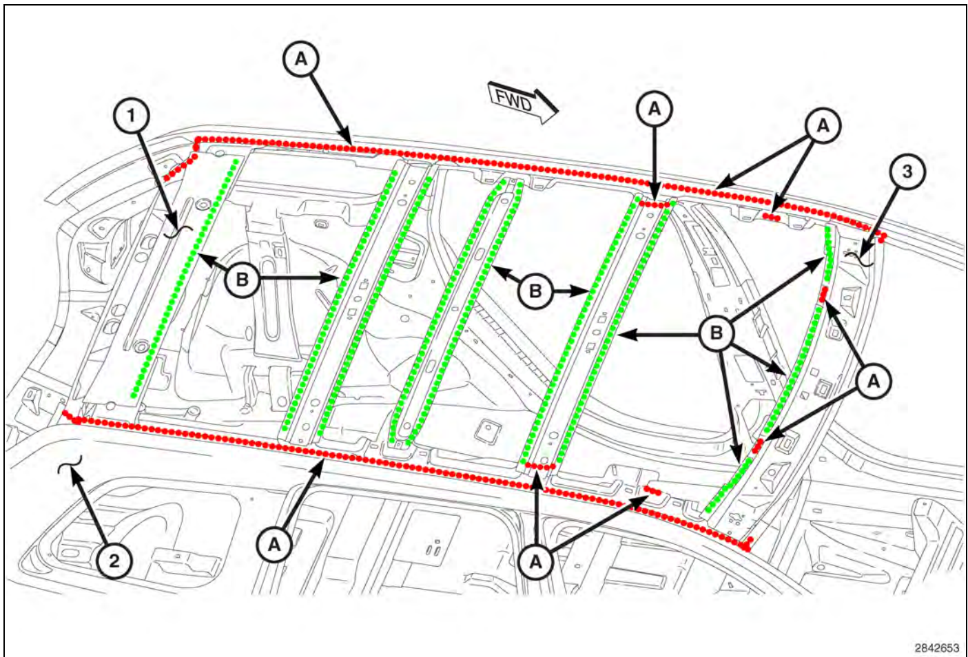
Fig. 56 Roof / Body Side
