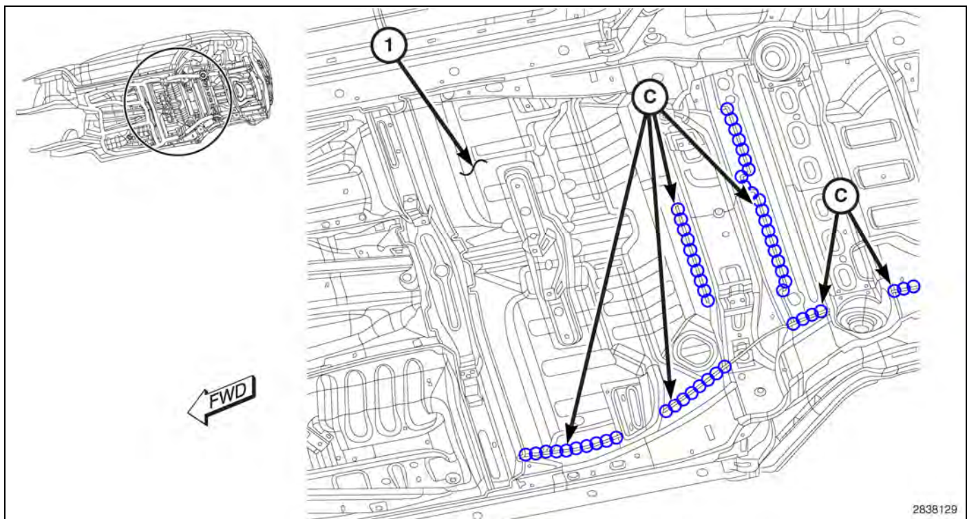
Fig. 79 Mid Floor (3 of 3)
