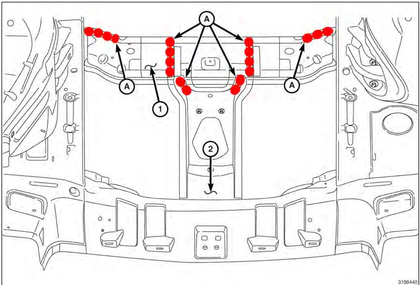
Fig. 81 Rear Floor (2 of 3)
