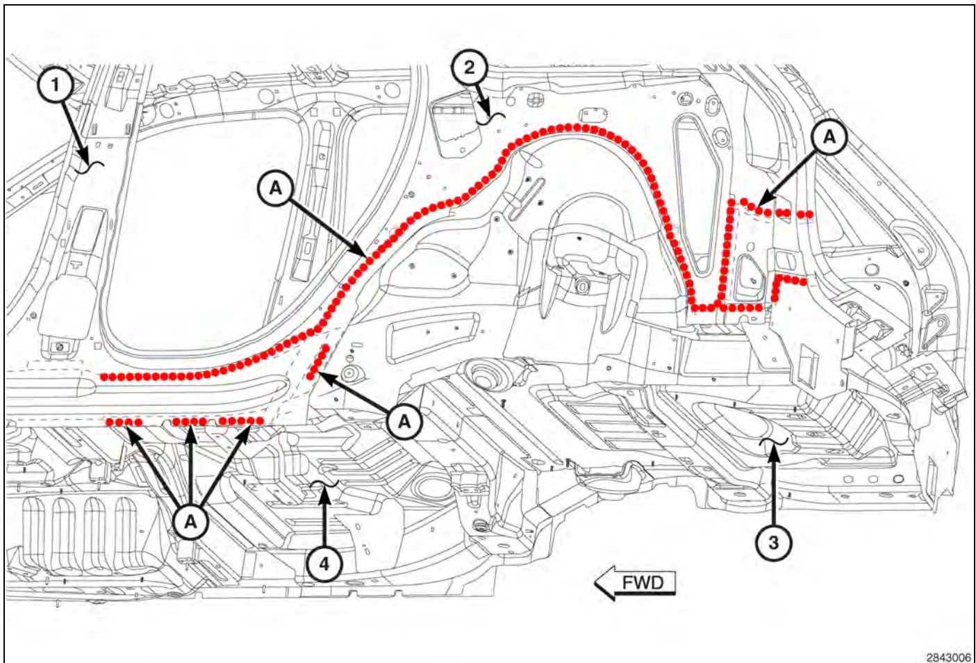
Fig. 86 Left Inner Wheelhouse / Inner Body Side Panel
