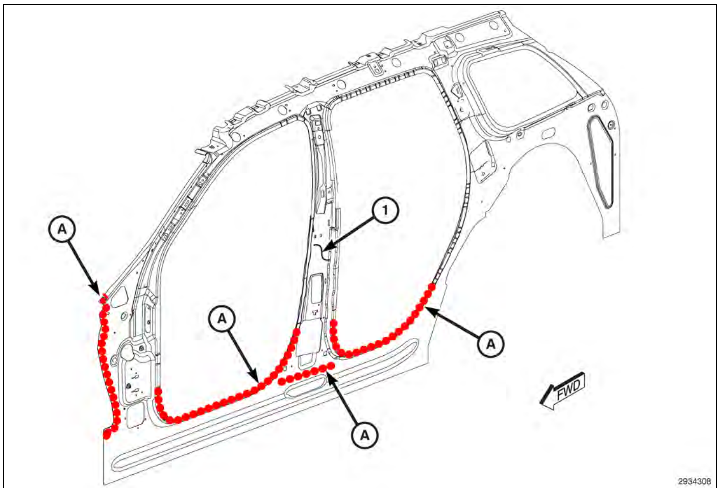
Fig. 75 Inner Body Side / Reinforcement Assembly
