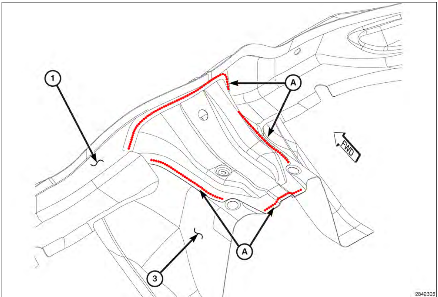
Fig. 69 Dash Reinforcement / Front Floor (1 of 2)
