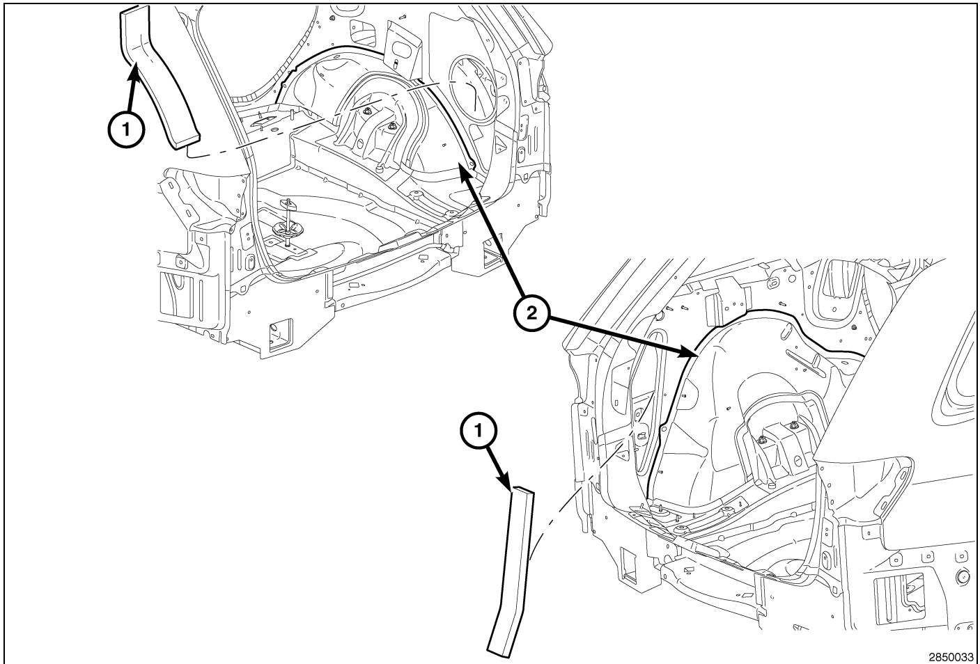
Fig. 42 Wheelhouse (2 of 3)
