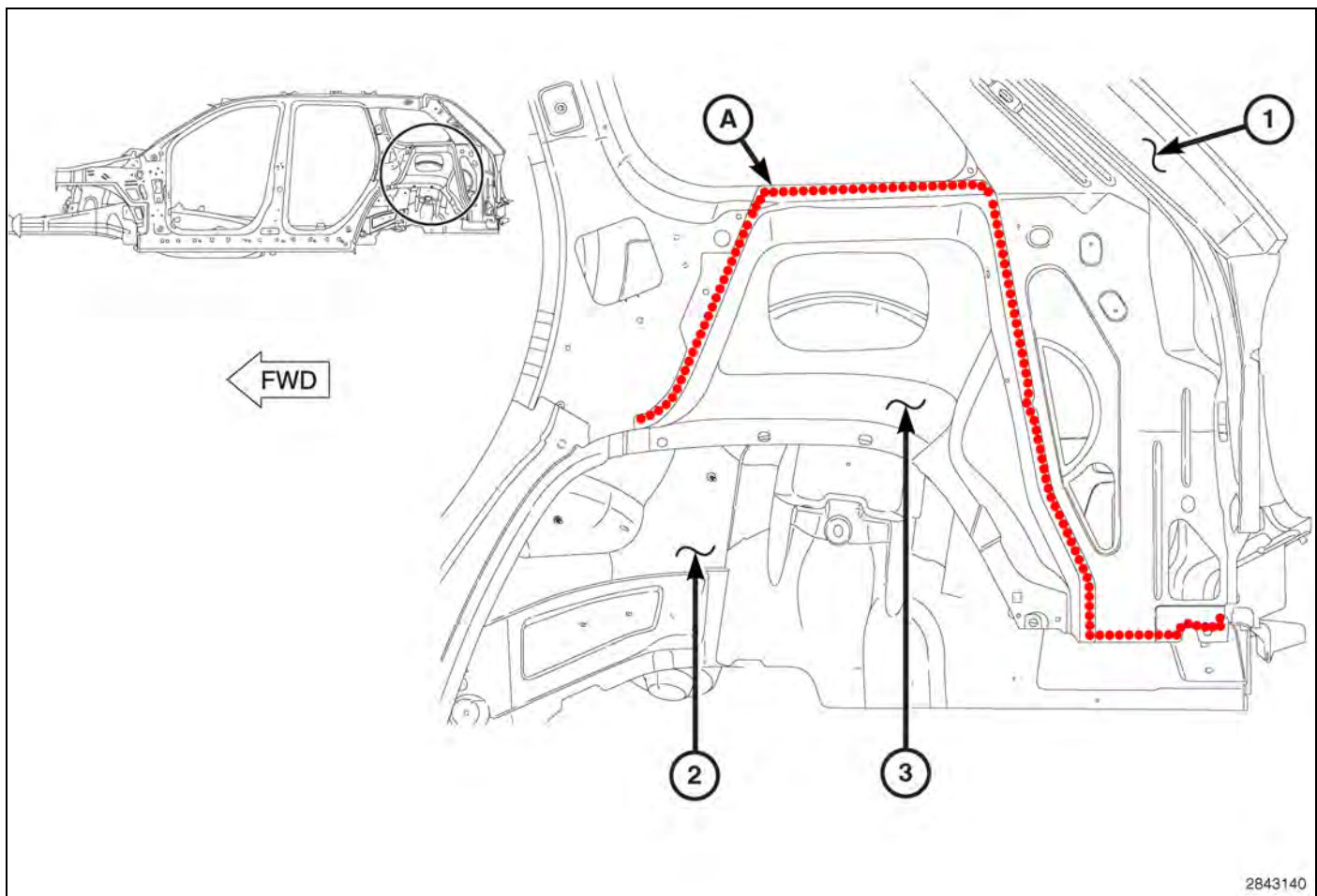
Fig. 87 Left Inner Body Side / Outer Wheelhouse
