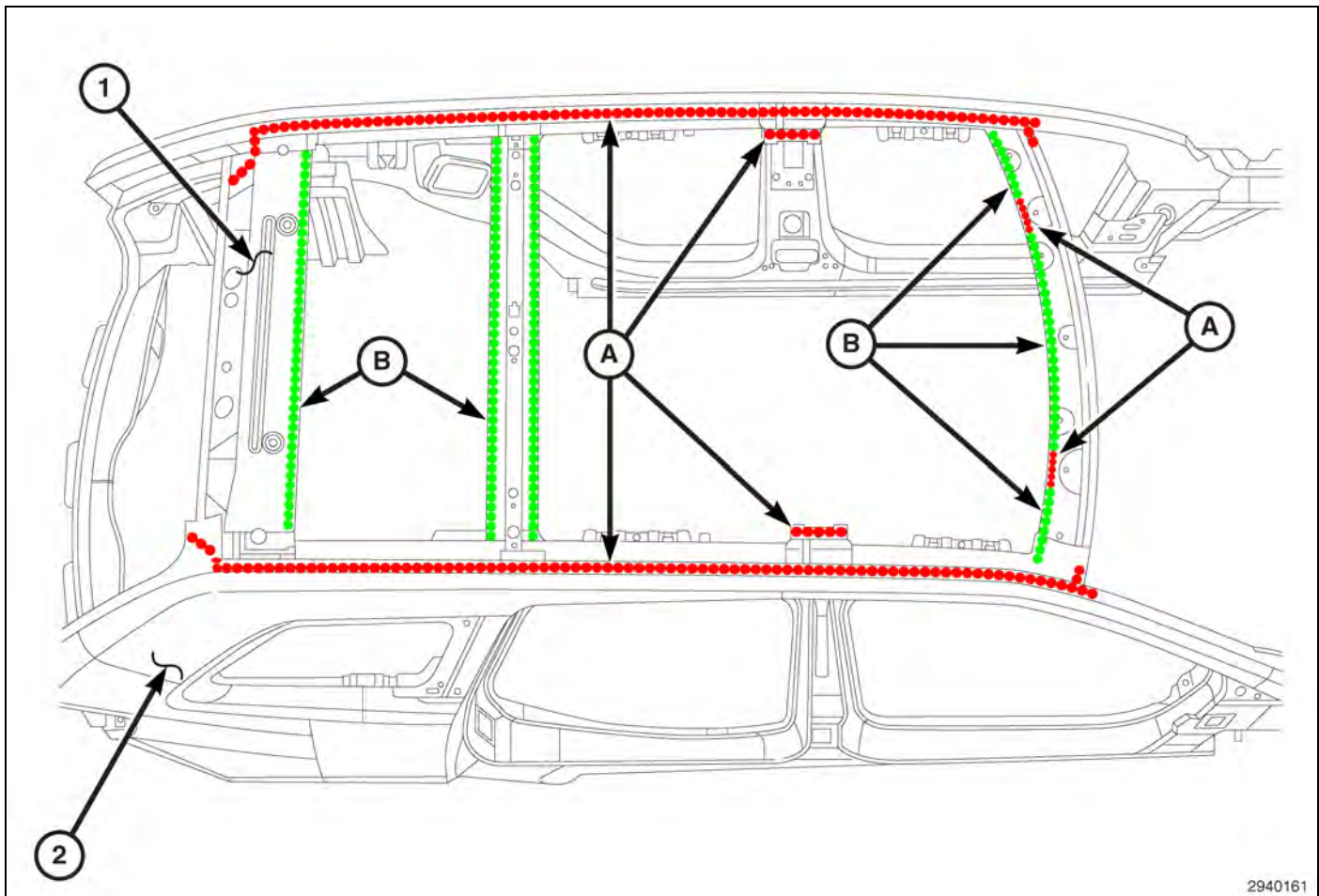
Fig. 57 Single Pane Sunroof Roof without Sunroof Support (1 of 2)
