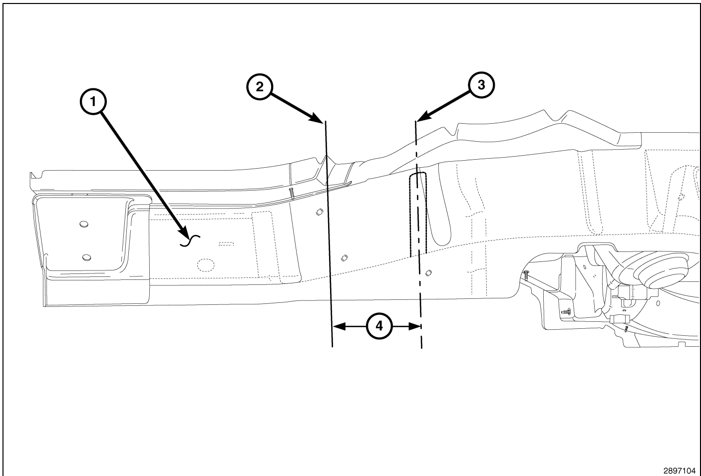
Fig. 27 Rear Rail
