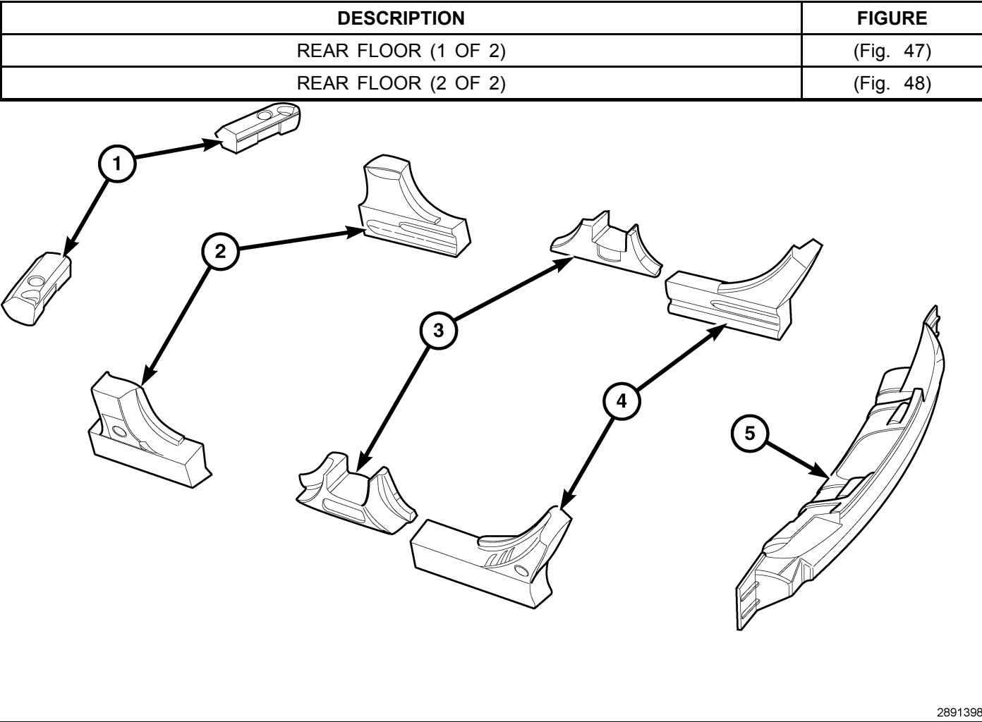
Fig. 28 PUR Foam Locations
