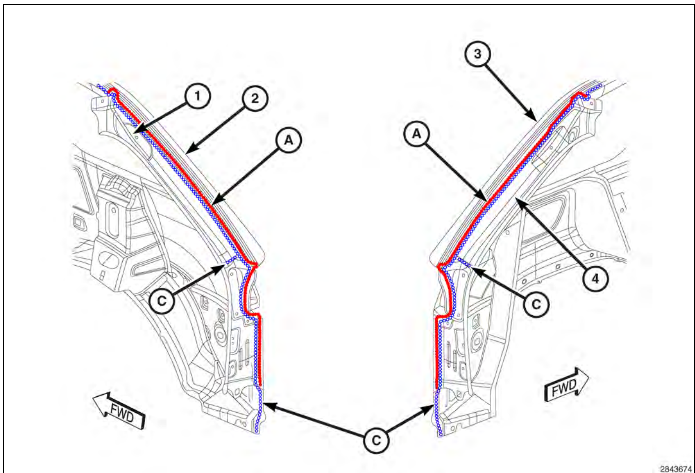
Fig. 95 D-Pillar Drain Trough / Outer Body Side Panel
