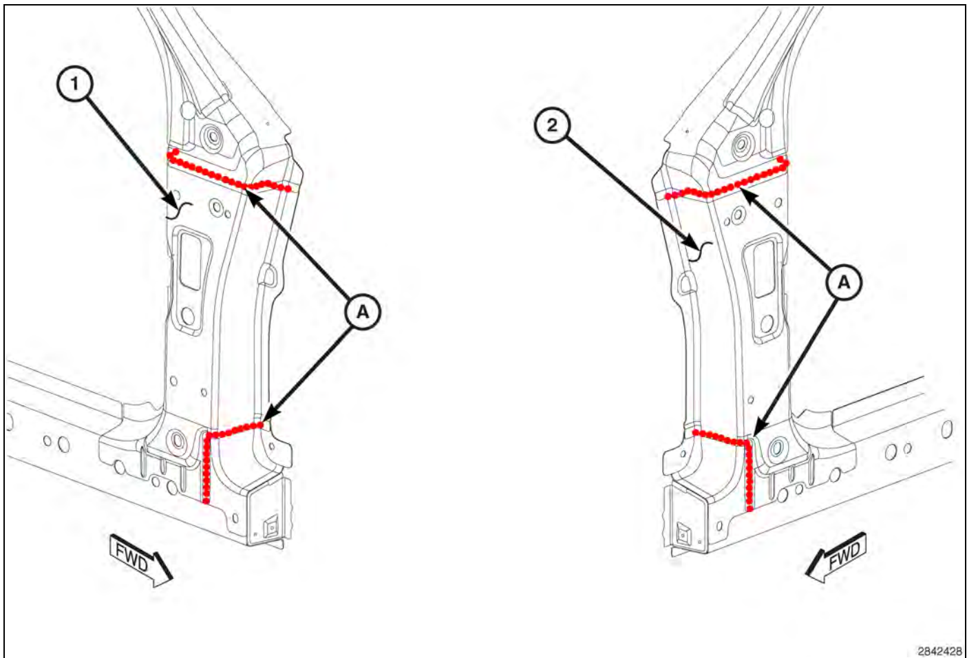
Fig. 63 Body Side Panels / Front Door Hinge Reinforcement
