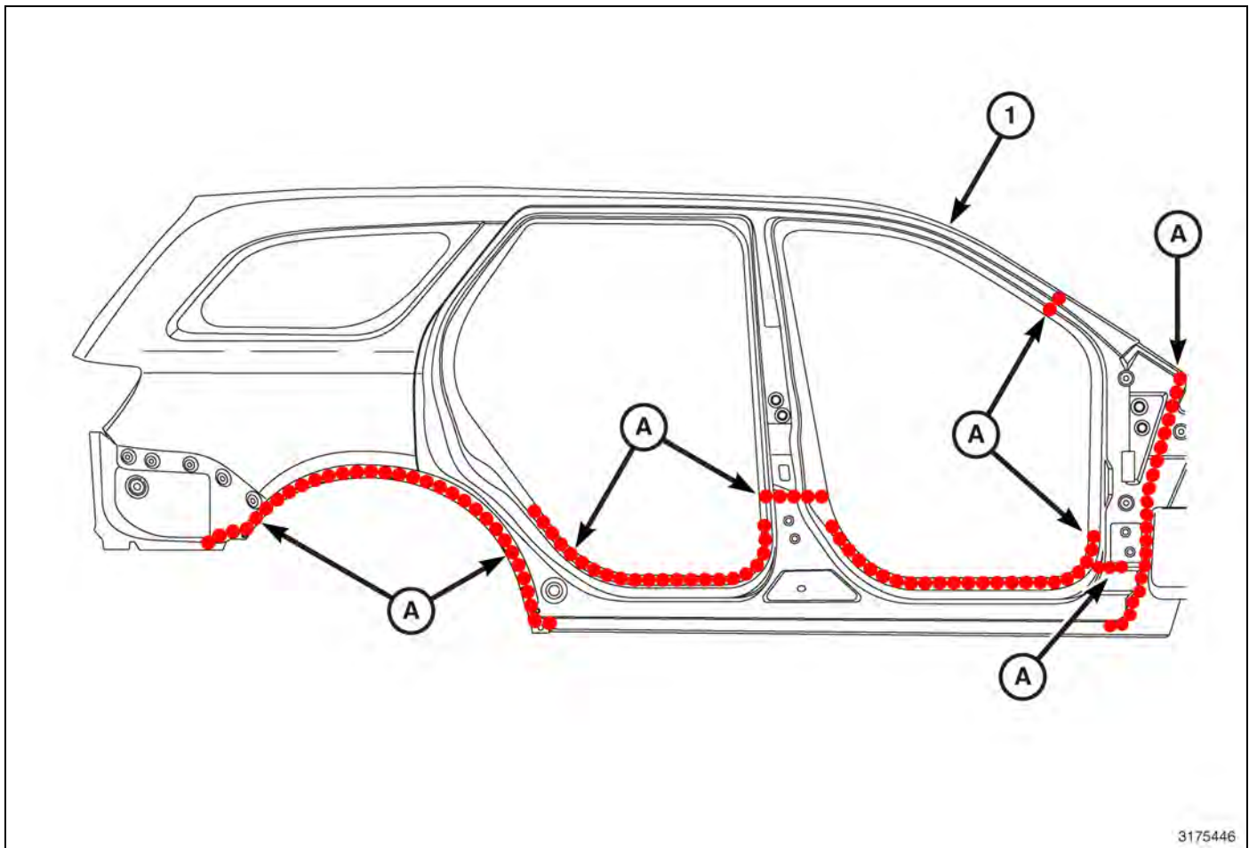
Fig. 53 Right Body Side Aperture
