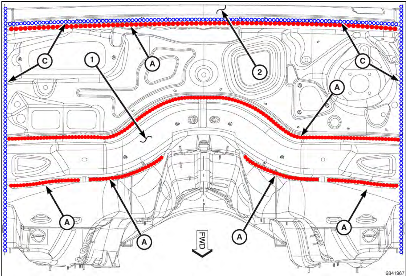
Fig. 64 Cowl / Dash Reinforcement
