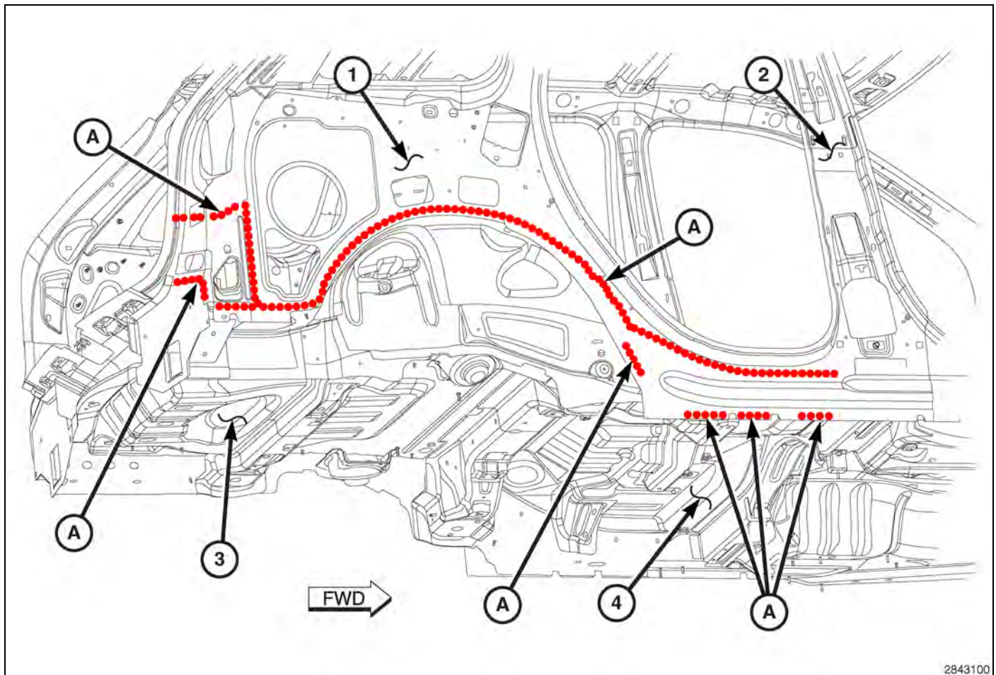
Fig. 90 Right Inner Body Side Panel / Inner Wheelhouse
