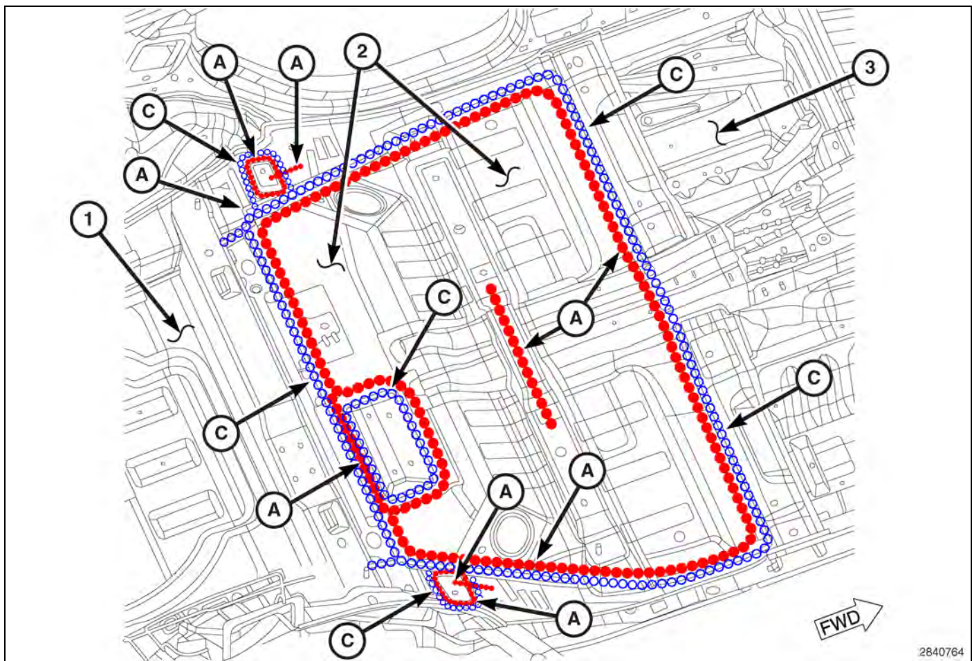
Fig. 77 Mid Floor (1 of 3)
