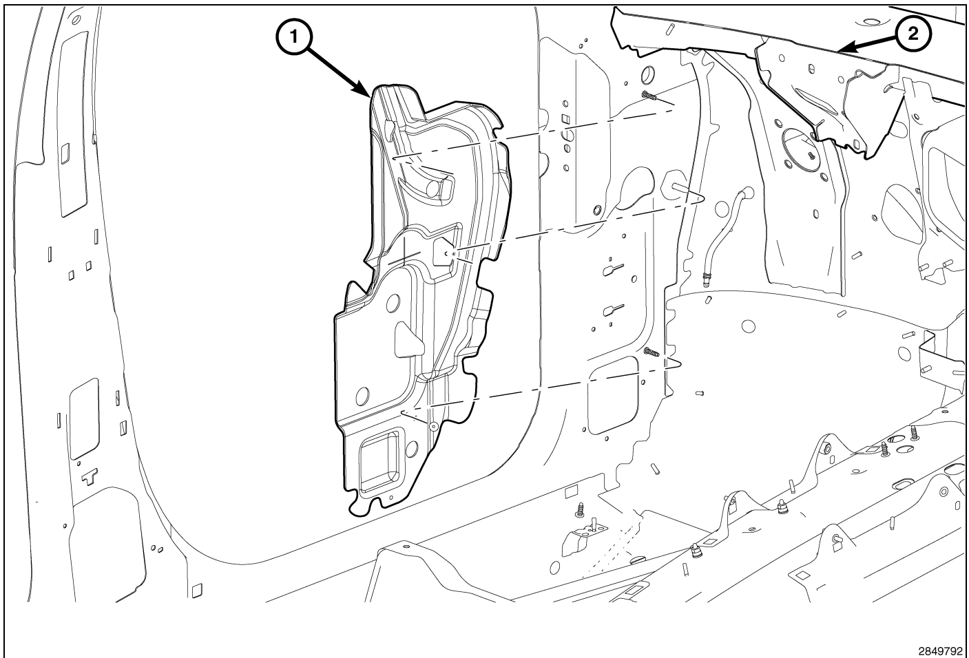
Fig. 35 Left Cowl
