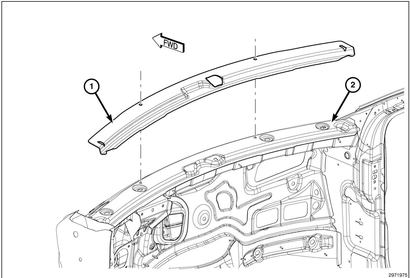
Fig. 32 Cowl Panel
