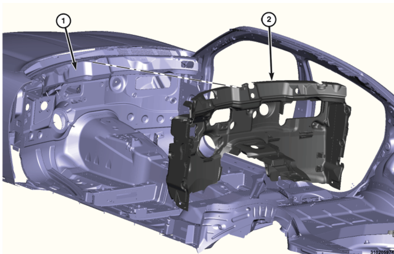
Dash Panel (Inner)
