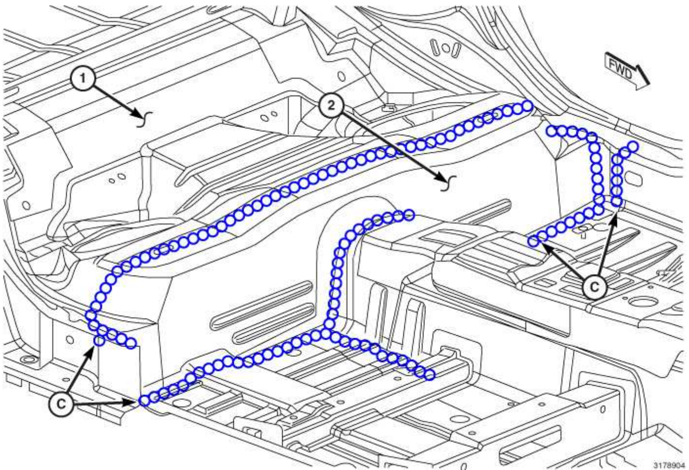
Rear Floor Crossmember
