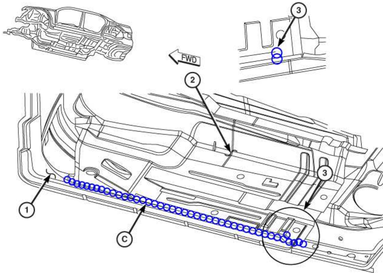
Front Floor
