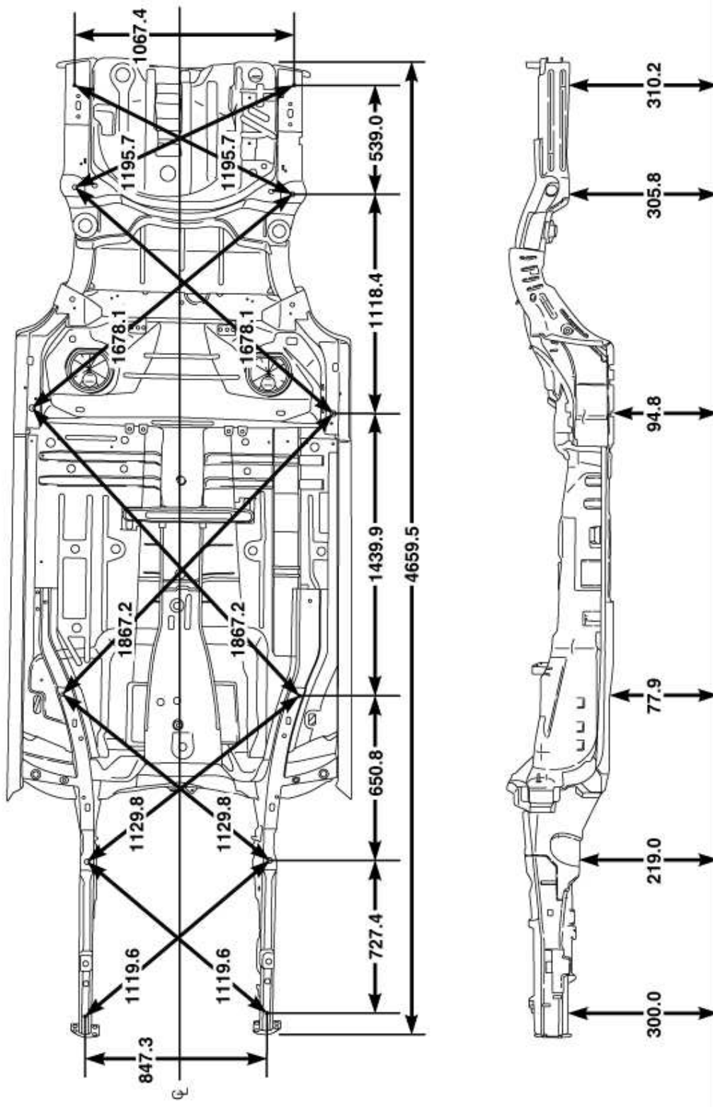
Underbody Dimensions
