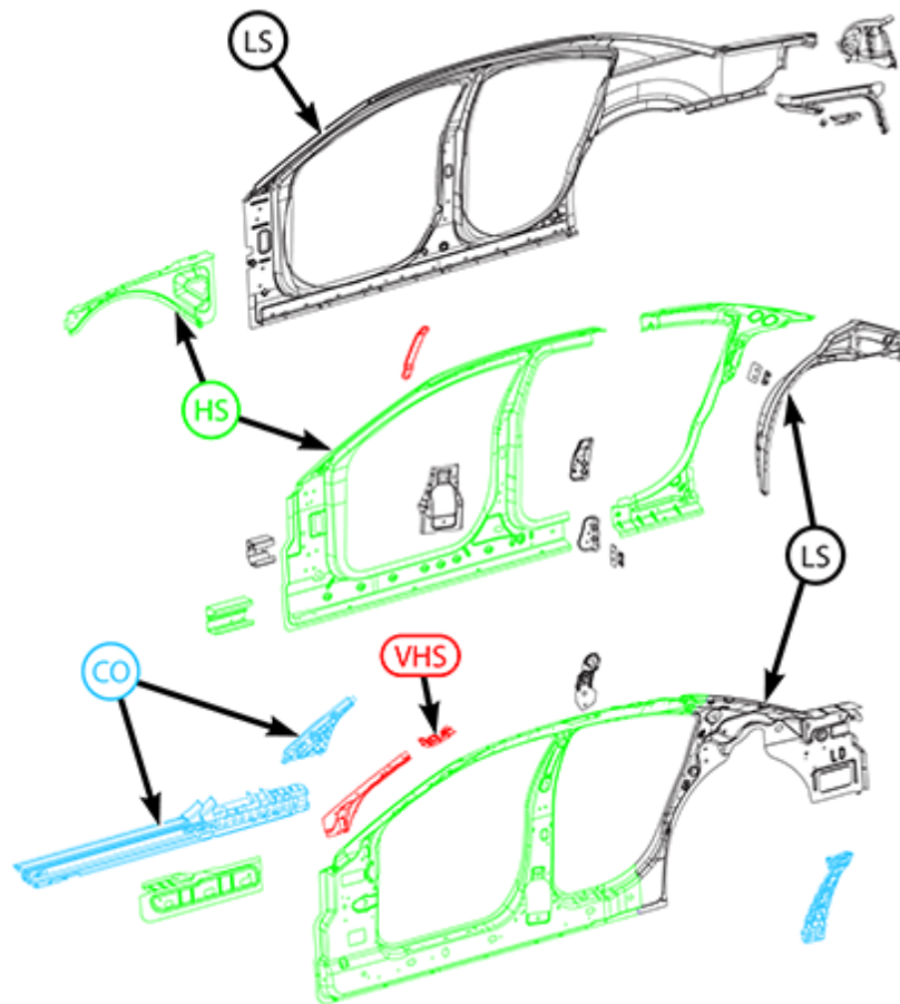
BODY IN WHITE COMPONENT IDENTIFICATION - BODY SIDE APERTURE
