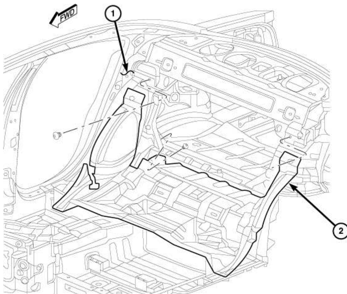
Floor Pan (1 of 2)
