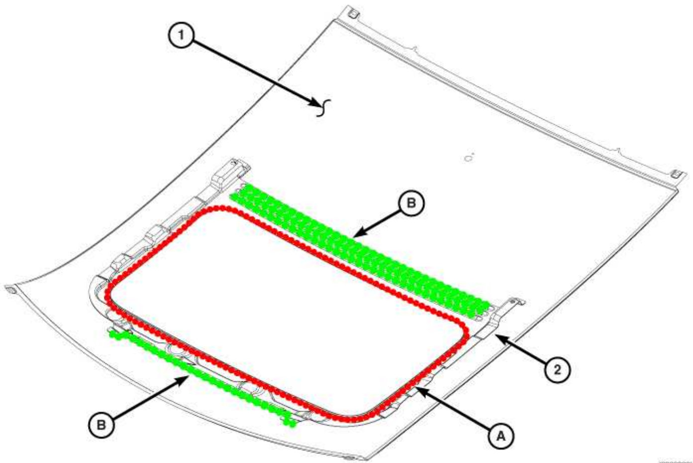
Sunroof Reinforcement (2 of 2)
