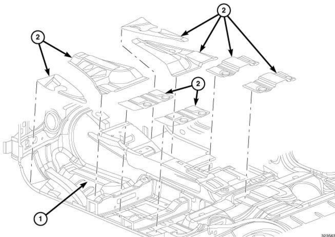
Front Floor Pan
