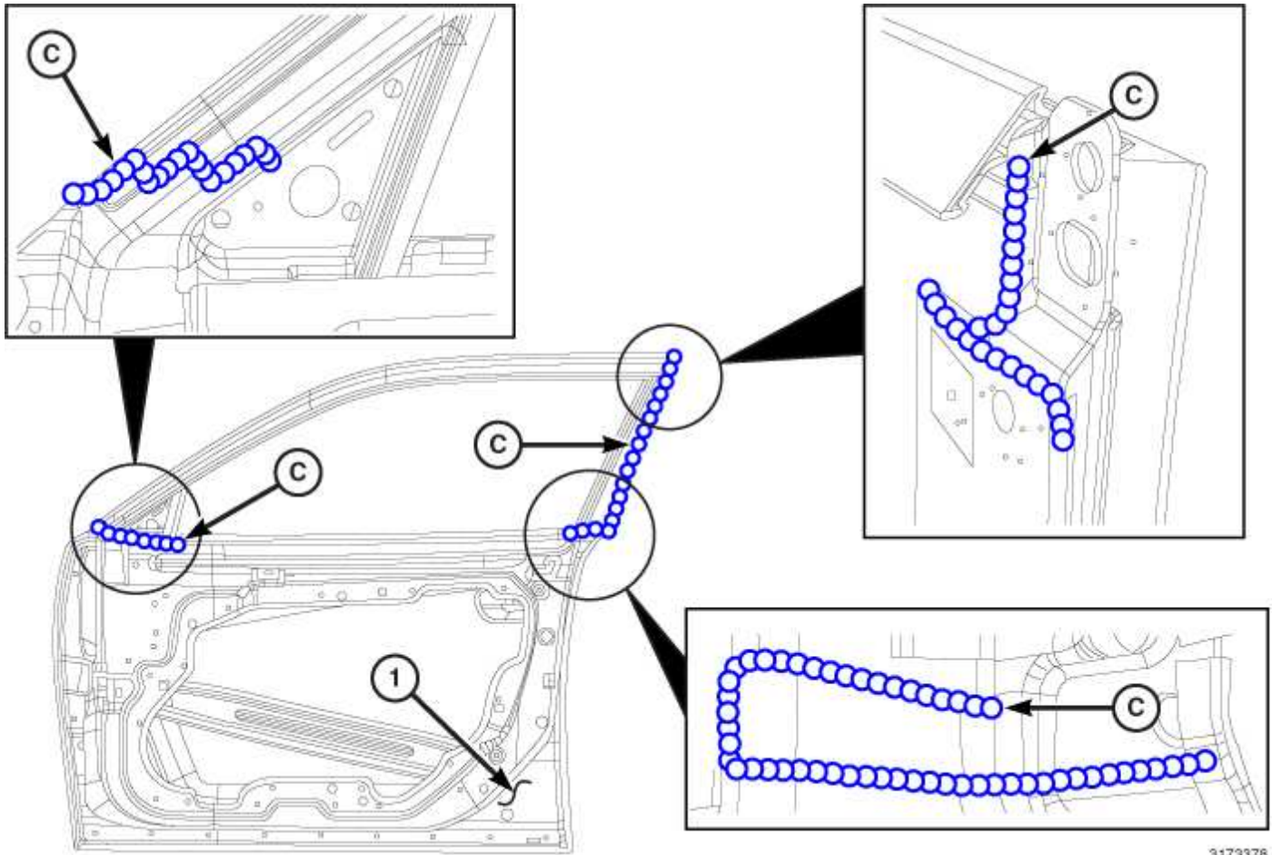
Front Door (2 of 2)
