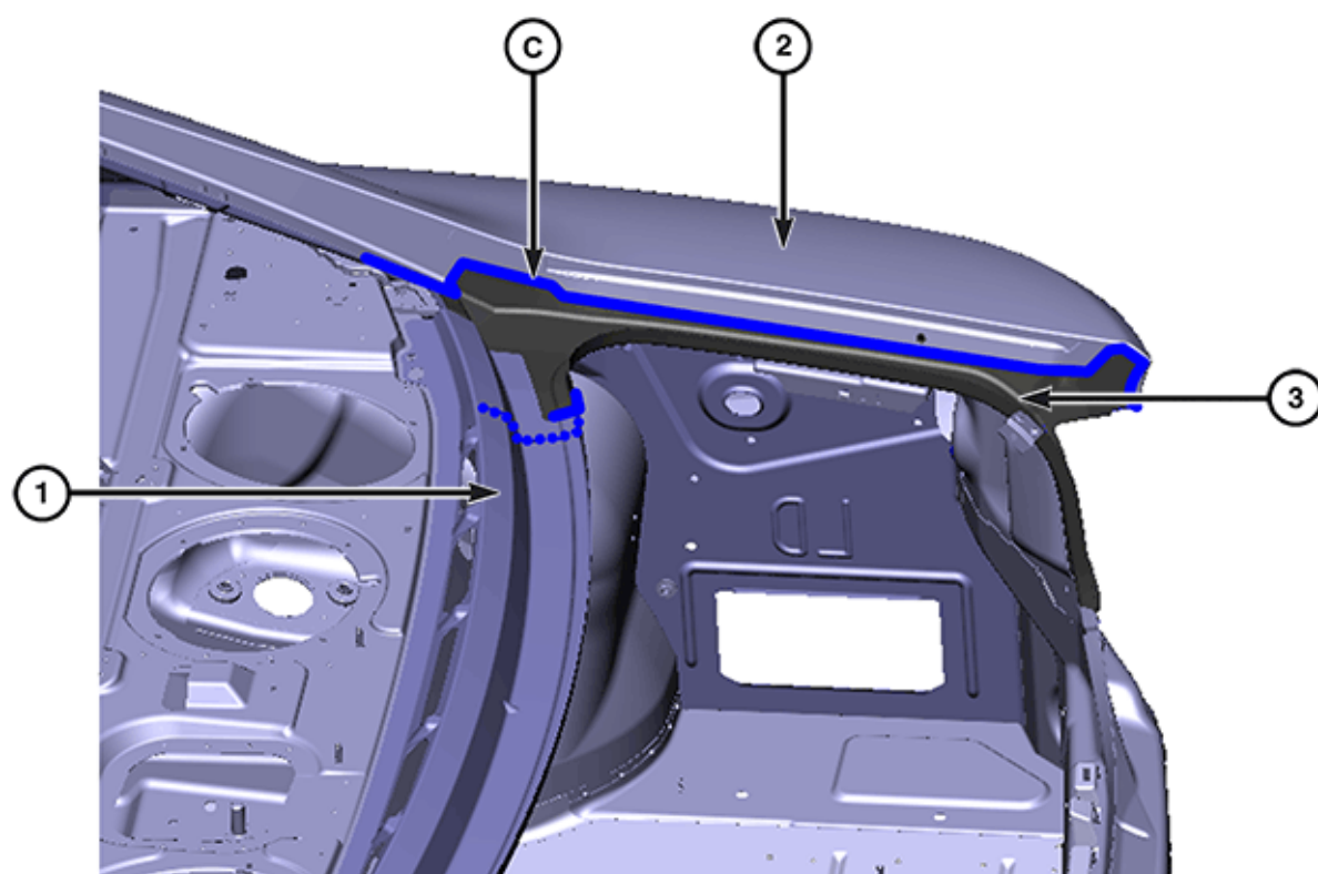
Drain Trough / Rear Shelf (1 of 2)
