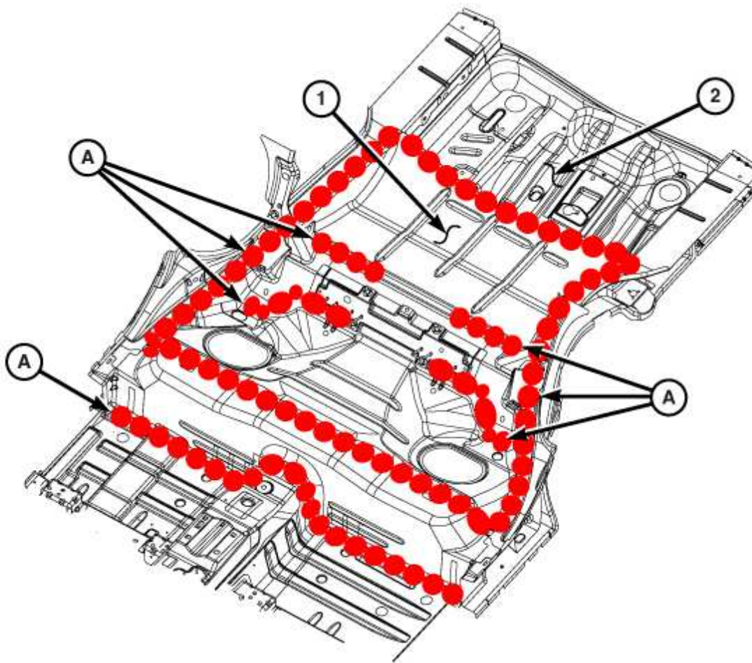
Rear Floor
