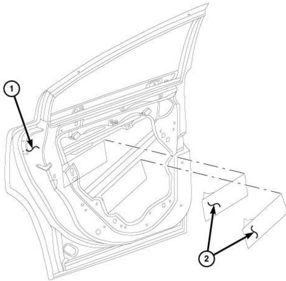
Rear Door
