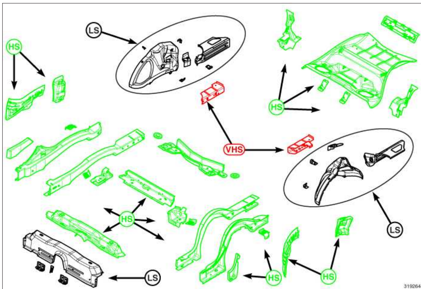
BODY IN WHITE COMPONENT IDENTIFICATION - REAR FLOOR
