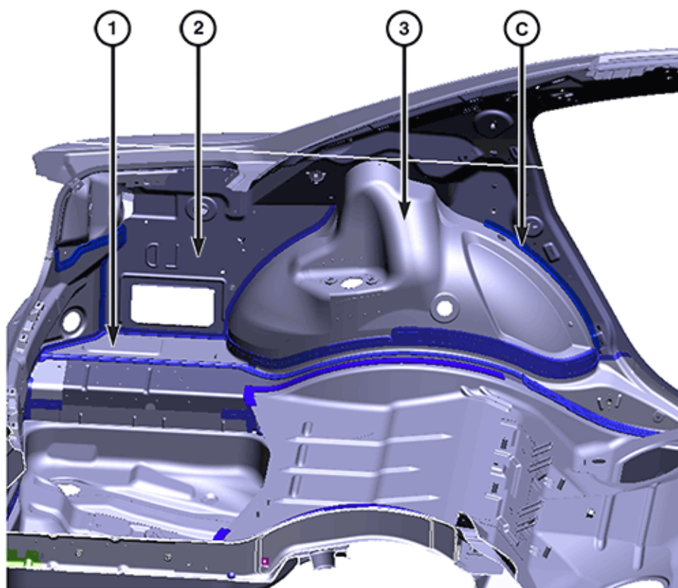
Rear Inner Wheelhouse (3 of 3)
