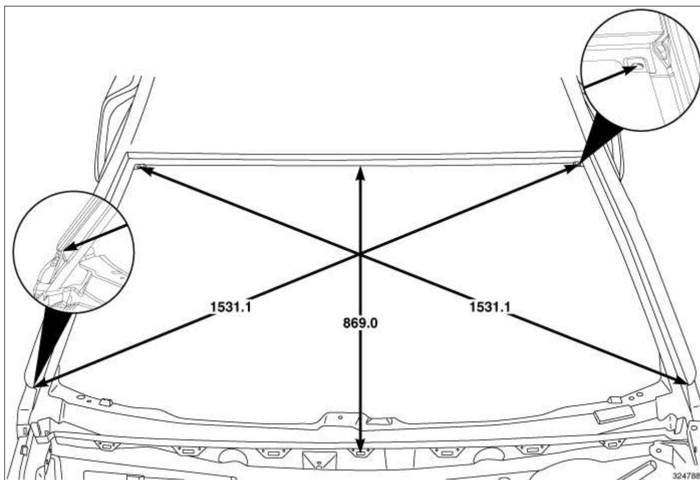
WINDSHIELD OPENING
