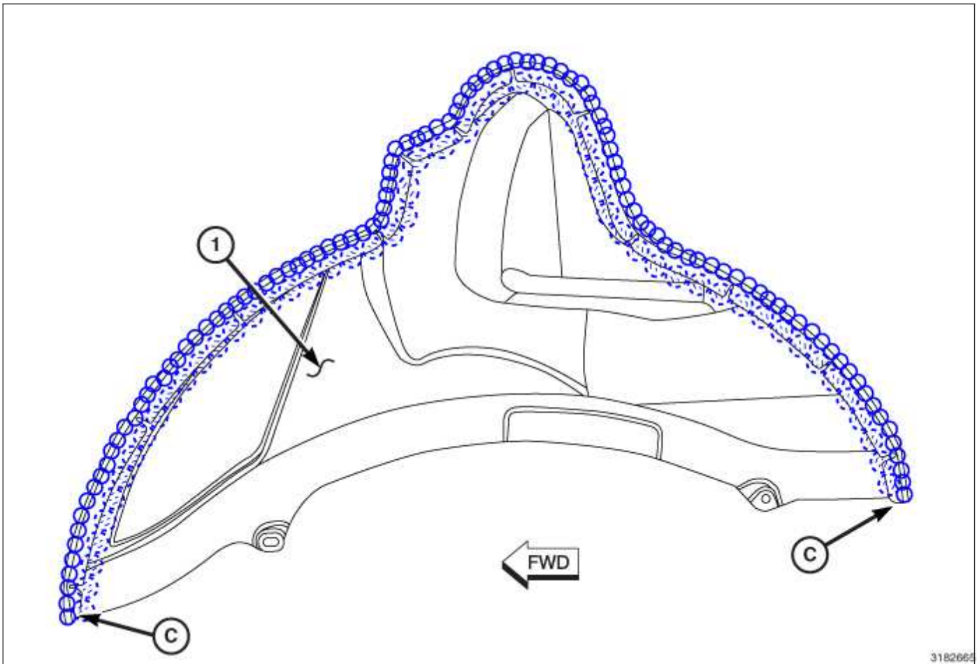
Left Wheelhouse
