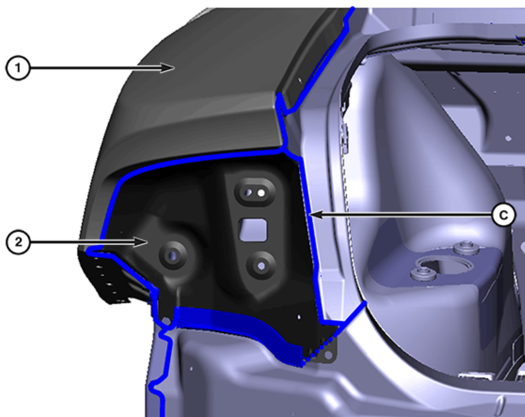
Taillamp Pocket (2 of 2)
