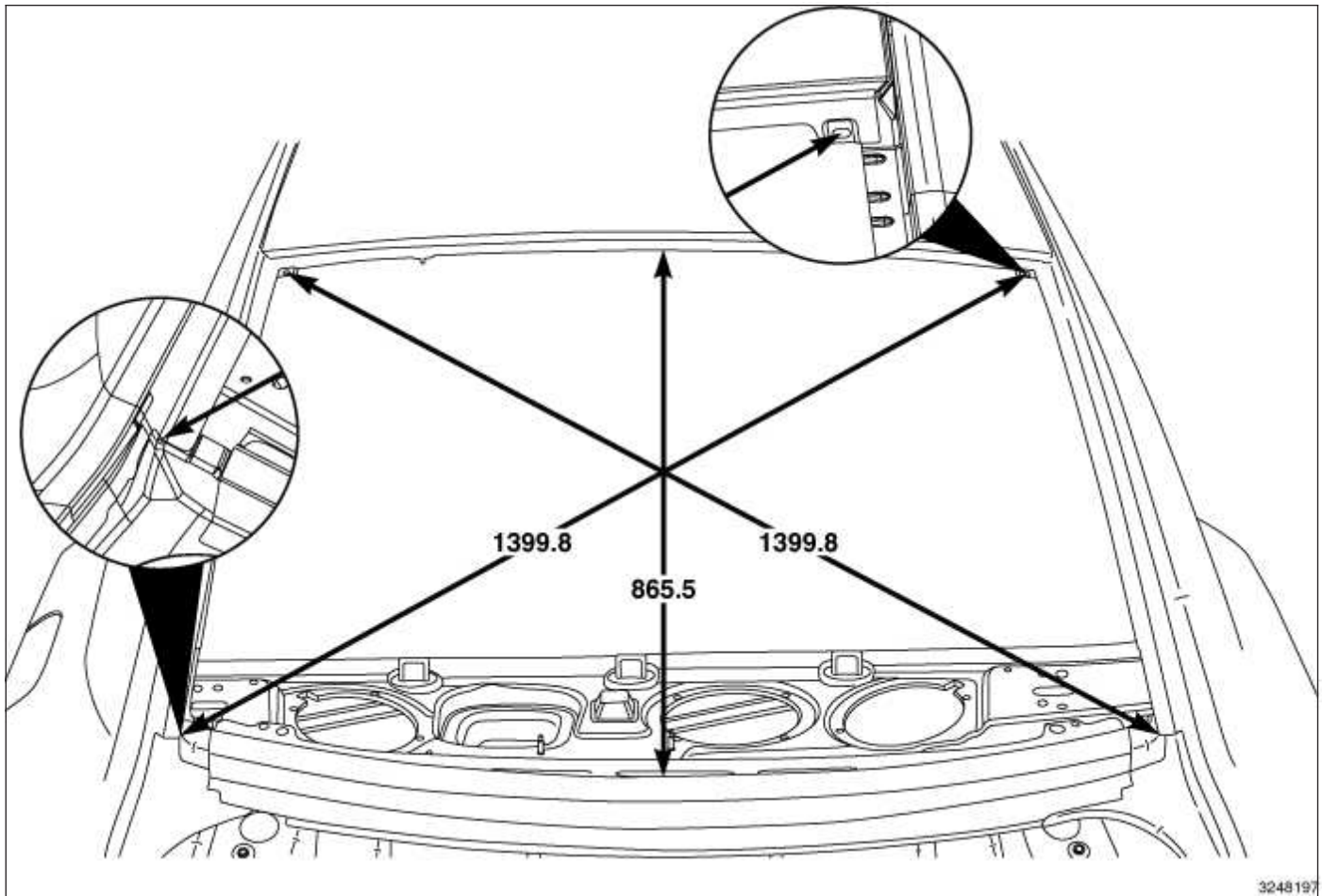
BACKLIGHT OPENING
