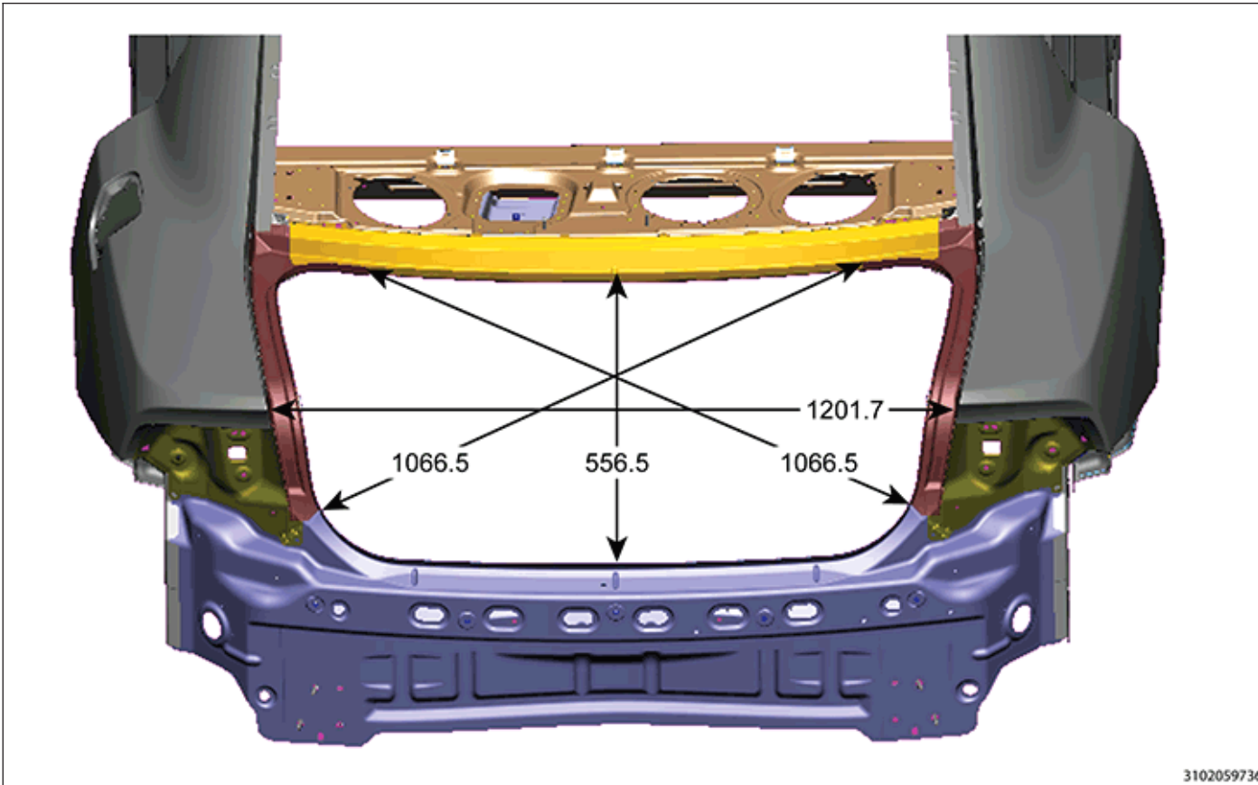
DECKLID OPENING
